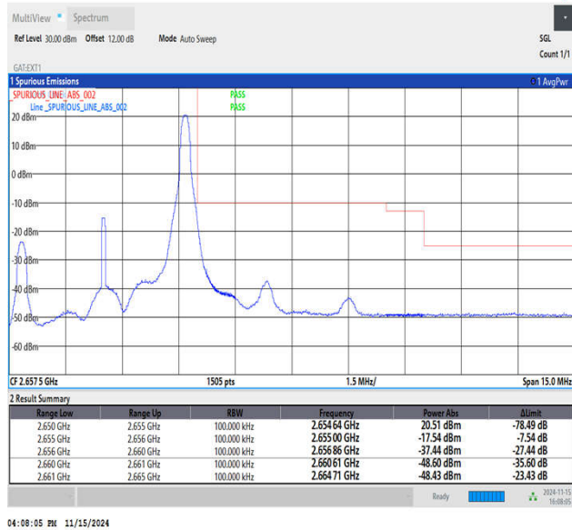
Band41_5MHz_64QAM_41215_1RB#24
