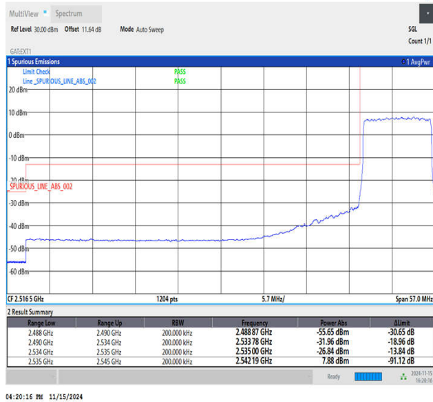
Band41_10MHz_QPSK_40090_50RB#0
