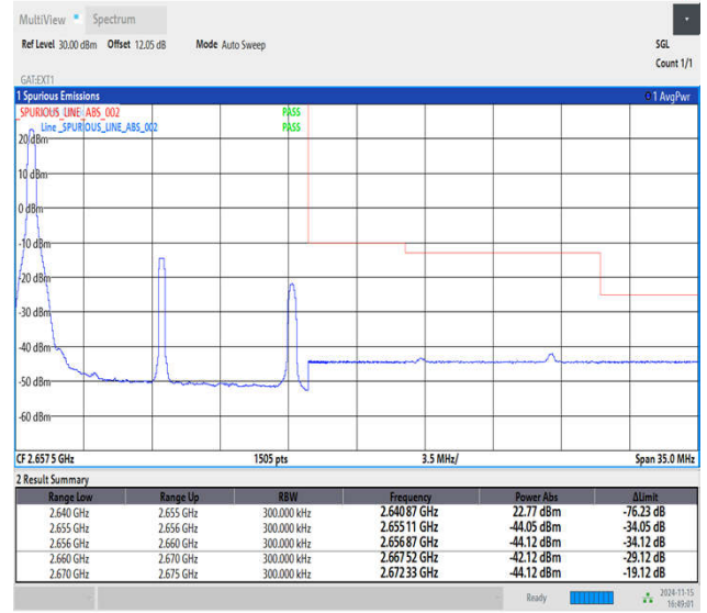
Band41_15MHz_64QAM_41165_1RB#0
