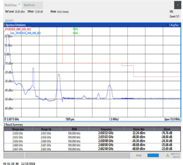
Band41_5MHz_QPSK_41215_1RB#0
