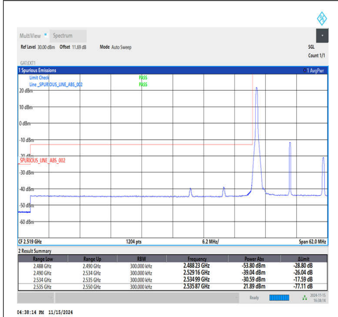
Band41_15MHz_64QAM_40115_1RB#0
