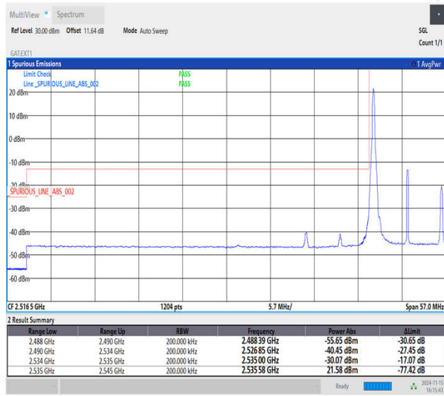
Band41_10MHz_64QAM_40090_1RB#0
