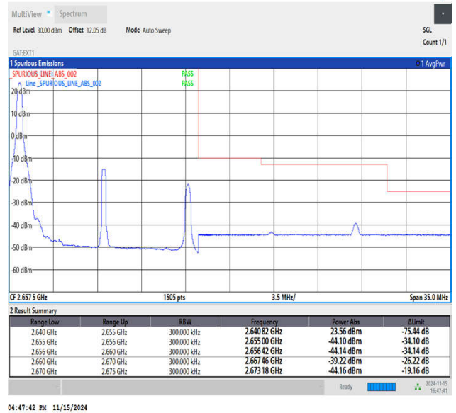
Band41_15MHz_16QAM_41165_1RB#0
