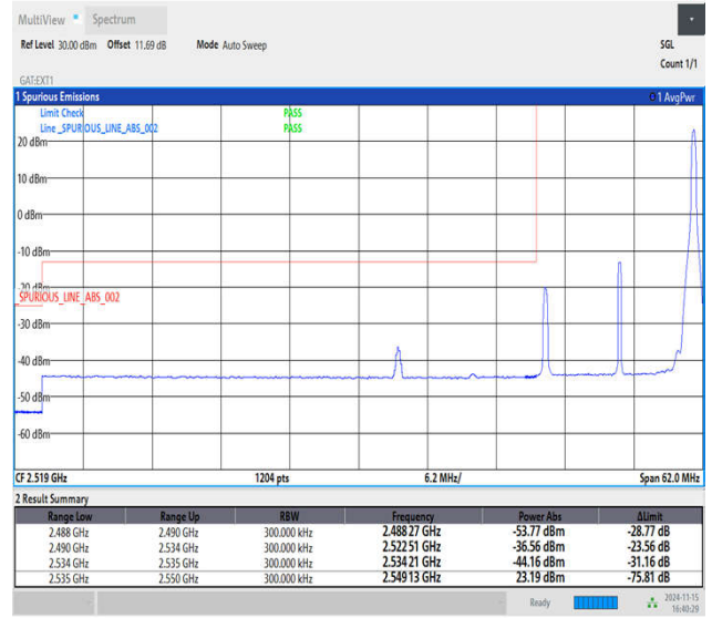
Band41_15MHz_16QAM_40115_1RB#74
