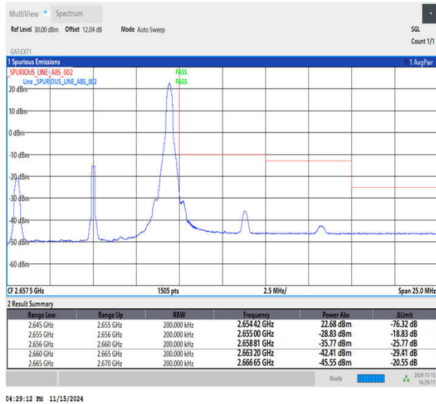
Band41_10MHz_16QAM_41190_1RB#49
