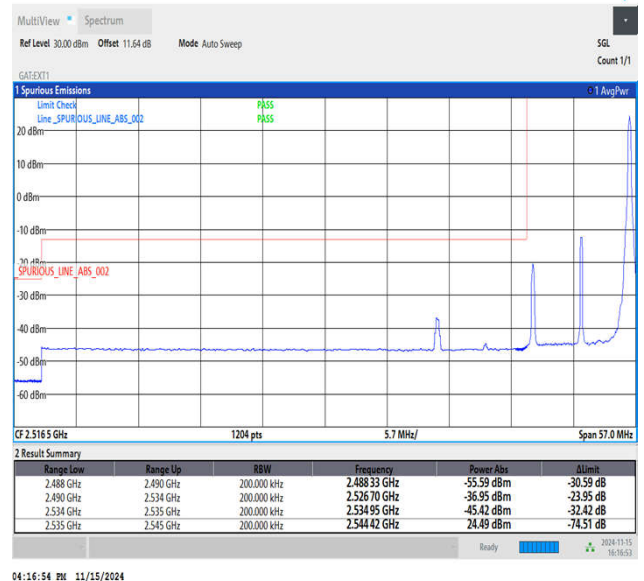
Band41_10MHz_QPSK_40090_1RB#49
