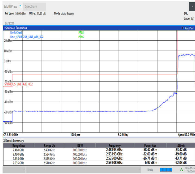
Band41_5MHz_64QAM_40065_25RB#0
