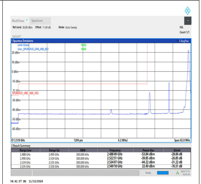
Band41_15MHz_64QAM_40115_1RB#74
