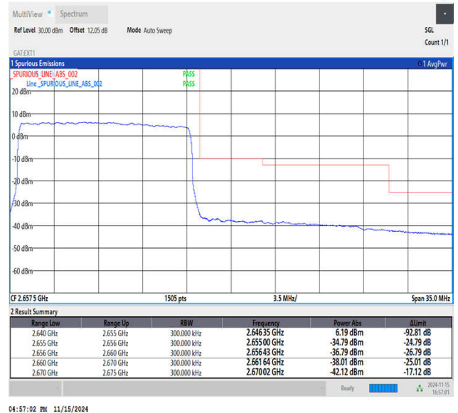
Band41_15MHz_64QAM_41165_75RB#0
