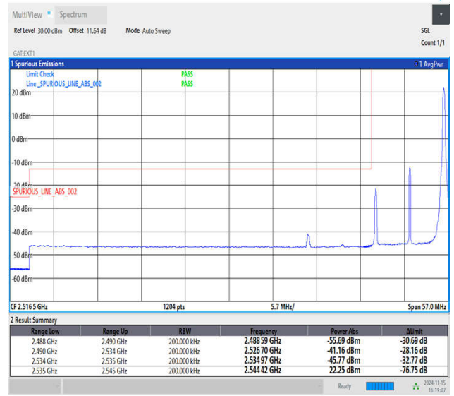
Band41_10MHz_64QAM_40090_1RB#49
