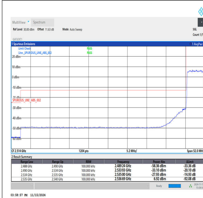
Band41_5MHz_16QAM_40065_25RB#0
