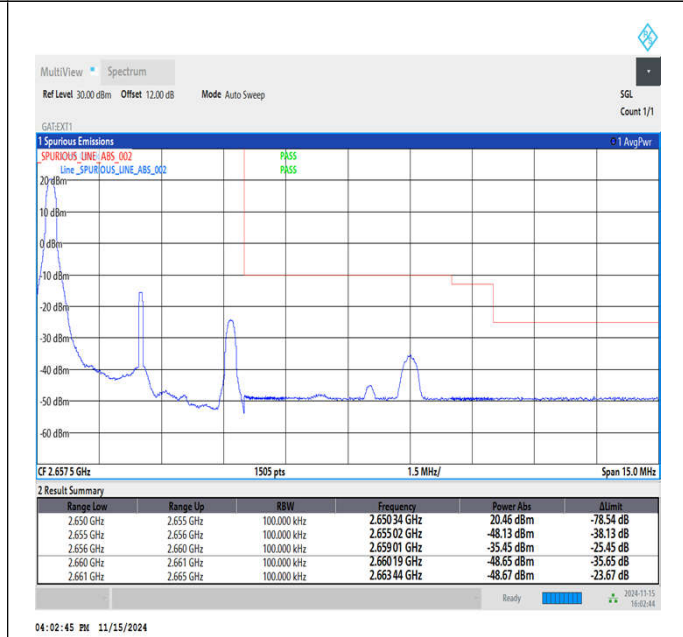
Band41_5MHz_16QAM_41215_1RB#0
