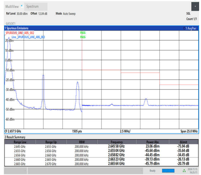
Band41_10MHz_16QAM_41190_1RB#0
