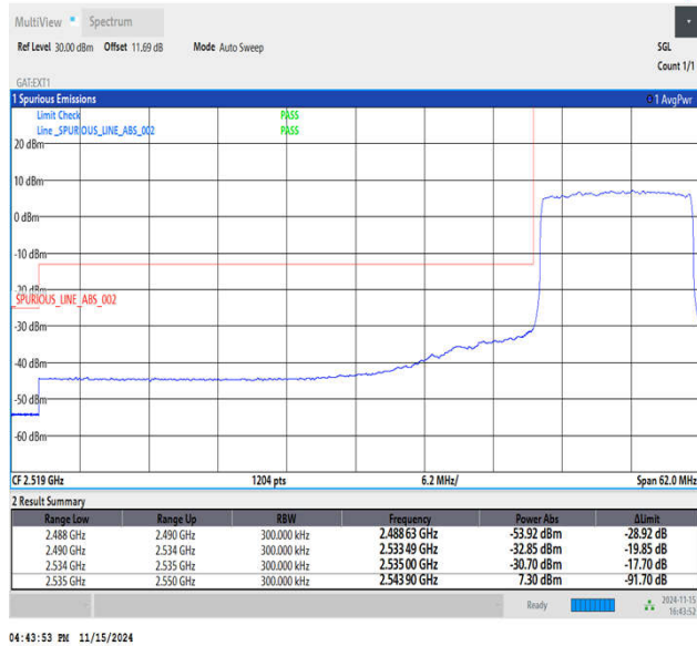
Band41_15MHz_16QAM_40115_75RB#0
