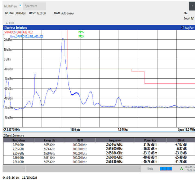
Band41_5MHz_QPSK_41215_1RB#24
