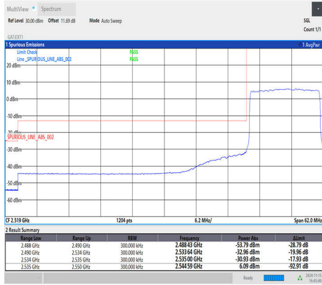
Band41_15MHz_64QAM_40115_75RB#0
