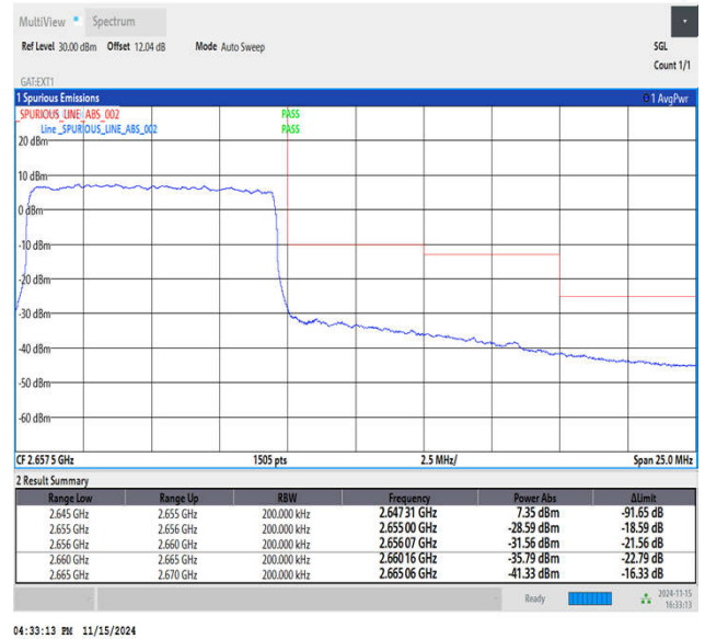
Band41_10MHz_16QAM_41190_50RB#0
