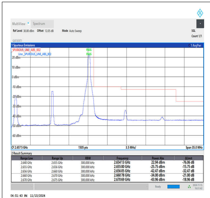
Band41_15MHz_16QAM_41165_1RB#74
