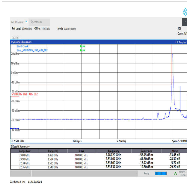
Band41_5MHz_16QAM_40065_1RB#0
