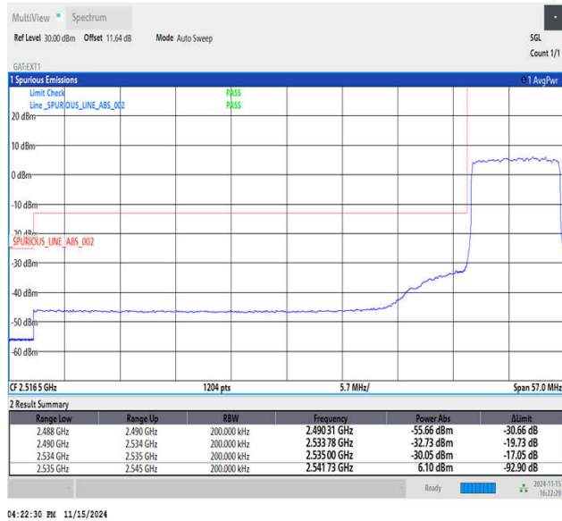
Band41_10MHz_64QAM_40090_50RB#0
