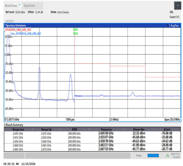
Band41_10MHz_64QAM_41190_1RB#0
