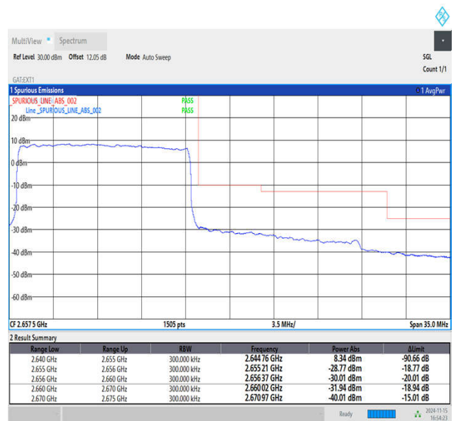
Band41_15MHz_QPSK_41165_1RB#0
