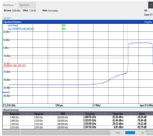
Band41_10MHz_16QAM_40090_50RB#0
