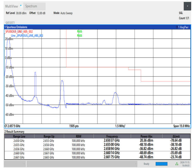
Band41_5MHz_64QAM_41215_1RB#0
