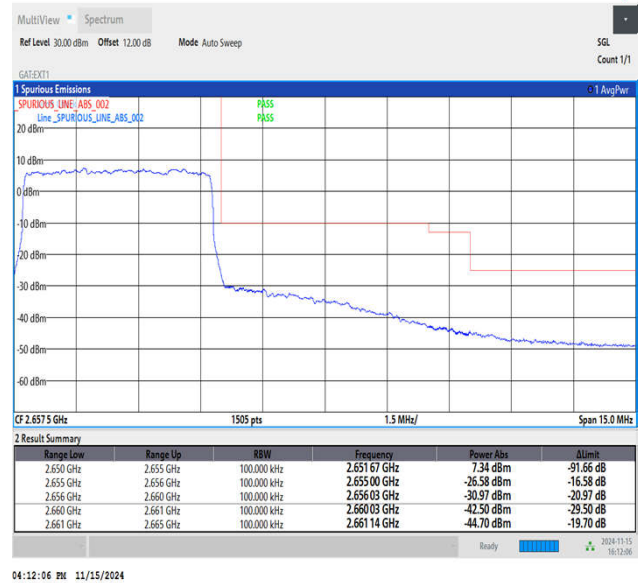
Band41_5MHz_64QAM_41215_25RB#0
