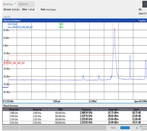
Band41_15MHz_16QAM_40115_1RB#0
