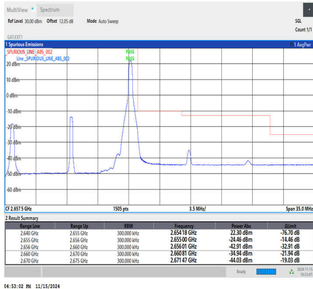
Band41_15MHz_64QAM_41165_1RB#74
