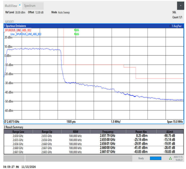
Band41_5MHz_QPSK_41215_25RB#0
