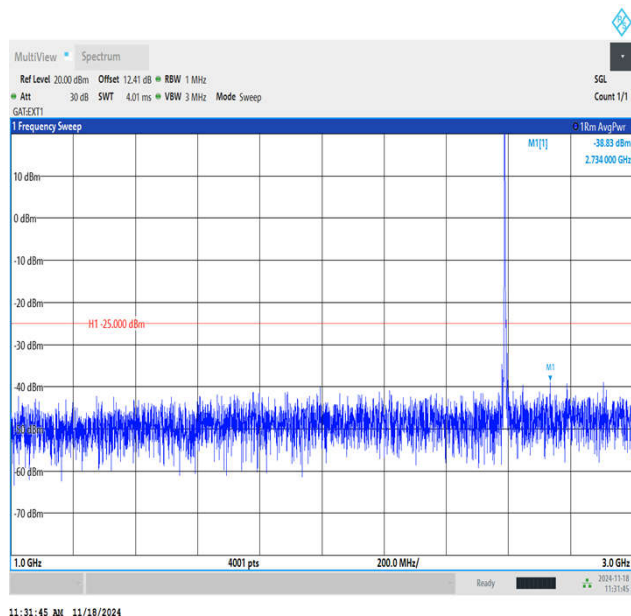
Band41_5MHz_QPSK_40590_1RB#0_1000~3000_1000~3000
