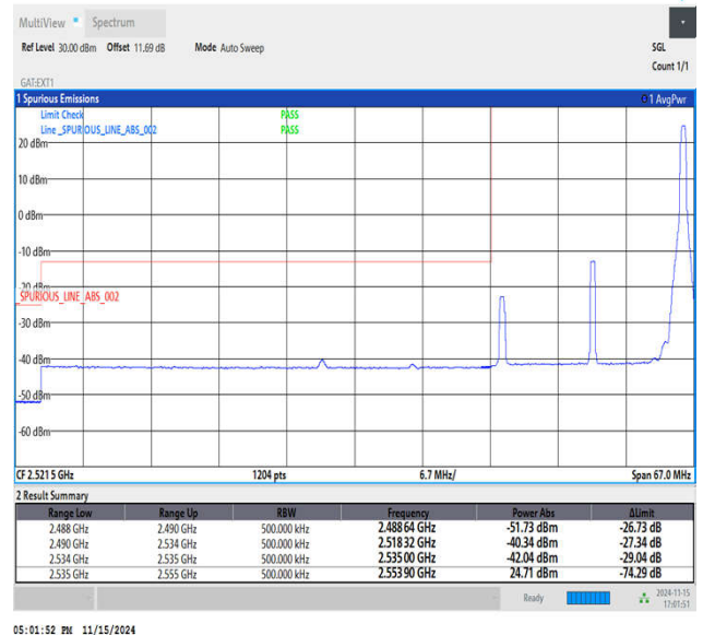
Band41_20MHz_QPSK_40140_1RB#99
