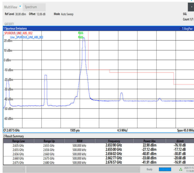
Band41_20MHz_16QAM_41140_1RB#99
