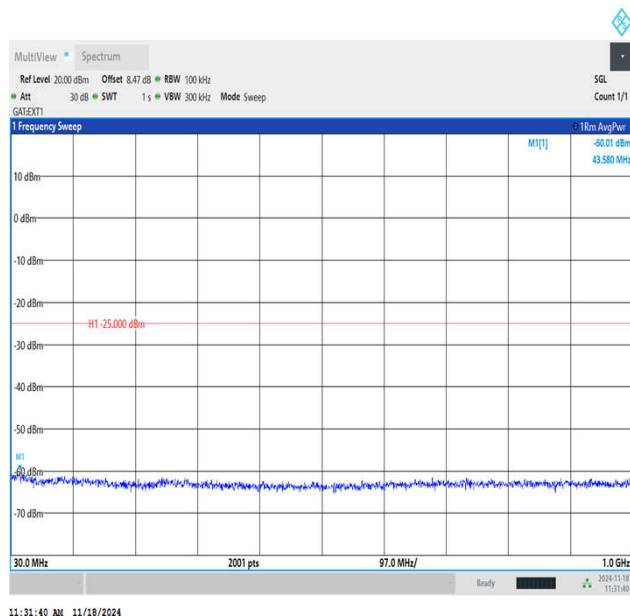
Band41_5MHz_QPSK_40590_1RB#0_30~1000_30~1000
