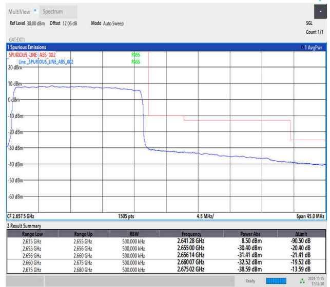
Band41_20MHz_16QAM_41140_100RB#0
