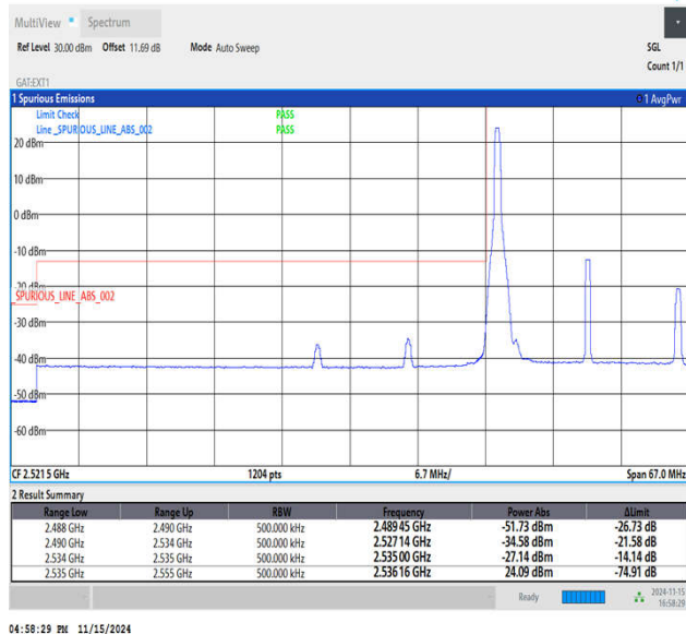
Band41_20MHz_QPSK_40140_1RB#0
