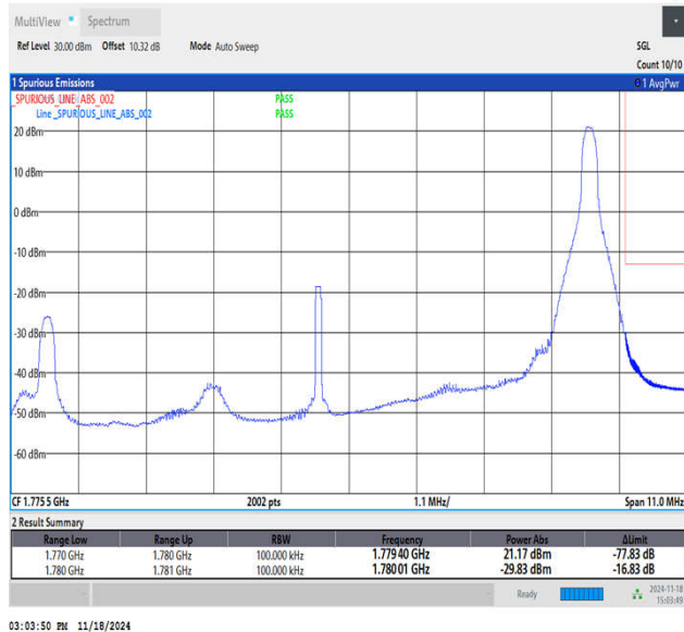
Band66_10MHz_16QAM_132622_1RB#49
