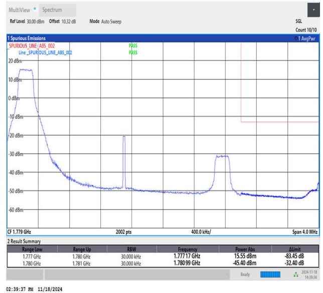
Band66_3MHz_64QAM_132657_1RB#0
