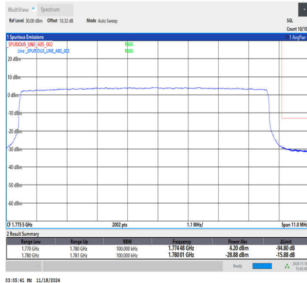
Band66_10MHz_16QAM_132622_50RB#0
