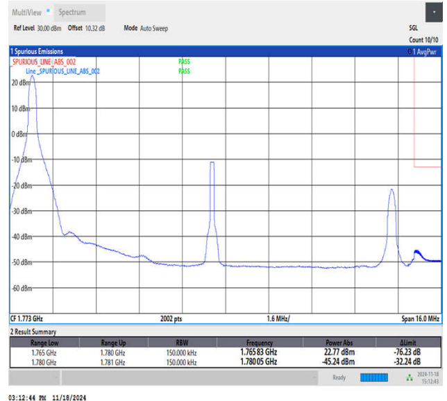
Band66_15MHz_QPSK_132597_1RB#0
