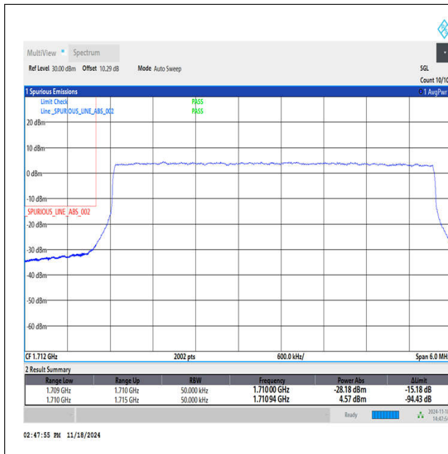
Band66_5MHz_QPSK_131997_25RB#0
