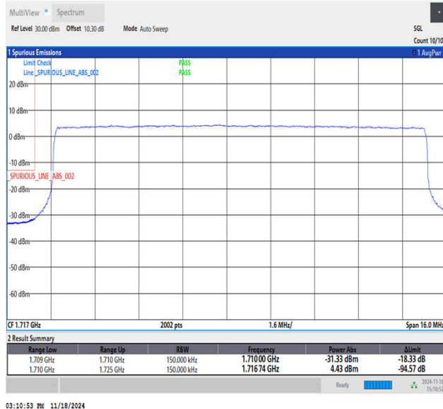
Band66_15MHz_QPSK_132047_75RB#0
