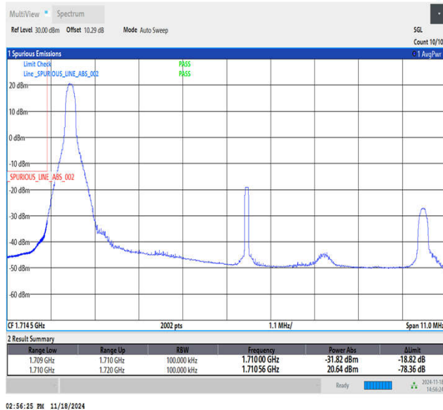
Band66_10MHz_16QAM_132022_1RB#0
