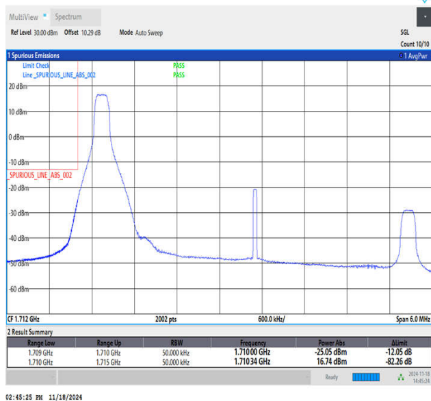
Band66_5MHz_64QAM_131997_1RB#0
