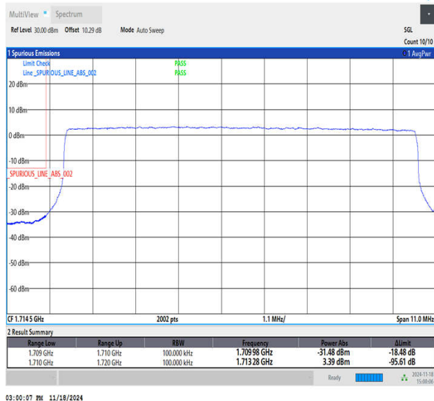
Band66_10MHz_16QAM_132022_50RB#0
