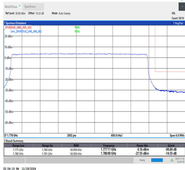
Band66_5MHz_16QAM_132647_25RB#0
