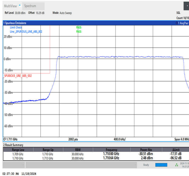
Band66_3MHz_64QAM_131987_15RB#0
