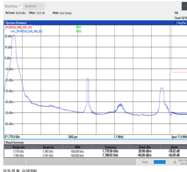
Band66_10MHz_16QAM_132622_1RB#0
