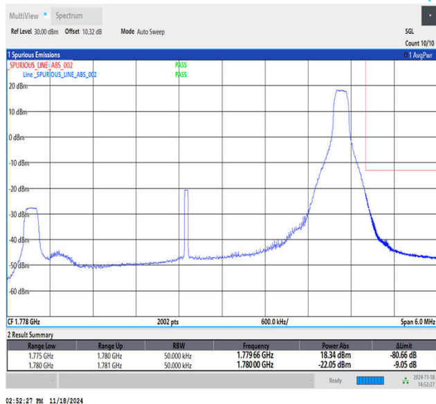
Band66_5MHz_16QAM_132647_1RB#24
