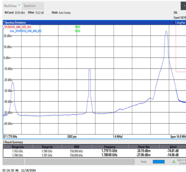
Band66_15MHz_QPSK_132597_1RB#74
