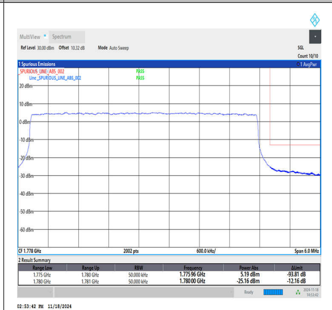
Band66_5MHz_QPSK_132647_1RB#0
