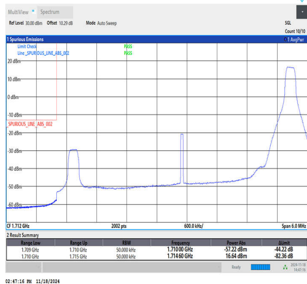
Band66_5MHz_64QAM_131997_1RB#24
