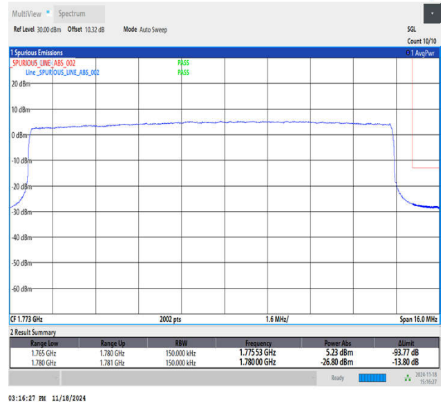
Band66_15MHz_QPSK_132597_75RB#0
