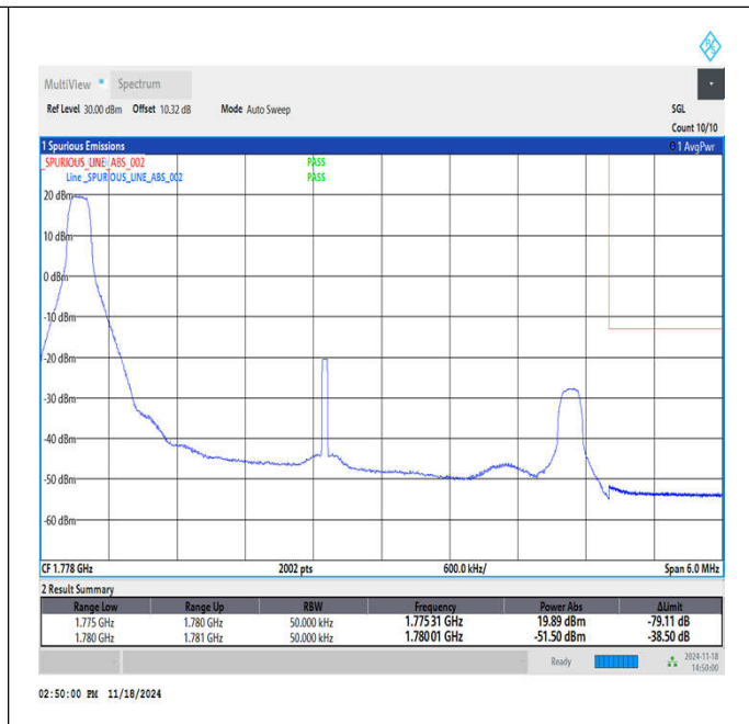
Band66_5MHz_QPSK_132647_1RB#0
