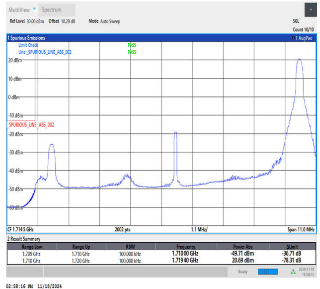
Band66_10MHz_16QAM_132022_1RB#49
