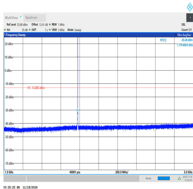
Band66_1.4MHz_QPSK_132665_1RB#0_1000~3000_1000 ~3000
