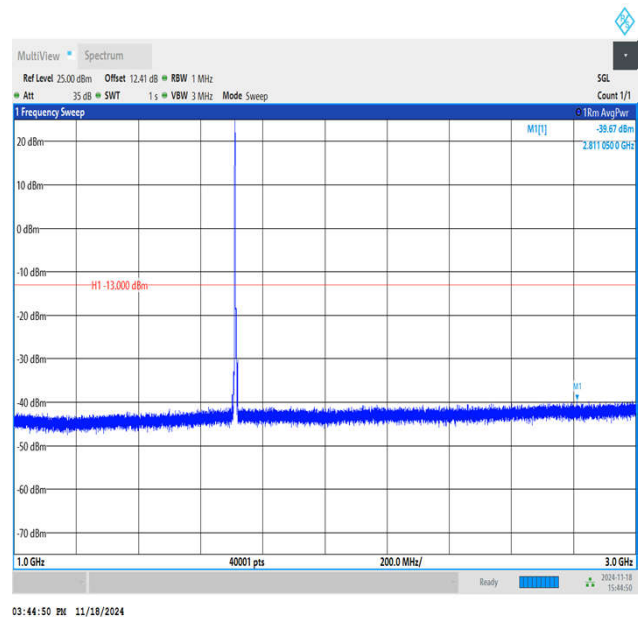
Band66_5MHz_QPSK_131997_1RB#0_1000~3000_1000~3000
