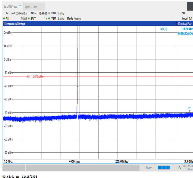
Band66_3MHz_QPSK_132657_1RB#0_1000~3000_1000~3000
