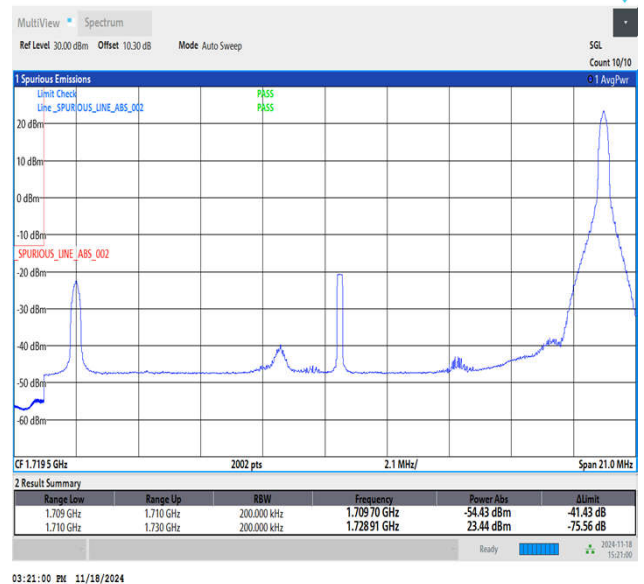
Band66_20MHz_16QAM_132072_1RB#99
