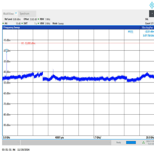
Band66_20MHz_QPSK_132322_1RB#0_3000~20000_3000~20000
