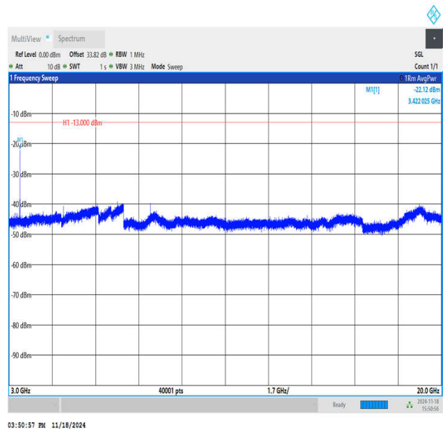
Band66_20MHz_QPSK_132072_1RB#0_3000~20000_3000 ~20000
