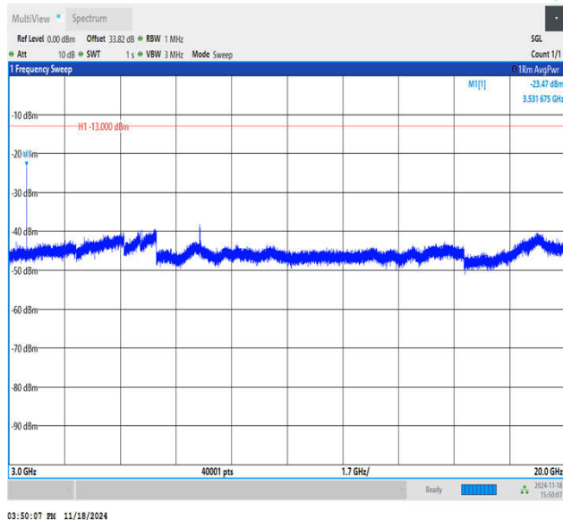
Band66_15MHz_QPSK_132597_1RB#0_3000~20000_3000 ~20000
