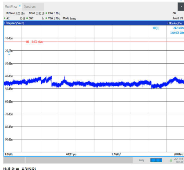
Band66_1.4MHz_QPSK_132322_1RB#0_3000~20000_300 0~20000
