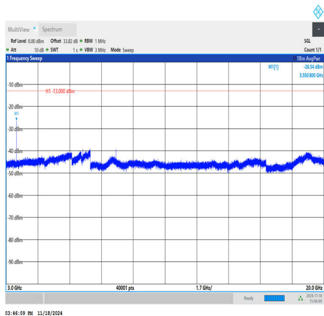
Band66_5MHz_QPSK_132647_1RB#0_3000~20000_3000~20000
