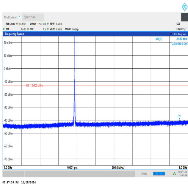
Band66_10MHz_QPSK_132622_1RB#0_1000~3000_1000~3000
