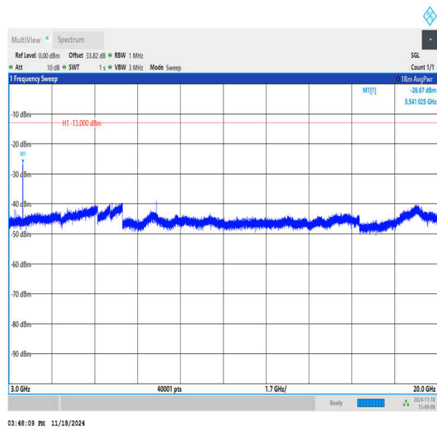
Band66_10MHz_QPSK_132622_1RB#0_3000~20000_3000~20000
