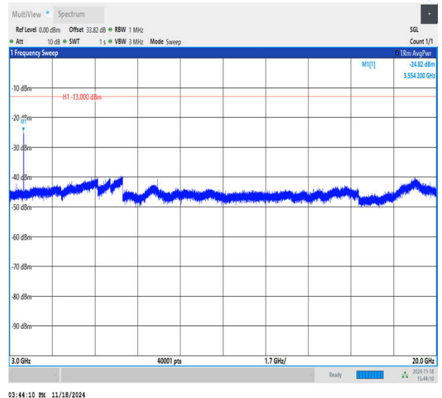
Band66_3MHz_QPSK_132657_1RB#0_3000~20000_3000~20000
