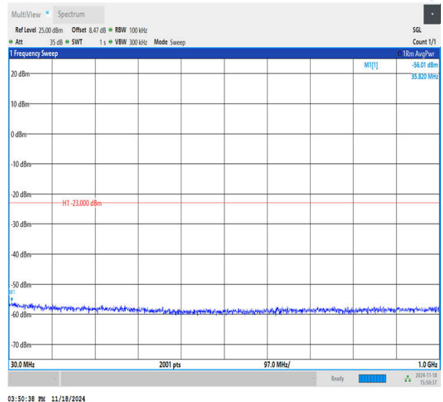
Band66_20MHz_QPSK_132072_1RB#0_30~1000_30~1000
