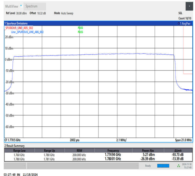
Band66_20MHz_QPSK_132572_100RB#0
