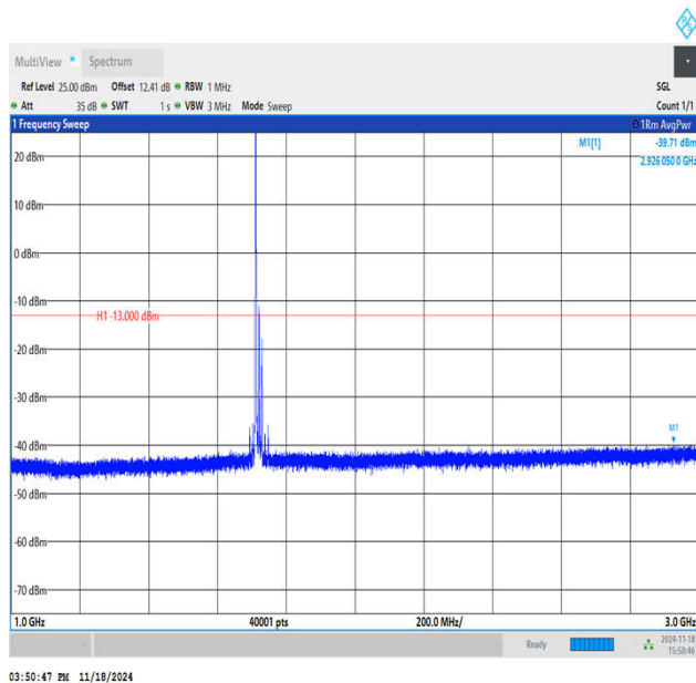
Band66_20MHz_QPSK_132072_1RB#0_1000~3000_1000~ 3000
