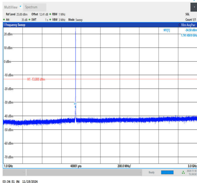
Band66_1.4MHz_QPSK_132322_1RB#0_1000~3000_1000 ~3000
