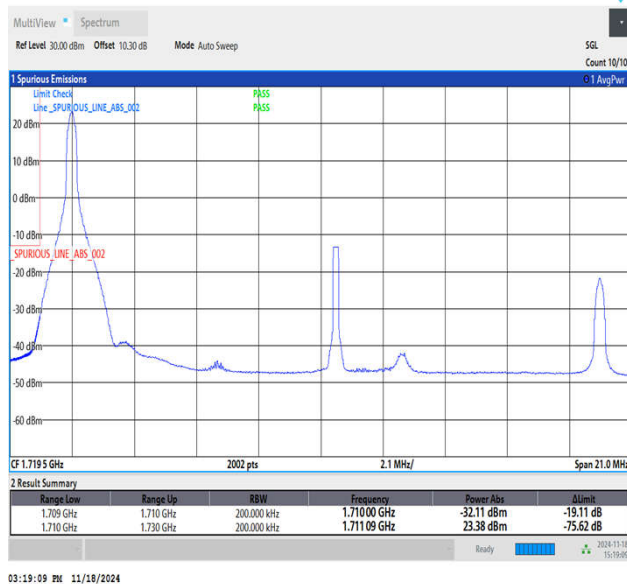
Band66_20MHz_16QAM_132072_1RB#0
