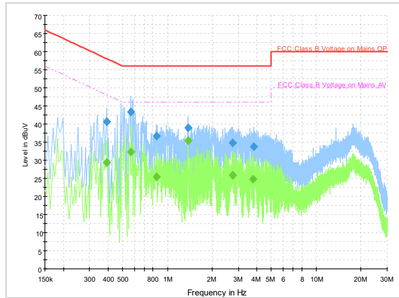
Fig.A.6.1. AC Powerline Conducted Emission-802.11a CH149 Tx
