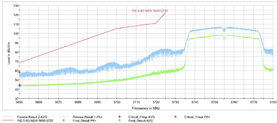
Fig. 5 Band Edges (802.11n-HT40 Ch151, 5755MHz)
