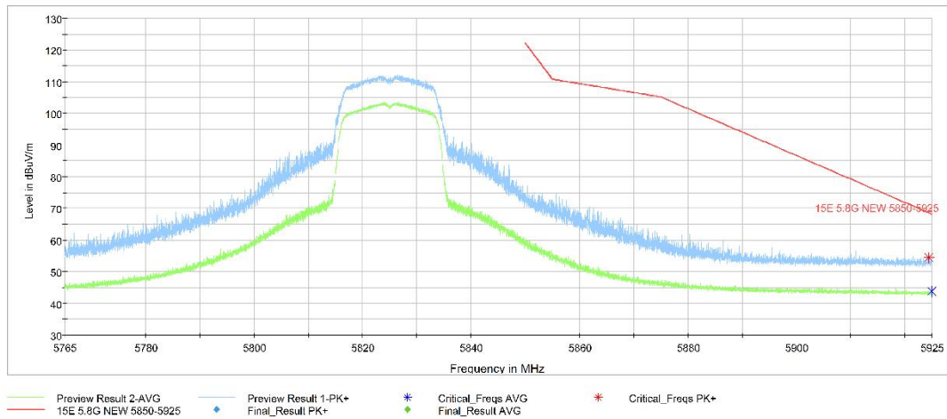
Fig. 8 Band Edges (802.11ac-HT20 Ch165, 5825MHz)
