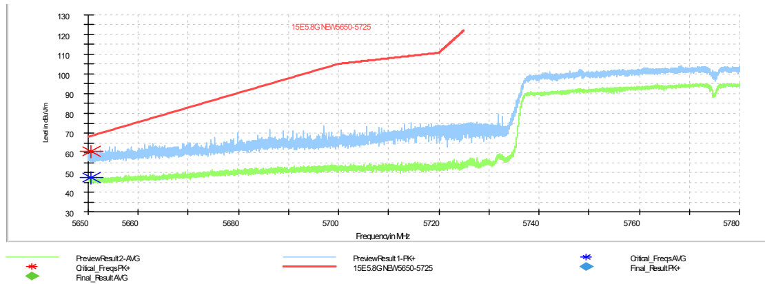
Fig. 11 Band Edges (802.11ac-HT80 Ch155, 5775MHz)
