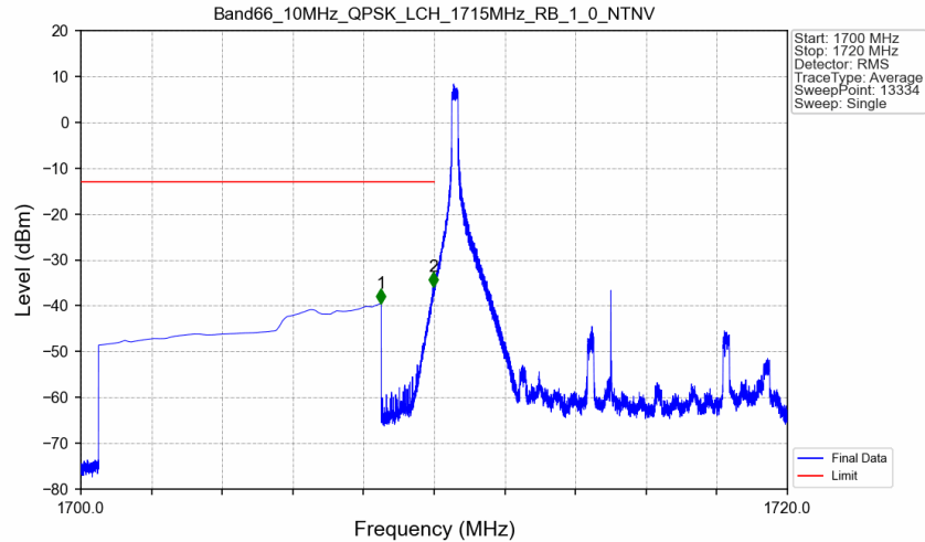
Band66_10MHz_QPSK_LCH_1715MHz_RB_1_0_NTNV
