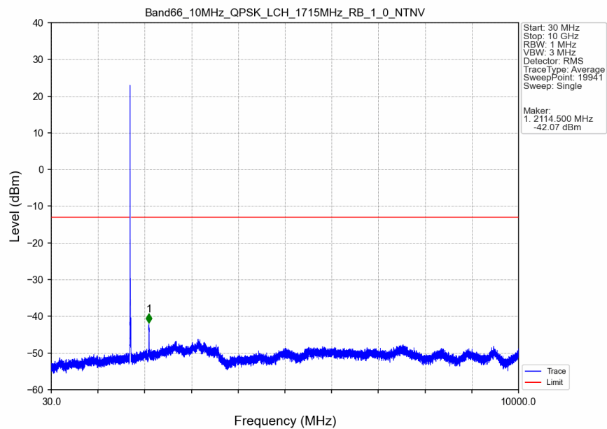
Band66_10MHz_QPSK_LCH_1715MHz_RB_1_0_NTNV
