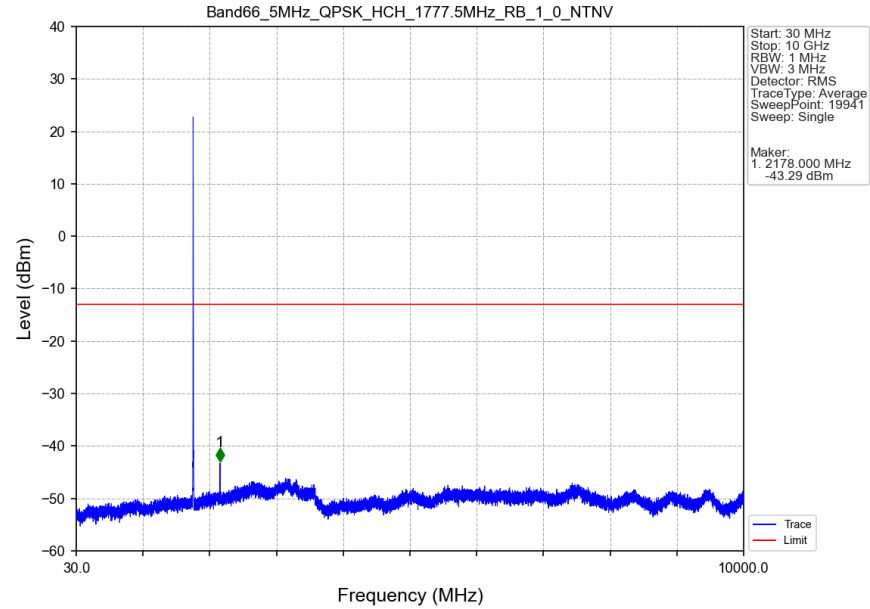
Band66_5MHz_QPSK_HCH_1777.5MHz_RB_1_0_NTNV
