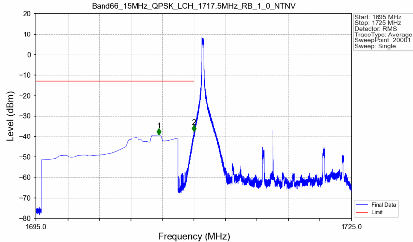
Band66_15MHz_QPSK_LCH_1717.5MHz_RB_1_0_NTNV
