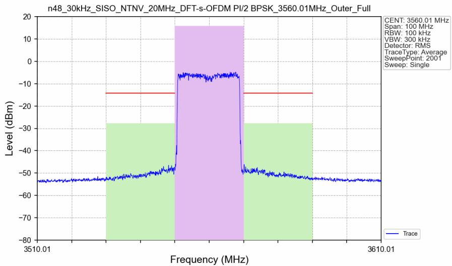
n48_30kHz_SISO_NTNV_20MHz_DFT-s-OFDM PI/2 BPSK_3560.01MHz_Outer_Full_Ant6
