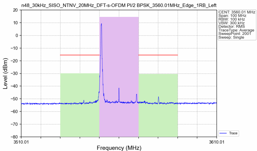
n48_30kHz_SISO_NTNV_20MHz_DFT-s-OFDM PI/2 BPSK_3560.01MHz_Edge_1RB_Left_Ant6
