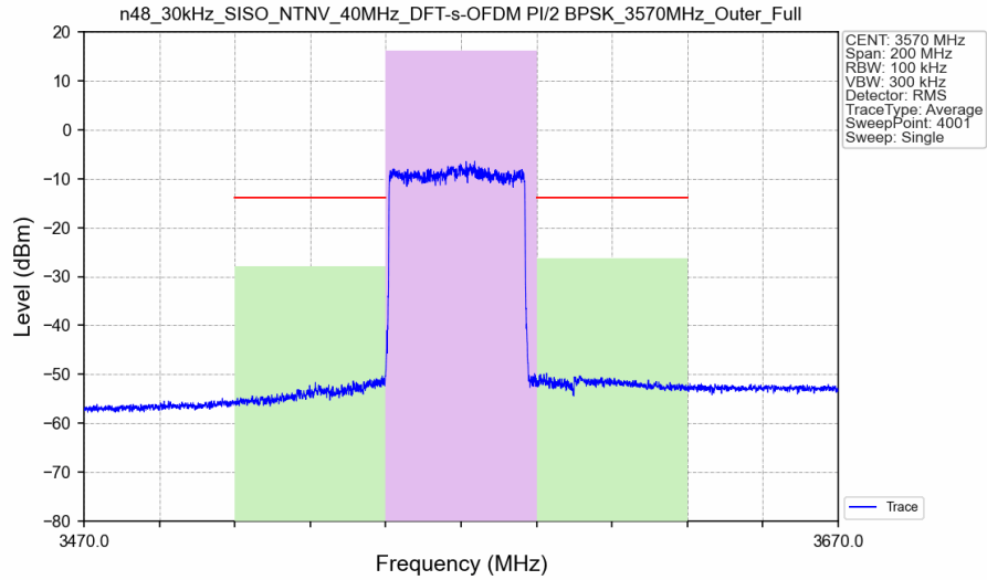
n48_30kHz_SISO_NTNV_40MHz_DFT-s-OFDM PI/2 BPSK_3570MHz_Outer_Full_Ant6
