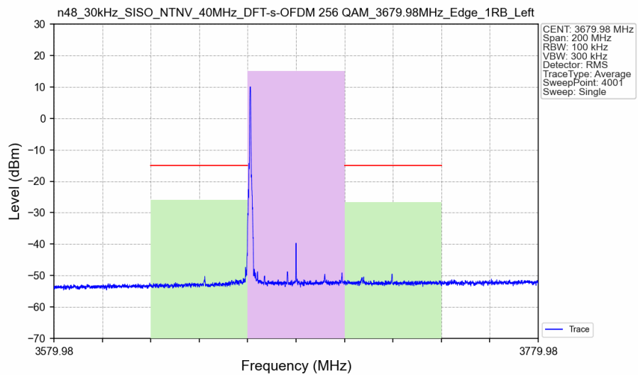
n48_30kHz_SISO_NTNV_40MHz_DFT-s-OFDM 256 QAM 3679.98MHz_Edge_1RB_Left_Ant6
