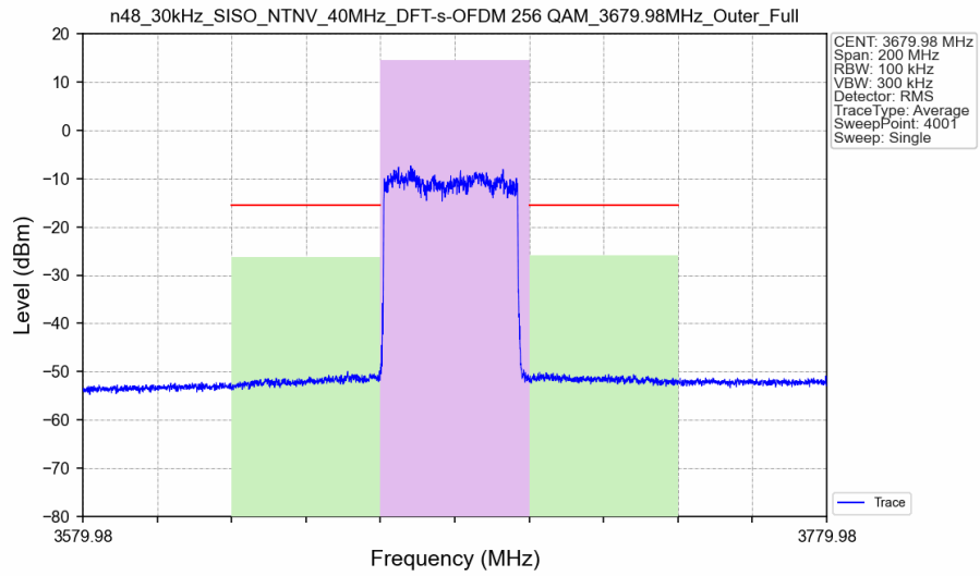
n48_30kHz_SISO_NTNV_40MHz_DFT-s-OFDM 256 QAM 3679.98MHz_Outer_Full_Ant6
