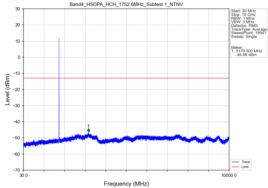
Band4_HSDPA_HCH_1752.6MHz_Subtest 1_NTNV
