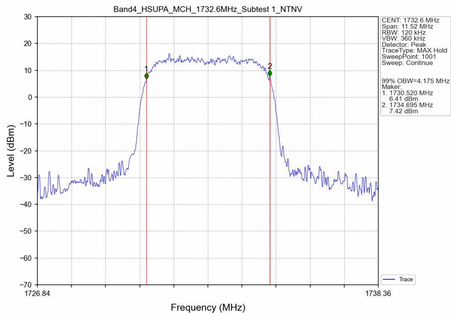
Band4_HSUPA_MCH_1732.6MHz_Subtest 1_NTNV
