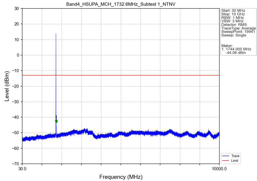
Band4_HSUPA_MCH_1732.6MHz_Subtest 1_NTNV
