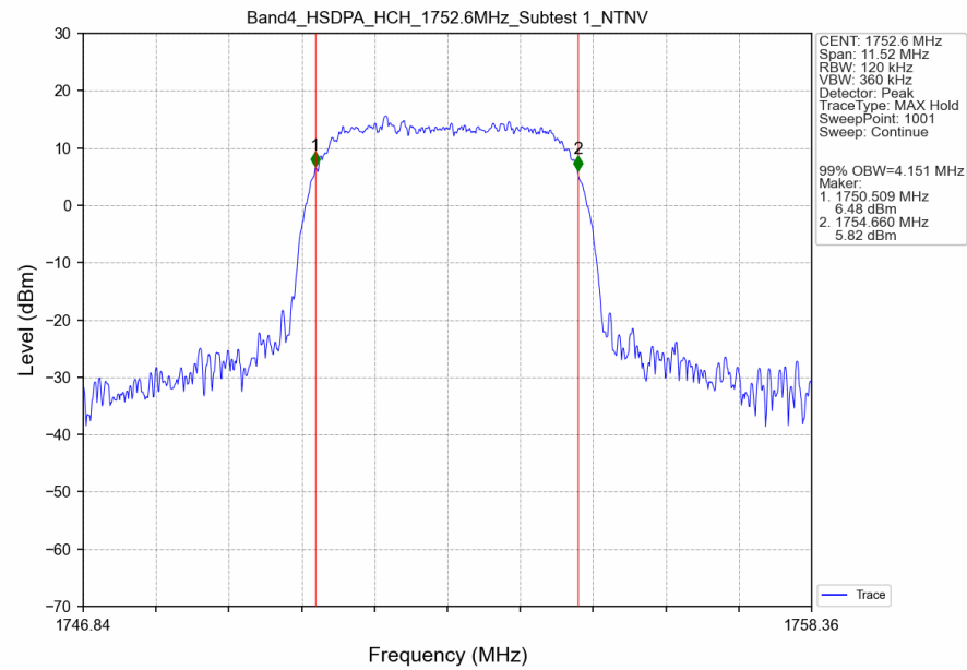
Band4_HSDPA_HCH_1752.6MHz_Subtest 1_NTNV
