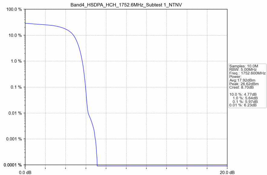
Band4_HSDPA_HCH_1752.6MHz_Subtest 1_NTNV
