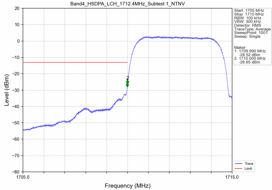
Band4_HSDPA_LCH_1712.4MHz_Subtest 1_NTNV
