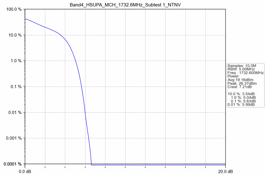
Band4_HSUPA_MCH_1732.6MHz_Subtest 1_NTNV
