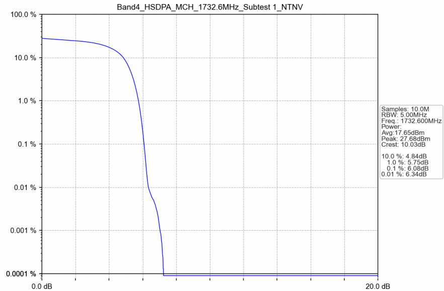
Band4_HSDPA_MCH_1732.6MHz_Subtest 1_NTNV
