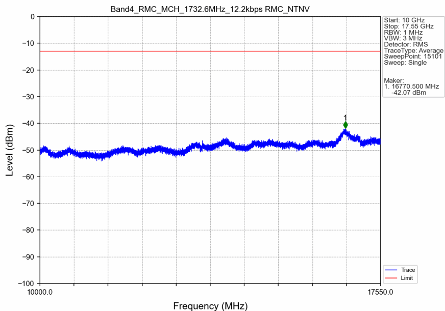
Band4_RMC_MCH_1732.6MHz_12.2kbps RMC_NTNV
