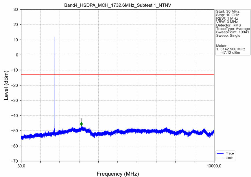
Band4_HSDPA_MCH_1732.6MHz_Subtest 1_NTNV
