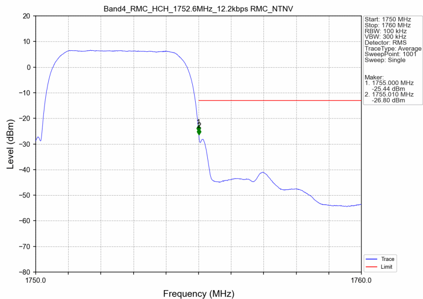
Band4_RMC_HCH_1752.6MHz_12.2kbps RMC_NTNV
