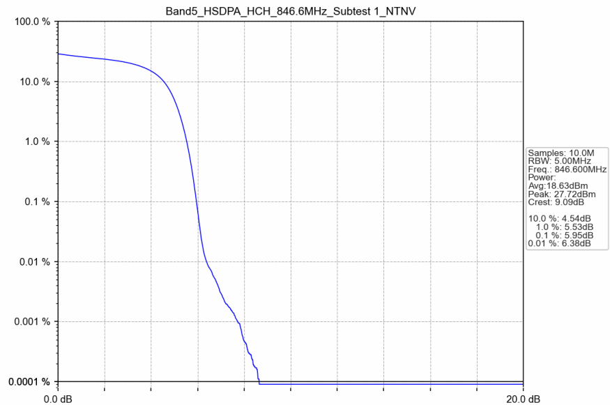
Band5_HSDPA_HCH_846.6MHz_Subtest 1_NTNV
