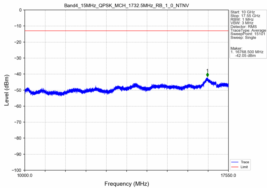
Band4_15MHz_QPSK_MCH_1732.5MHz_RB_1_0_NTNV
