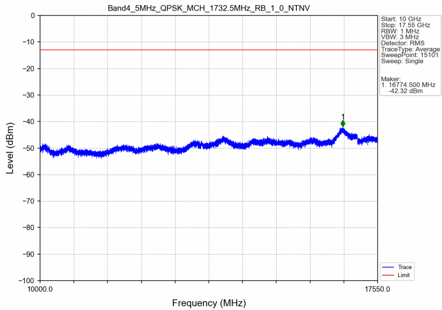
Band4_5MHz_QPSK_MCH_1732.5MHz_RB_1_0_NTNV
