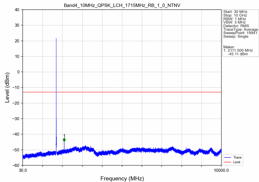
Band4_10MHz_QPSK_LCH_1715MHz_RB_1_0_NTNV
