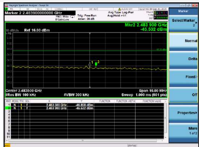
802.11n-40 MHz CHANNEL 9, BAND EDGE
