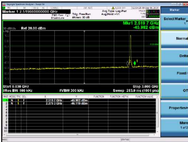
802.11b CHANNEL 6, SPURIOUS 30 MHz ~ 3 GHz
