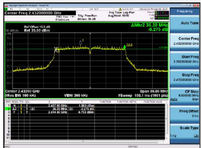
VHT-40 MHz CHANNEL 5
