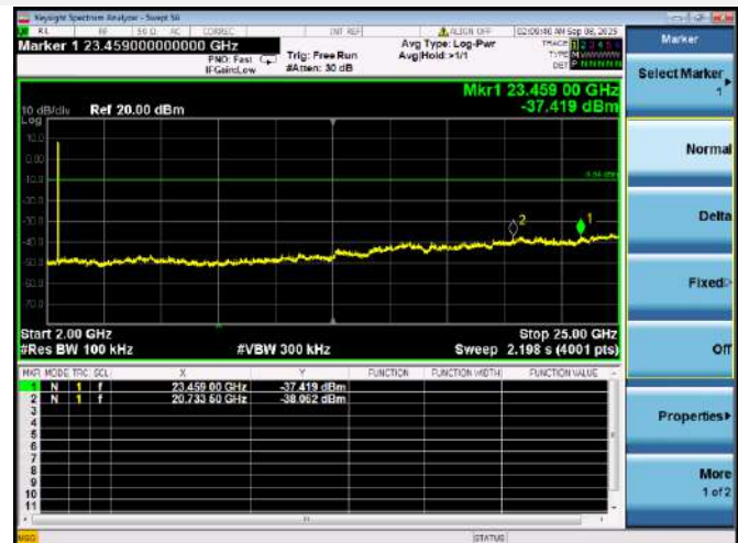
802.11b CHANNEL 11, SPURIOUS 2 GHz ~ 25 GHz
