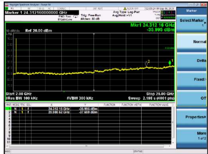
802.11b CHANNEL 6, SPURIOUS 2 GHz ~ 25 GHz
