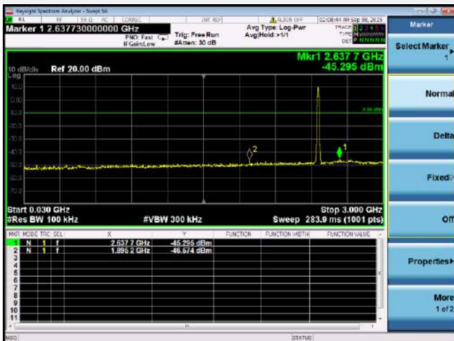
802.11b CHANNEL 11, SPURIOUS 30 MHz ~ 3 GHz
