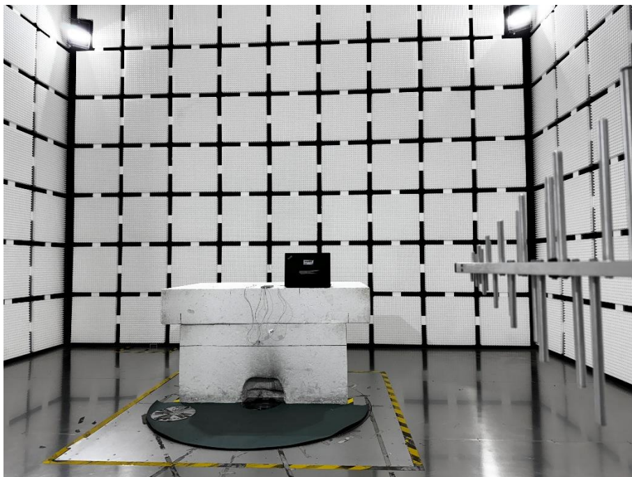
Below 1 GHz-USB Test Mode
