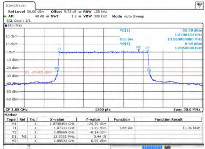
Band 2 16-QAM 15 MHz Bandwidth RB75#0 MCH
