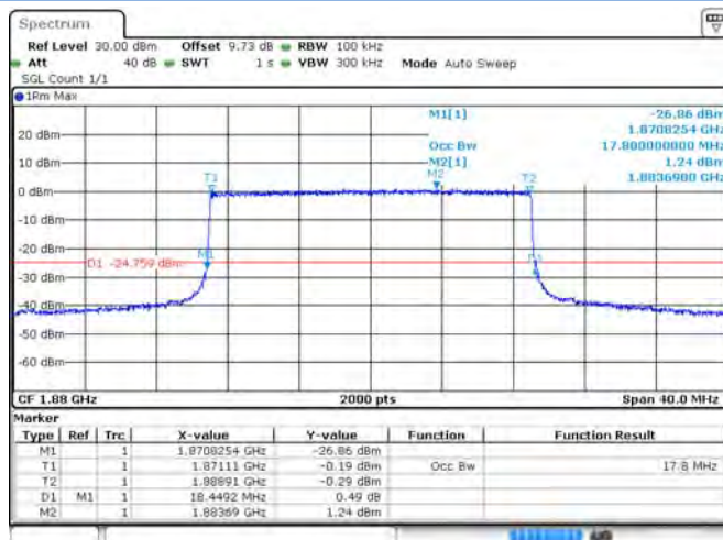
Band 2 QPSK 20 MHz Bandwidth RB100#0 MCH
