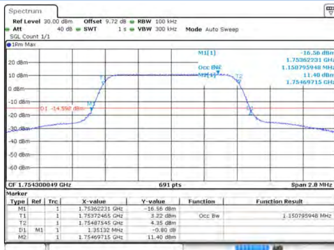
Band 4 16-QAM 1.4 MHz Bandwidth RB6#0 HCH
