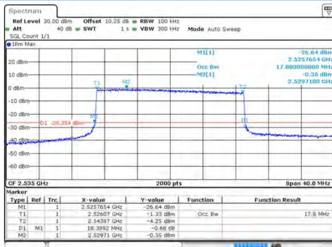
Band 7 16-QAM 20 MHz Bandwidth RB100#0 MCH
