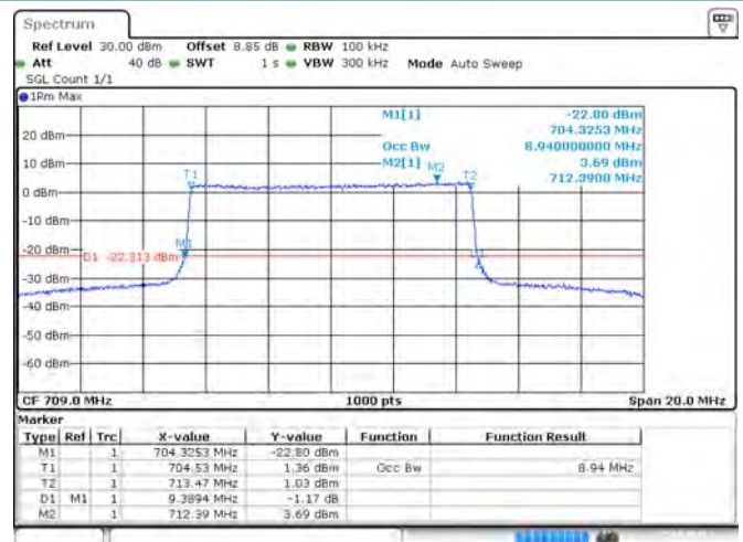
Band 17 16-QAM 10 MHz Bandwidth RB50#0 LCH
