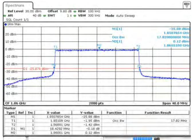
Band 2 16-QAM 20 MHz Bandwidth RB100#0 LCH
