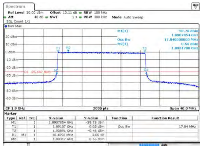
Band 2 16-QAM 20 MHz Bandwidth RB100#0 HCH
