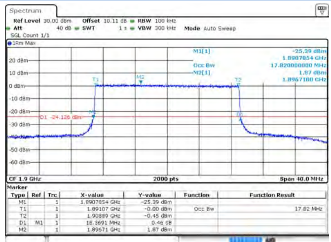
Band 2 QPSK 20 MHz Bandwidth RB100#0 HCH
