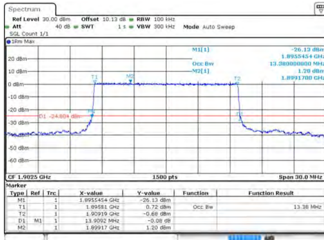
Band 2 16-QAM 15 MHz Bandwidth RB75#0 HCH
