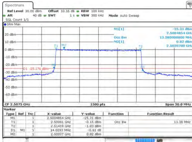
Band 7 16-QAM 15 MHz Bandwidth RB75#0 LCH
