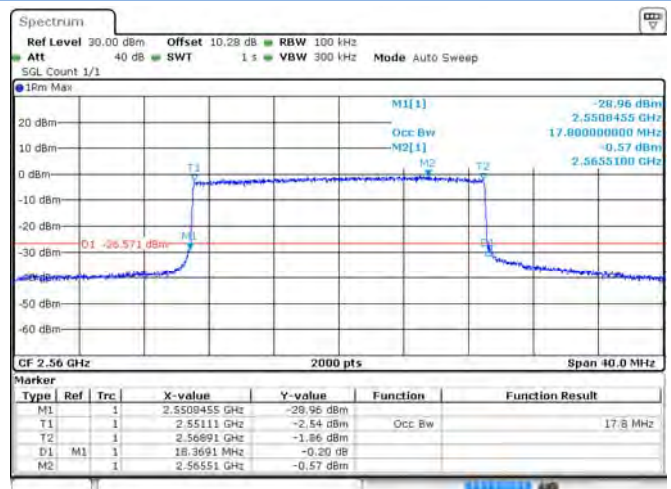
Band 7 16-QAM 20 MHz Bandwidth RB100#0 HCH
