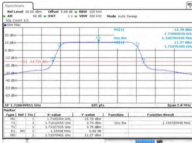
Band 4 16-QAM 1.4 MHz Bandwidth RB6#0 LCH
