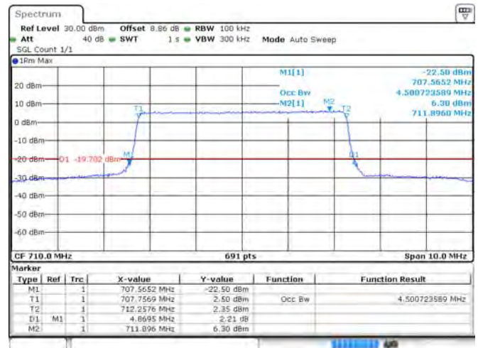
Band 17 16-QAM 5 MHz Bandwidth RB25#0 MCH
