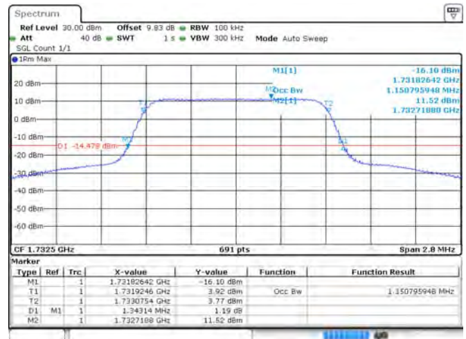
Band 4 16-QAM 1.4 MHz Bandwidth RB6#0 MCH
