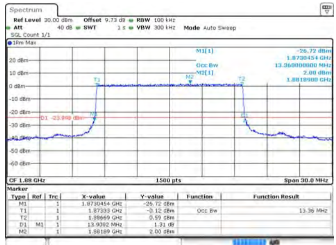
Band 2 QPSK 15 MHz Bandwidth RB75#0 MCH
