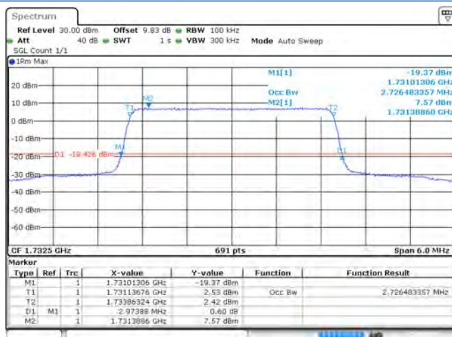
Band 4 16-QAM 3 MHz Bandwidth RB15#0 MCH
