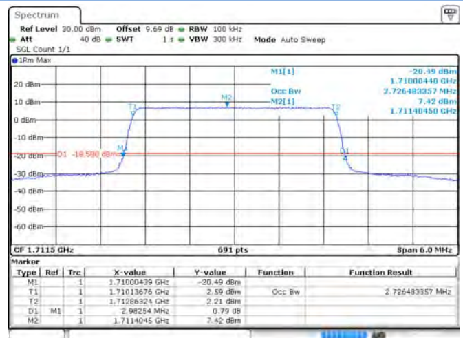
Band 4 16-QAM 3 MHz Bandwidth RB15#0 LCH
