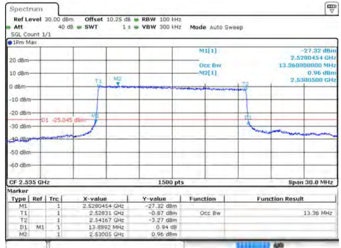
Band 7 16-QAM 15 MHz Bandwidth RB75#0 MCH
