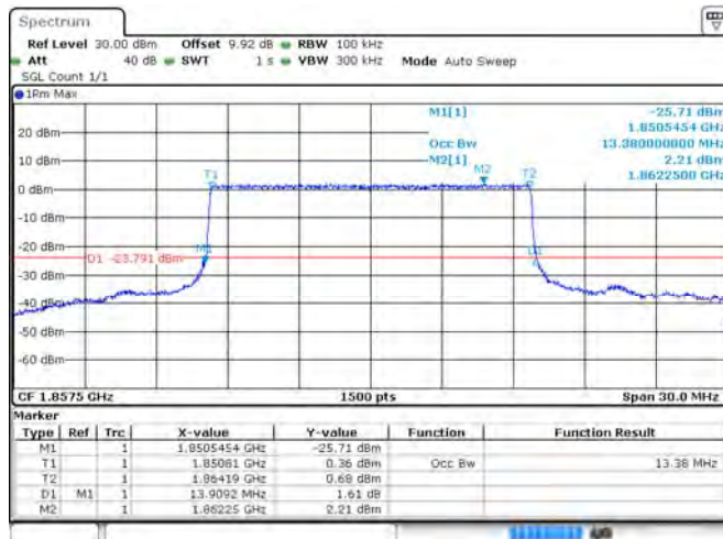
Band 2 QPSK 15 MHz Bandwidth RB75#0 LCH
