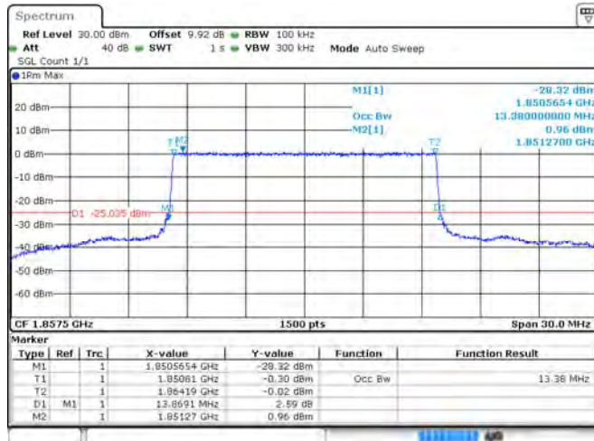
Band 2 16-QAM 15 MHz Bandwidth RB75#0 LCH
