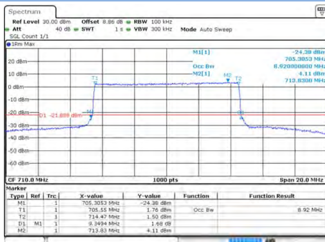
Band 17 16-QAM 10 MHz Bandwidth RB50#0 MCH
