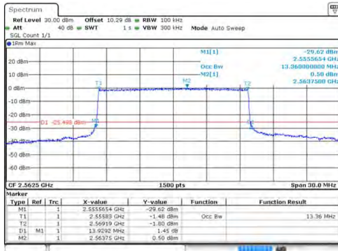
Band 7 16-QAM 15 MHz Bandwidth RB75#0 HCH
