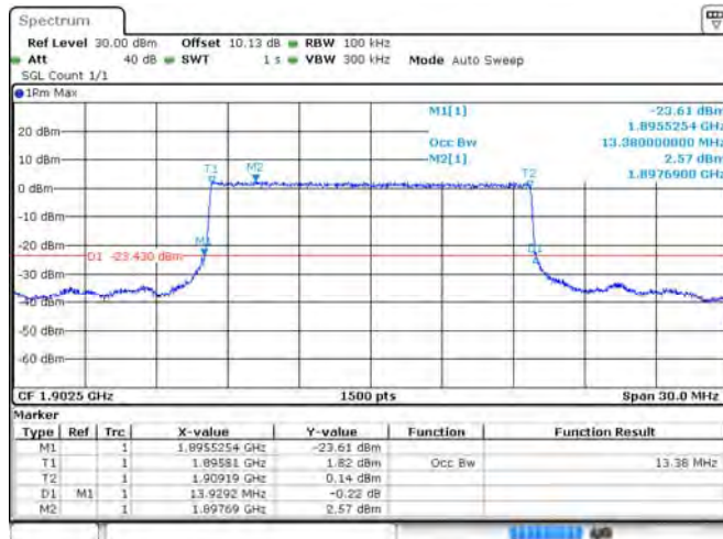
Band 2 QPSK 15 MHz Bandwidth RB75#0 HCH
