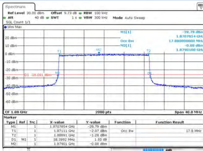
Band 2 16-QAM 20 MHz Bandwidth RB100#0 MCH
