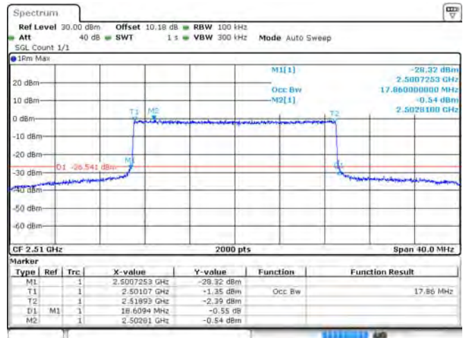
Band 7 16-QAM 20 MHz Bandwidth RB100#0 LCH
