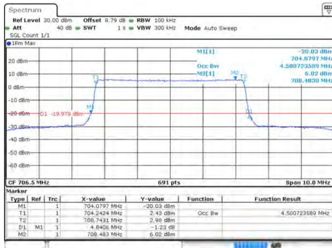
Band 17 16-QAM 5 MHz Bandwidth RB25#0 LCH
