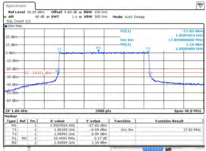
Band 2 QPSK 20 MHz Bandwidth RB100#0 LCH
