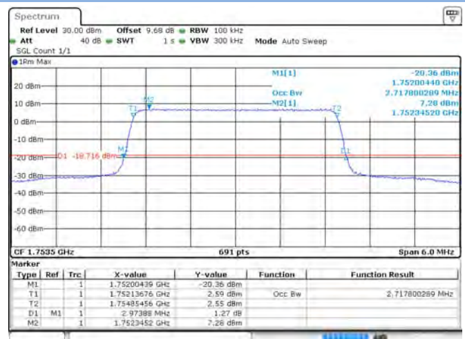
Band 4 16-QAM 3 MHz Bandwidth RB15#0 HCH
