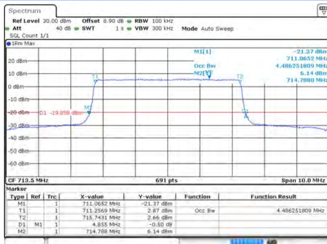
Band 17 16-QAM 5 MHz Bandwidth RB25#0 HCH
