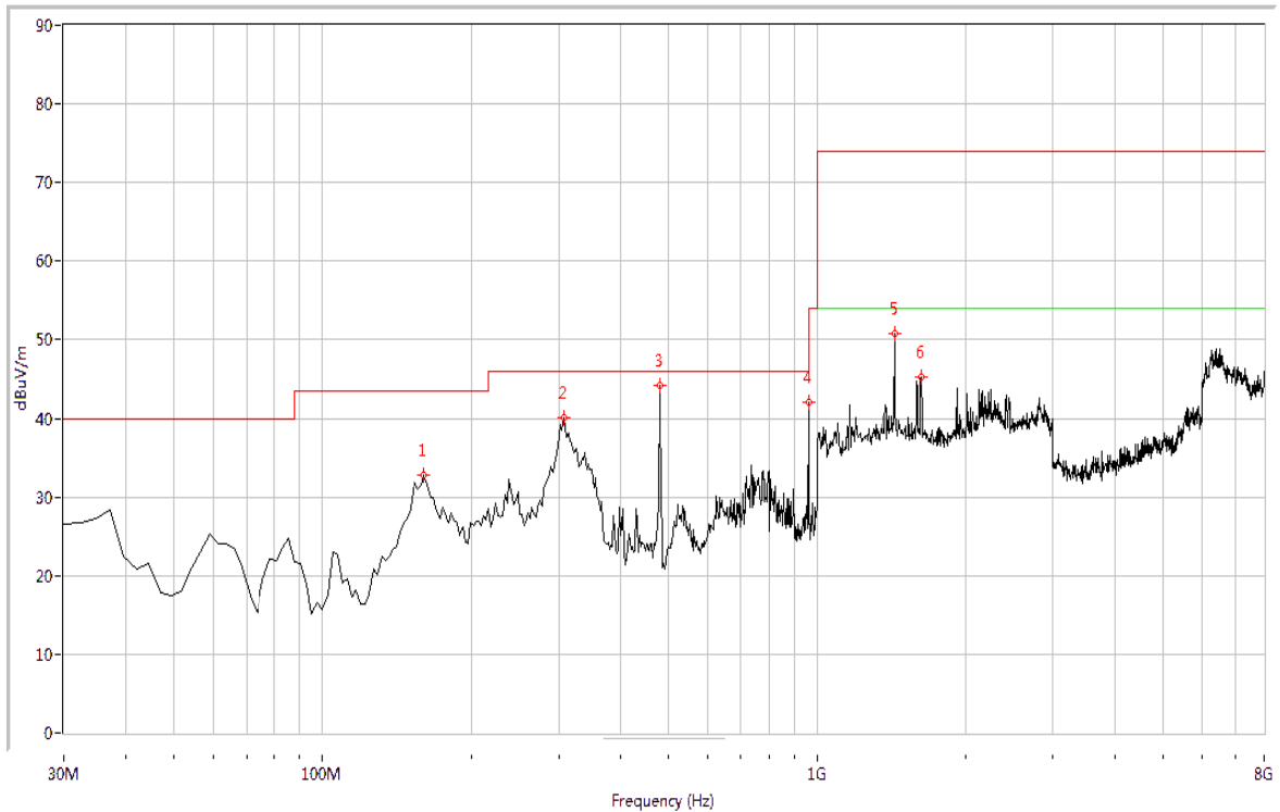
(Plot B: 30MHz – 8GHz, Test Antenna Horizontal)
