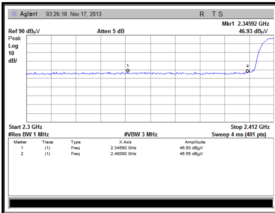
(Plot A1: Channel = 1 PEAK @ 802.11b)
