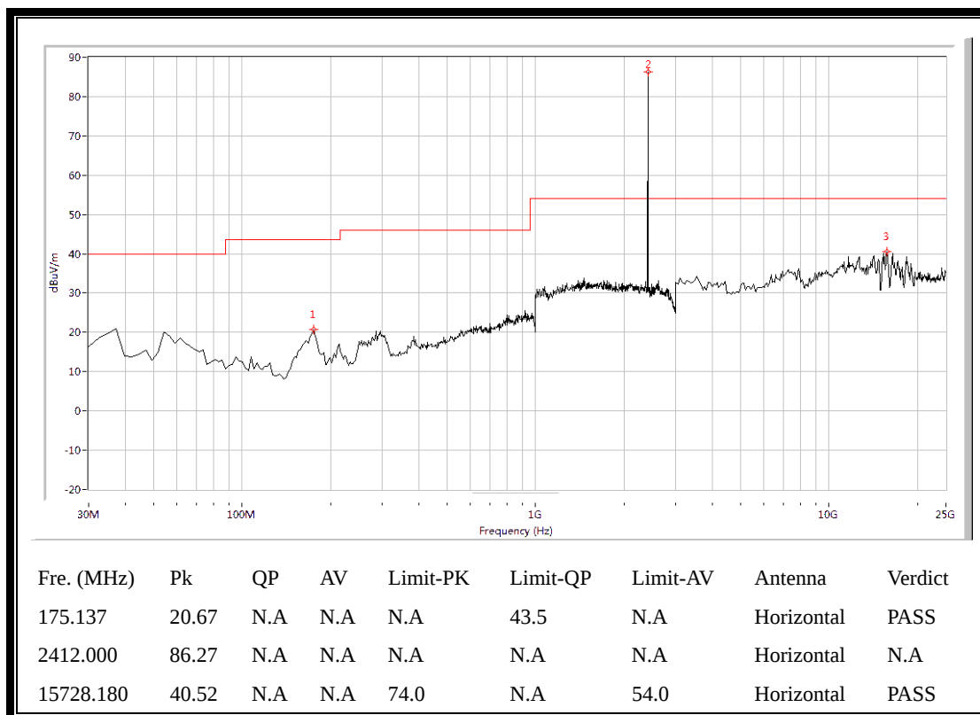
(Plot G.2: Antenna Horizontal, 30MHz to 25GHz)
