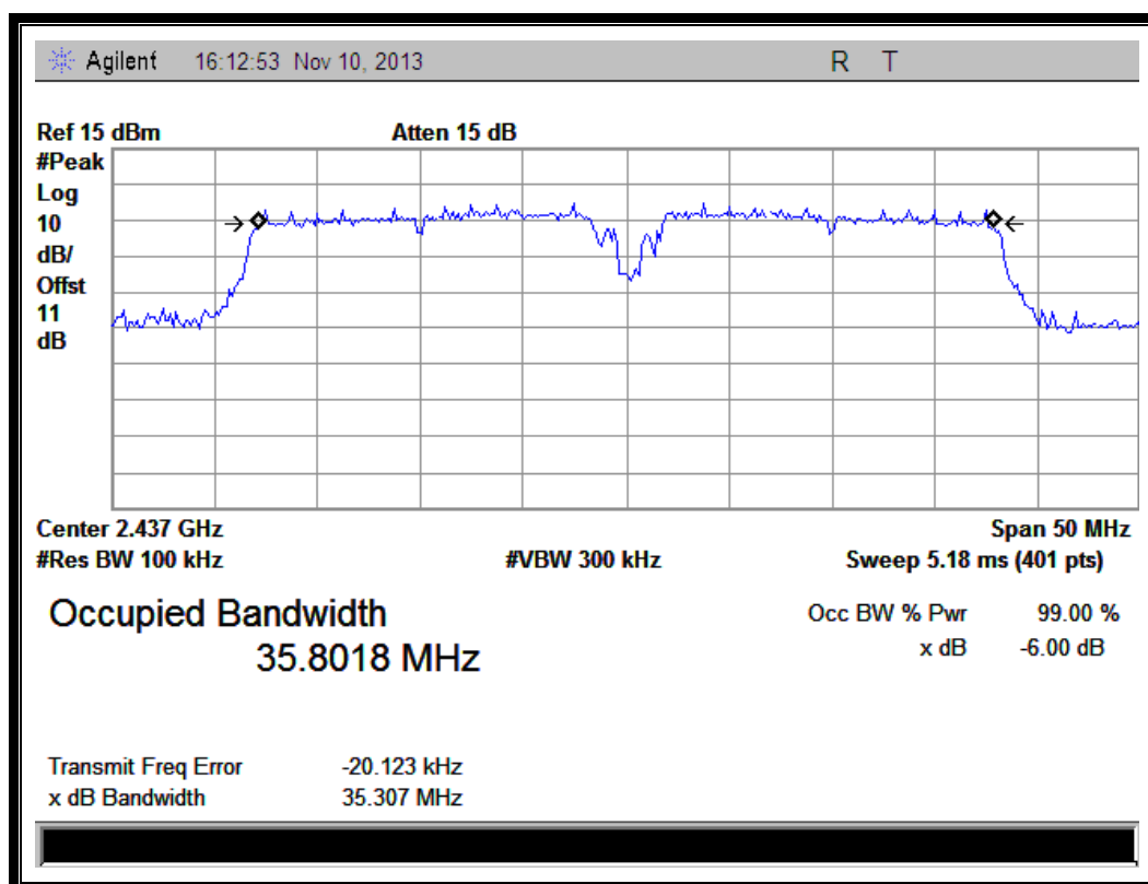
(Plot H: Channel 6: 2437MHz @ 802.11n-40)
