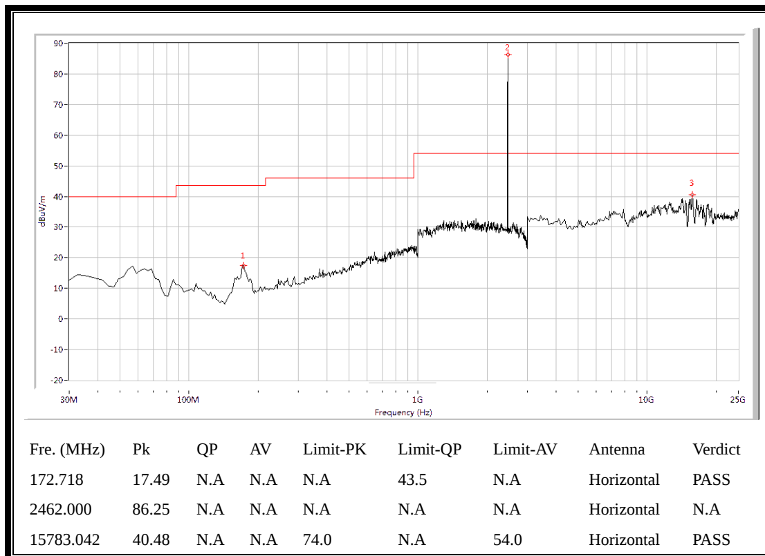
(Plot C.2: Antenna Horizontal, 30MHz to 25GHz)
