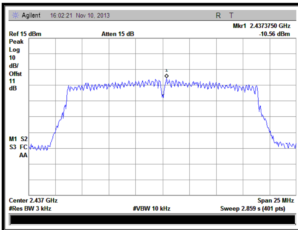
(Plot H: Channel = 6 @ 802.11n-20MHz)
