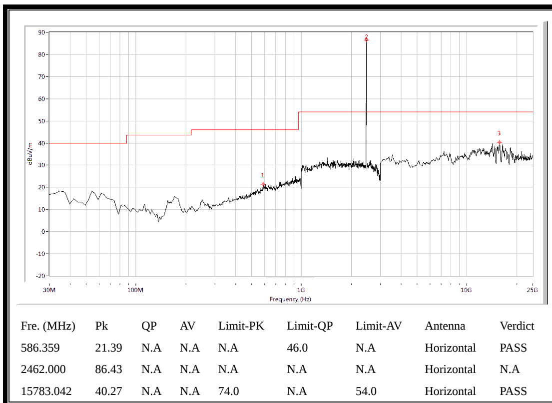
(Plot F.2: Antenna Horizontal, 30MHz to 25GHz)
