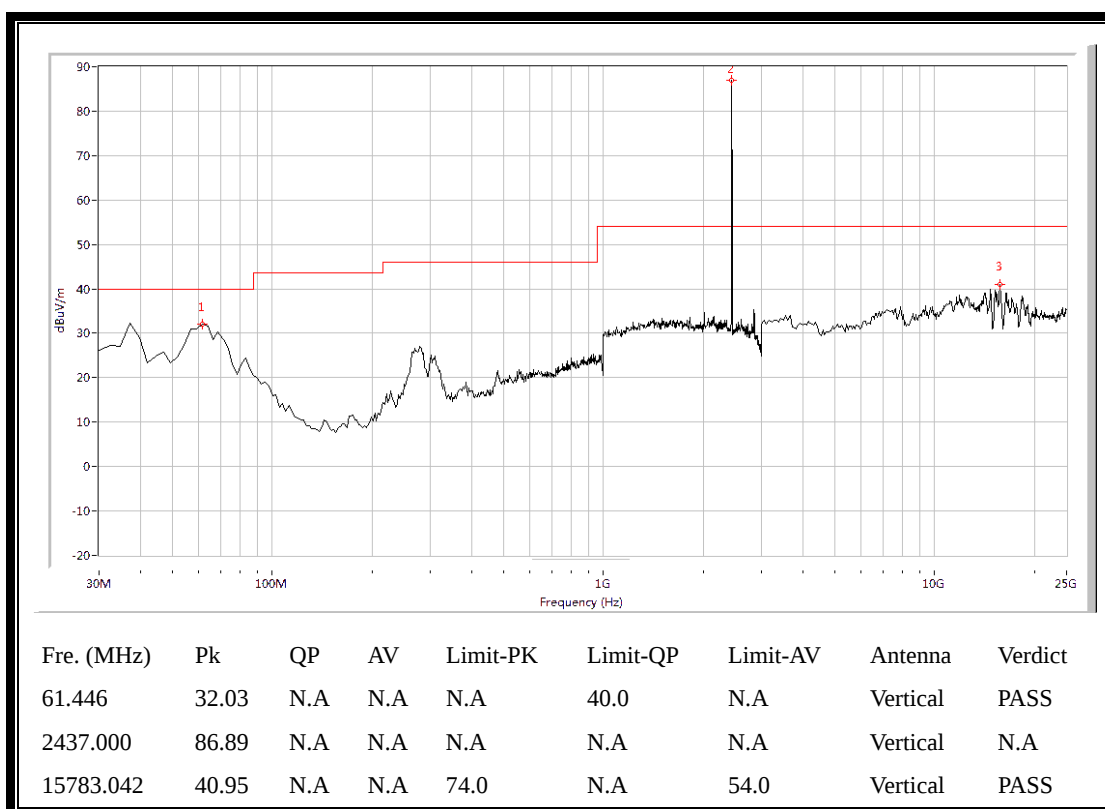
(Plot E.3: Antenna Vertical, 30MHz to 25GHz)
