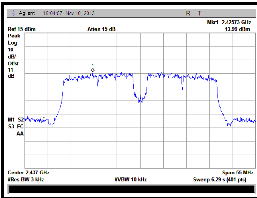
(Plot H: Channel = 6 @ 802.11n-40MHz)
