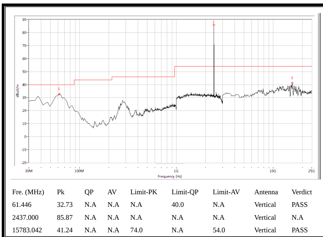
(Plot H.3: Antenna Vertical, 30MHz to 25GHz)
