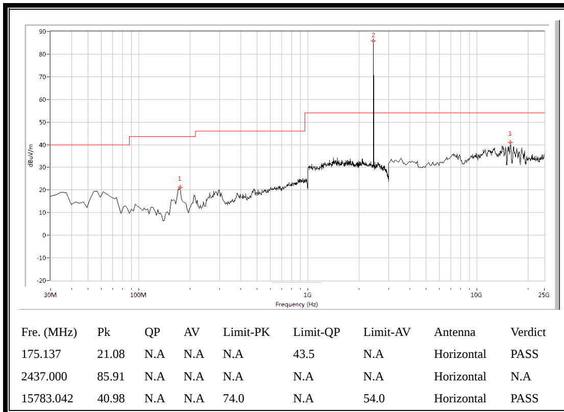
(Plot B.2: Antenna Horizontal, 30MHz to 25GHz)
