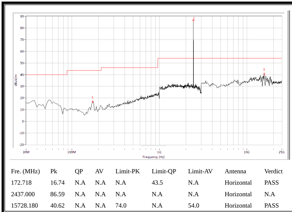
(Plot H.2: Antenna Horizontal, 30MHz to 25GHz)
