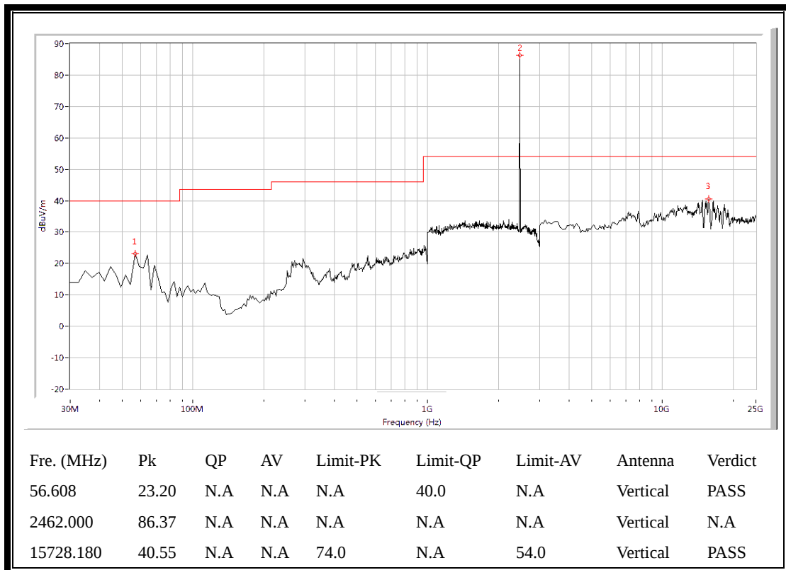
(Plot I.3: Antenna Vertical, 30MHz to 25GHz)
