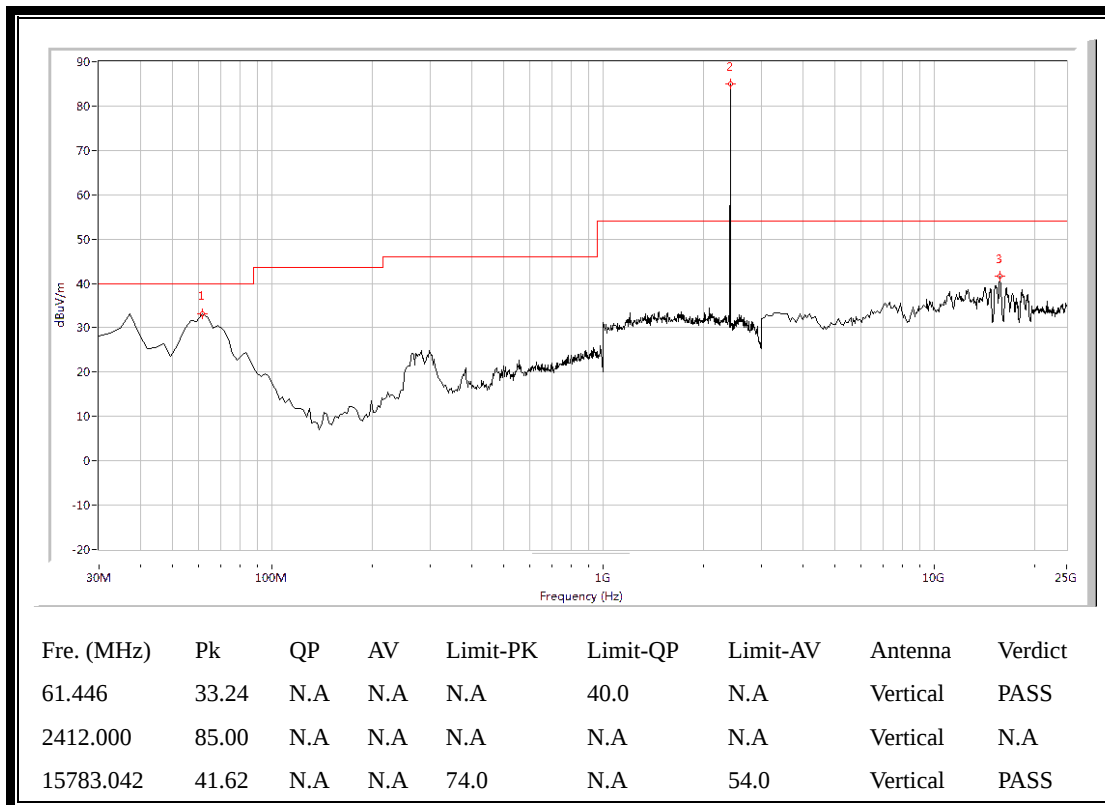
(Plot D.3: Antenna Vertical, 30MHz to 25GHz)
