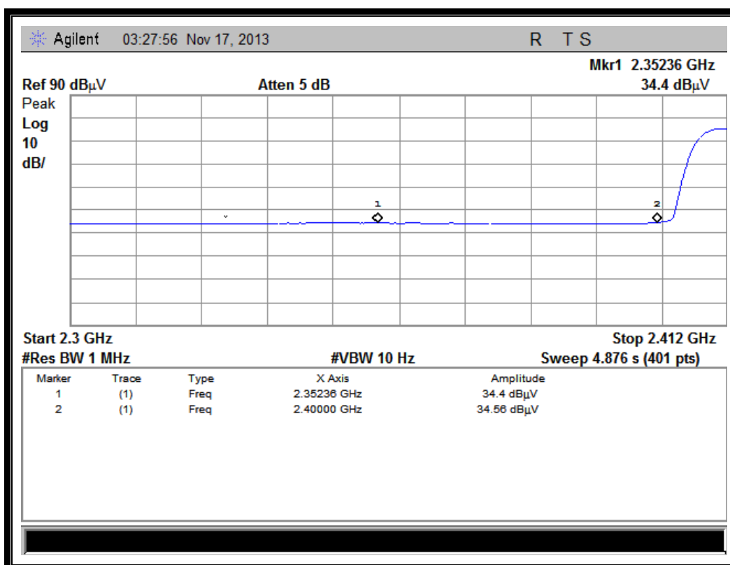
(Plot A2: Channel = 1 AVG @ 802.11b)
