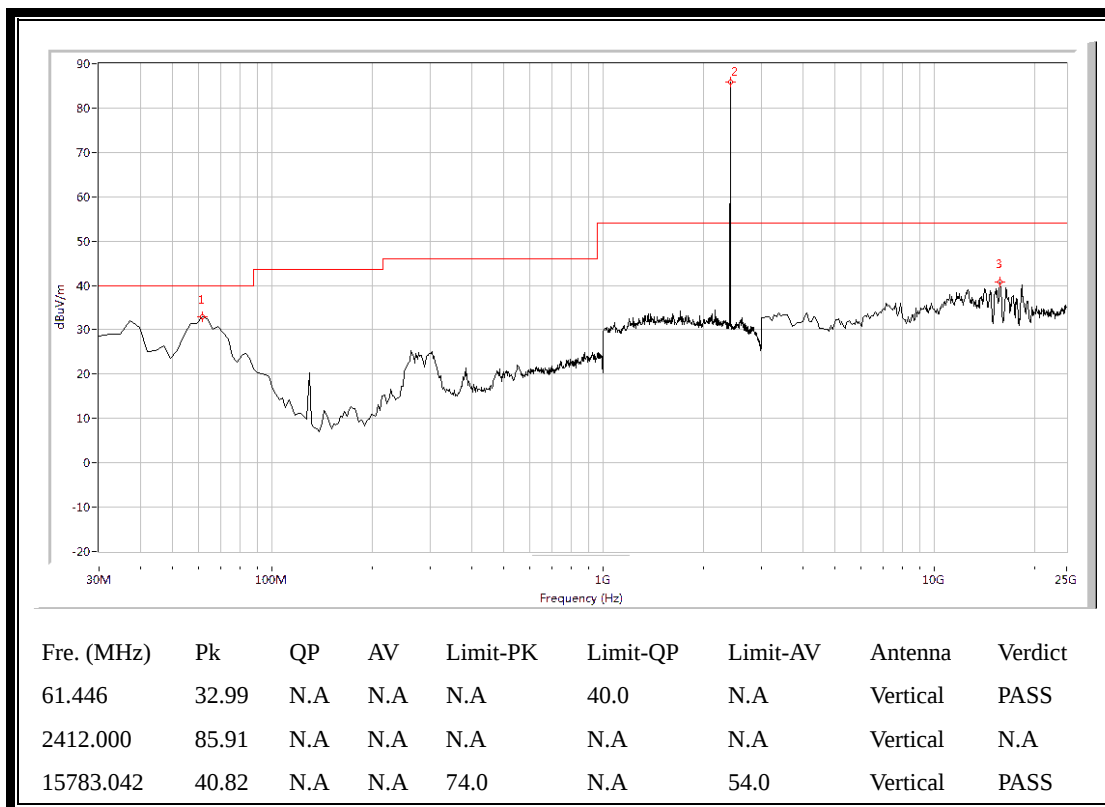
(Plot G.3: Antenna Vertical, 30MHz to 25GHz)
