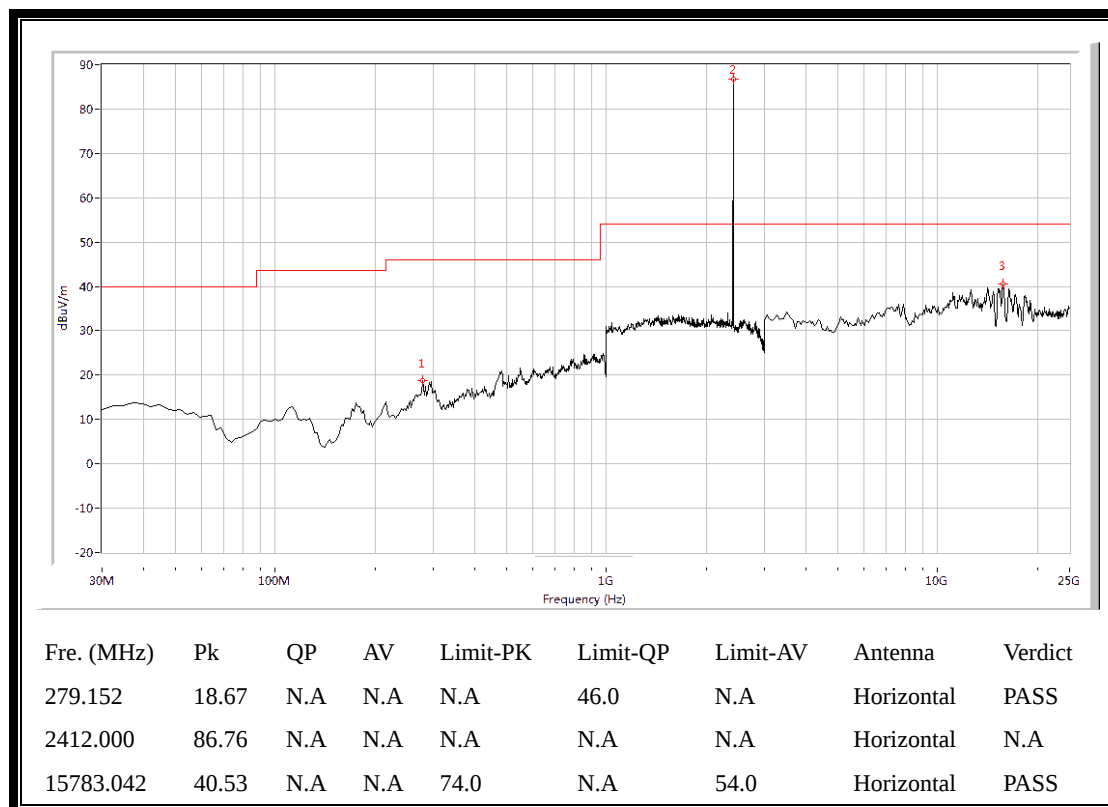
(Plot A.2: Antenna Horizontal, 30MHz to 25GHz)
