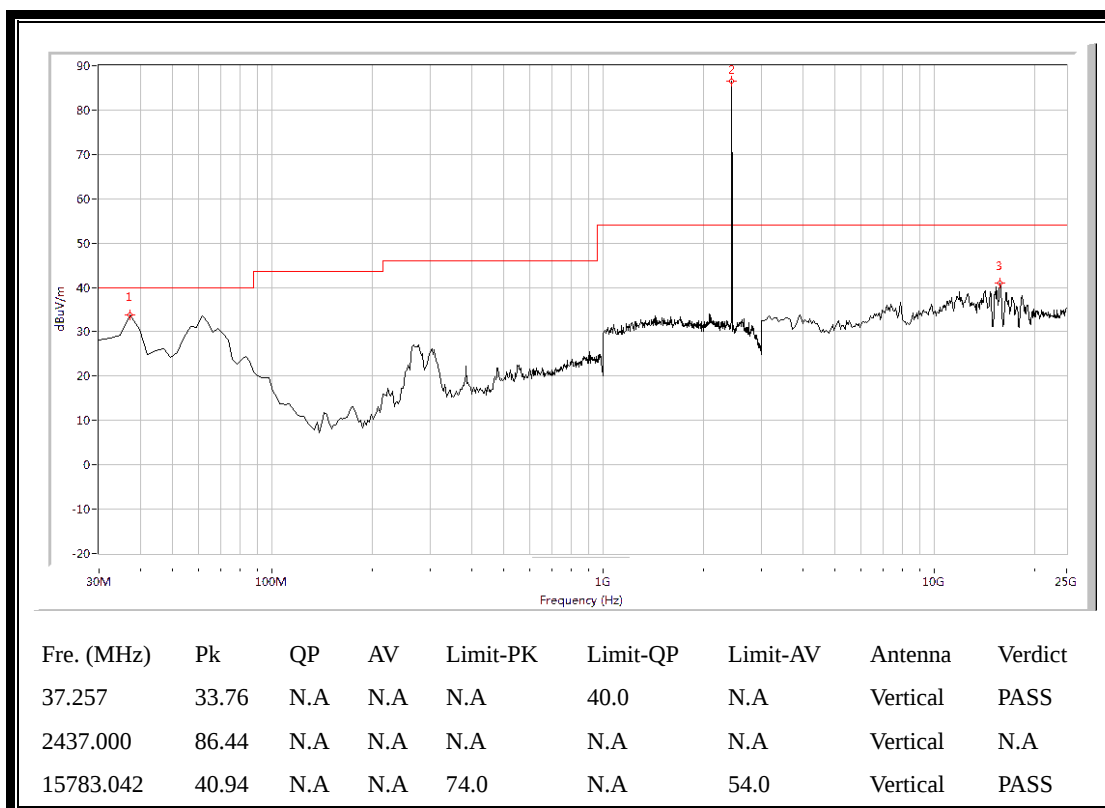
(Plot B.3: Antenna Vertical, 30MHz to 25GHz)
