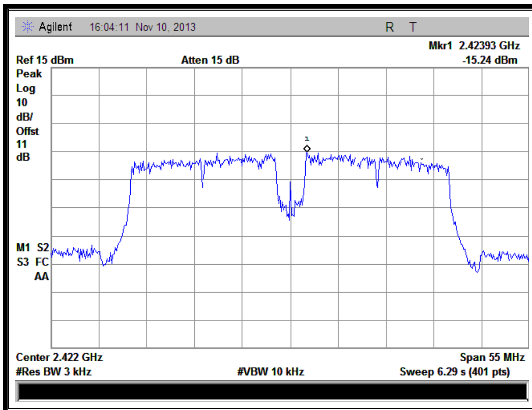
(Plot G: Channel = 3 @ 802.11n-40MHz)
