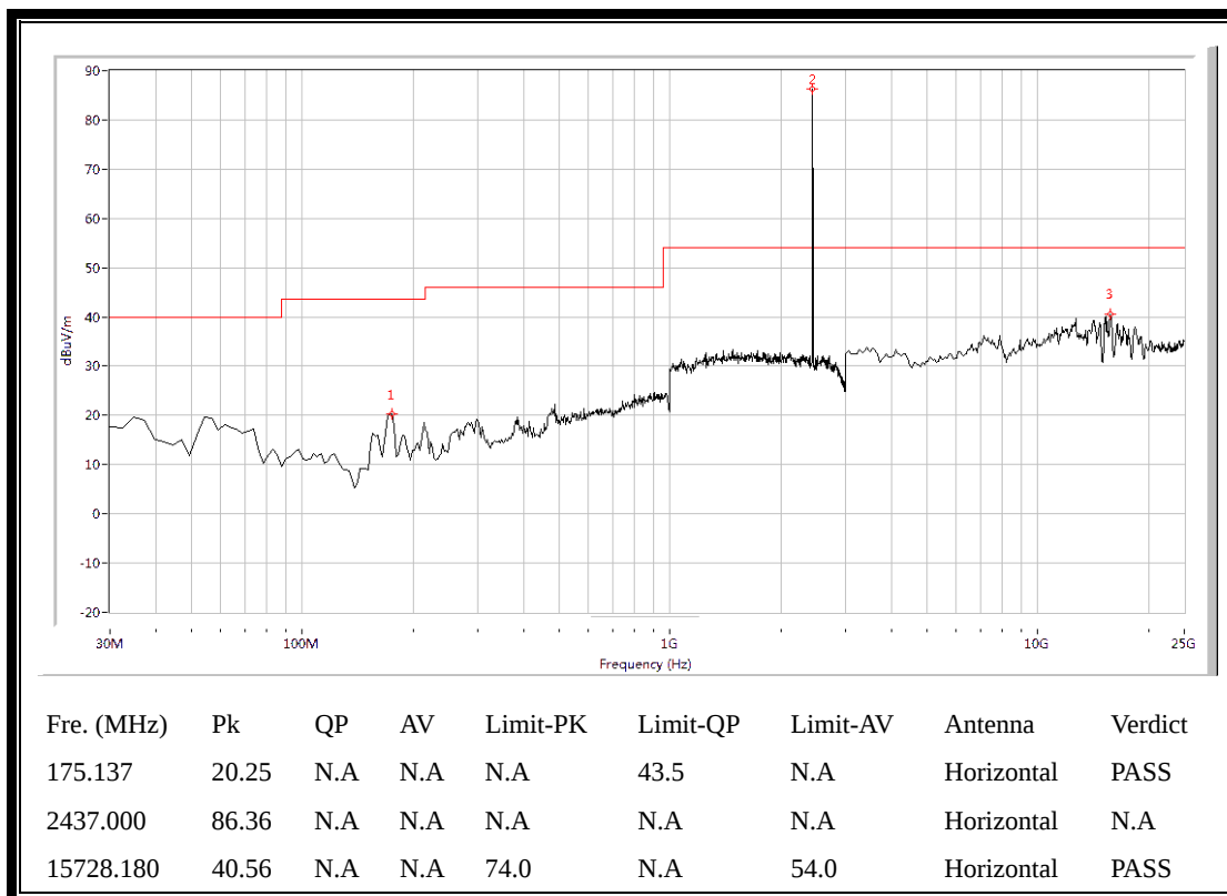
(Plot E.2: Antenna Horizontal, 30MHz to 25GHz)
