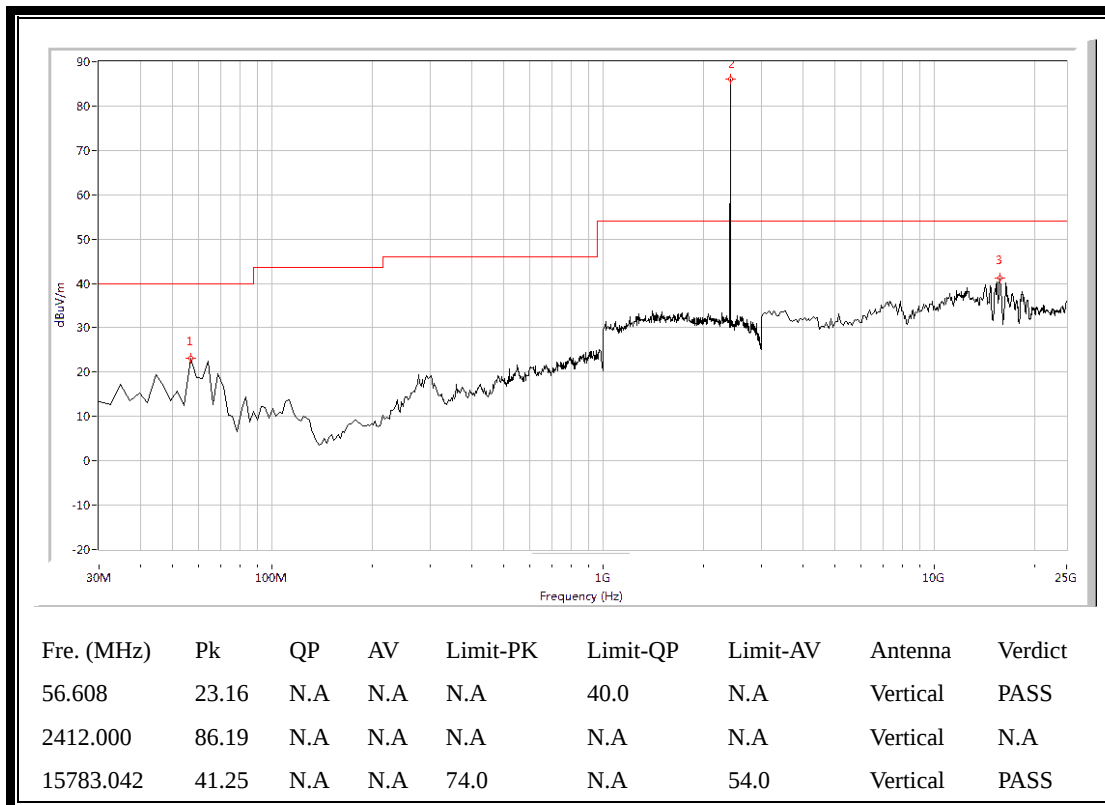
(Plot A.3: Antenna Vertical, 30MHz to 25GHz)
