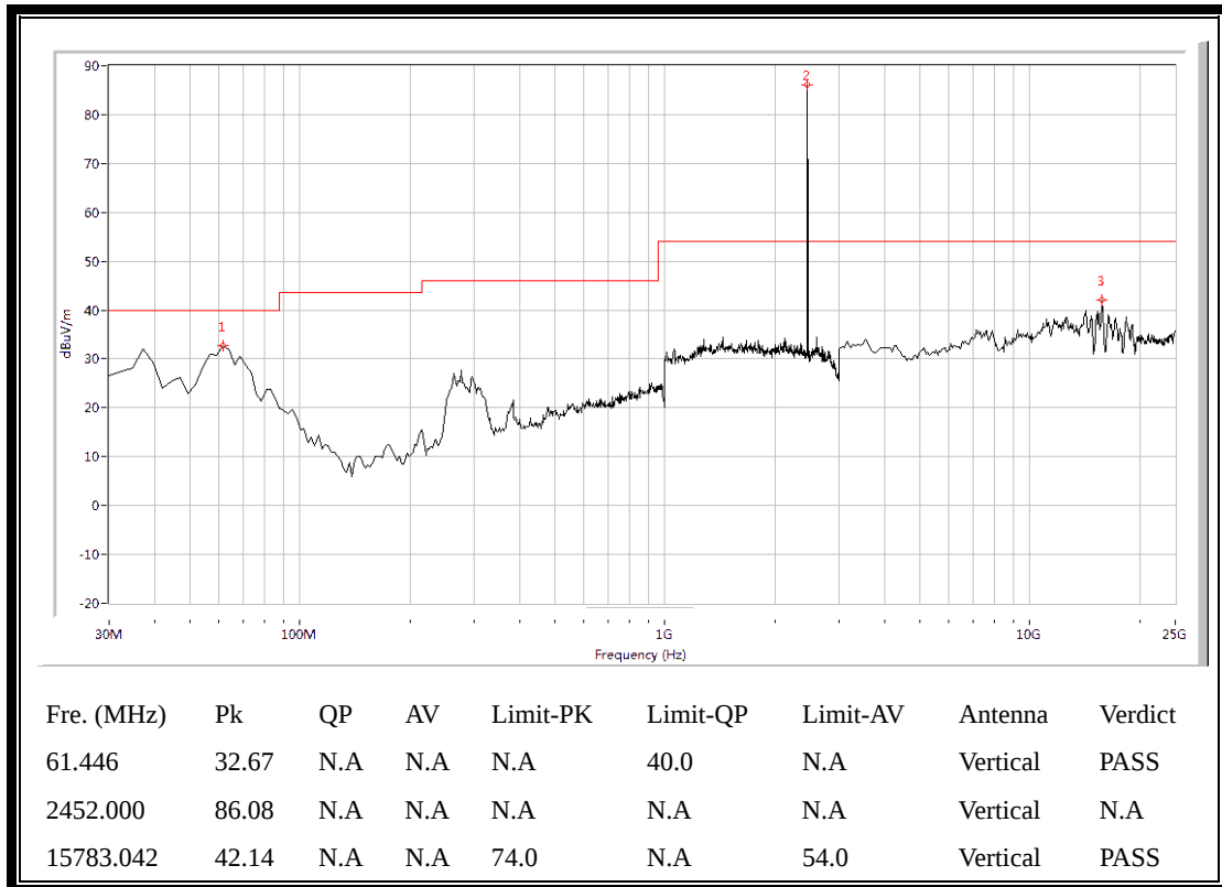
(Plot C.3: Antenna Vertical, 30MHz to 25GHz)
