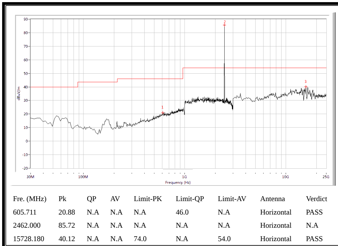
(Plot I.2: Antenna Horizontal, 30MHz to 25GHz)
