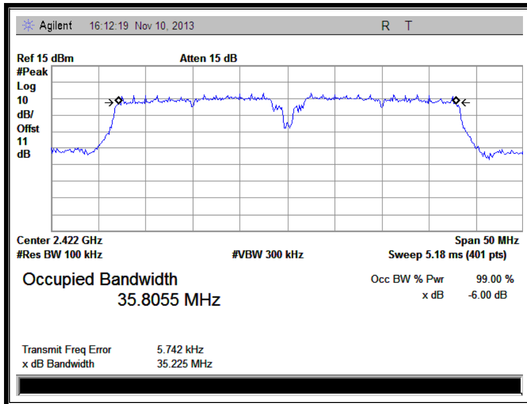
(Plot G: Channel 3: 2422MHz @ 802.11n-40)
