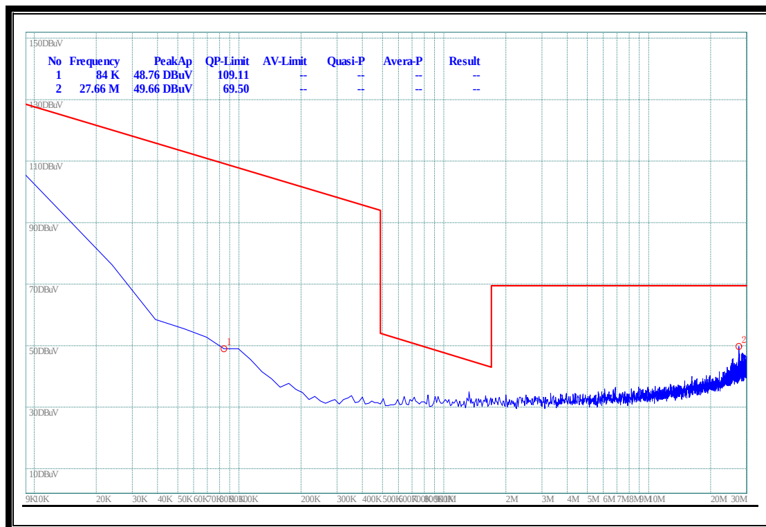
(Plot A.1: 9kHz to 30MHz)
