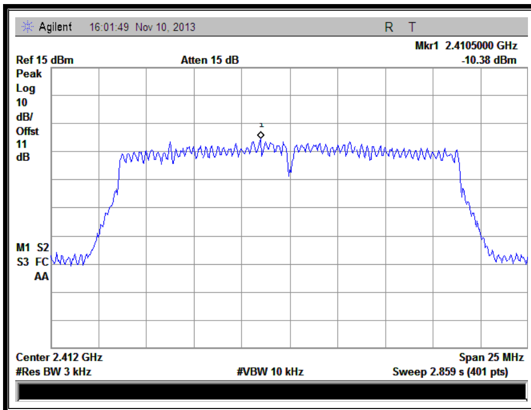
(Plot G: Channel = 1 @ 802.11n-20MHz)
