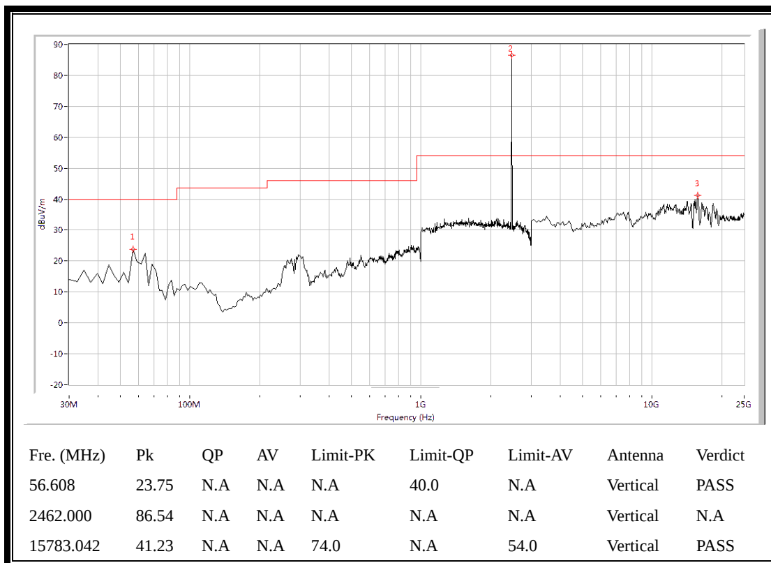
(Plot F.3: Antenna Vertical, 30MHz to 25GHz)
