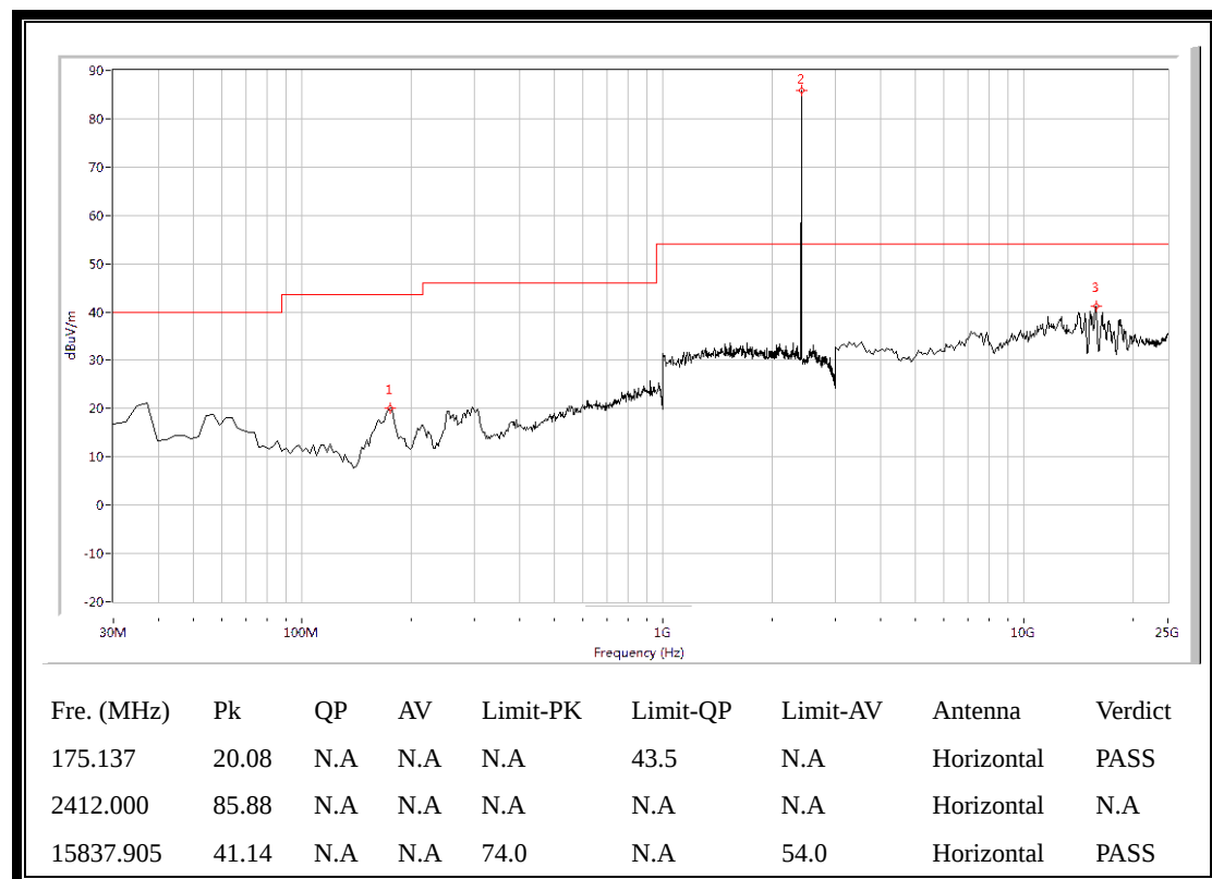
(Plot D.2: Antenna Horizontal, 30MHz to 25GHz)
