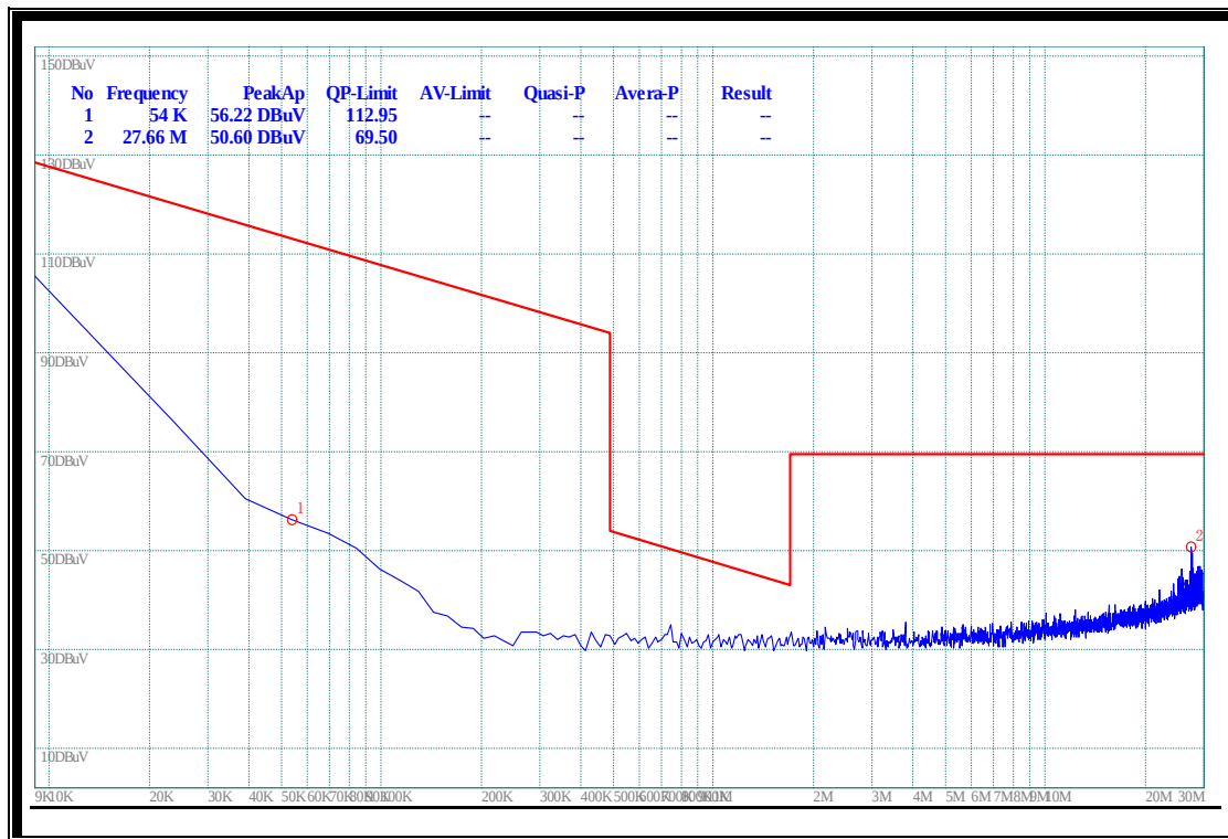
(Plot D.1: 9kHz to 30MHz)
