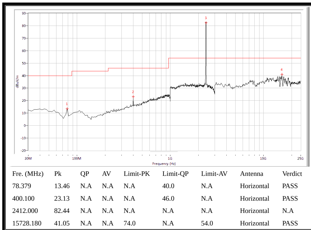
(Plot D.2: Antenna Horizontal, 30MHz to 25GHz)
