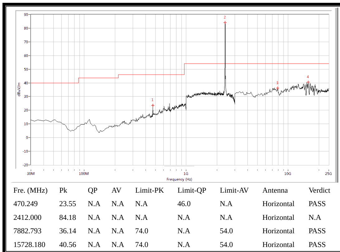
(Plot G.2: Antenna Horizontal, 30MHz to 25GHz)
