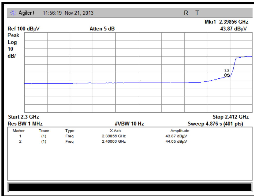
(Plot C2: Channel = 1 AVG @ 802.11g)
