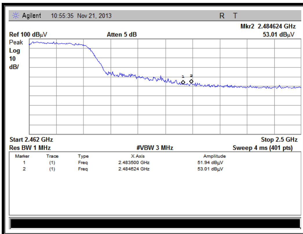
(Plot D1: Channel = 11 PEAK @ 802.11g)
