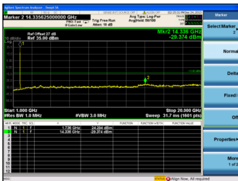
(Plot O2.1: HSUPA 1700MHz Channel = 1412, 1GHz to 20GHz)
