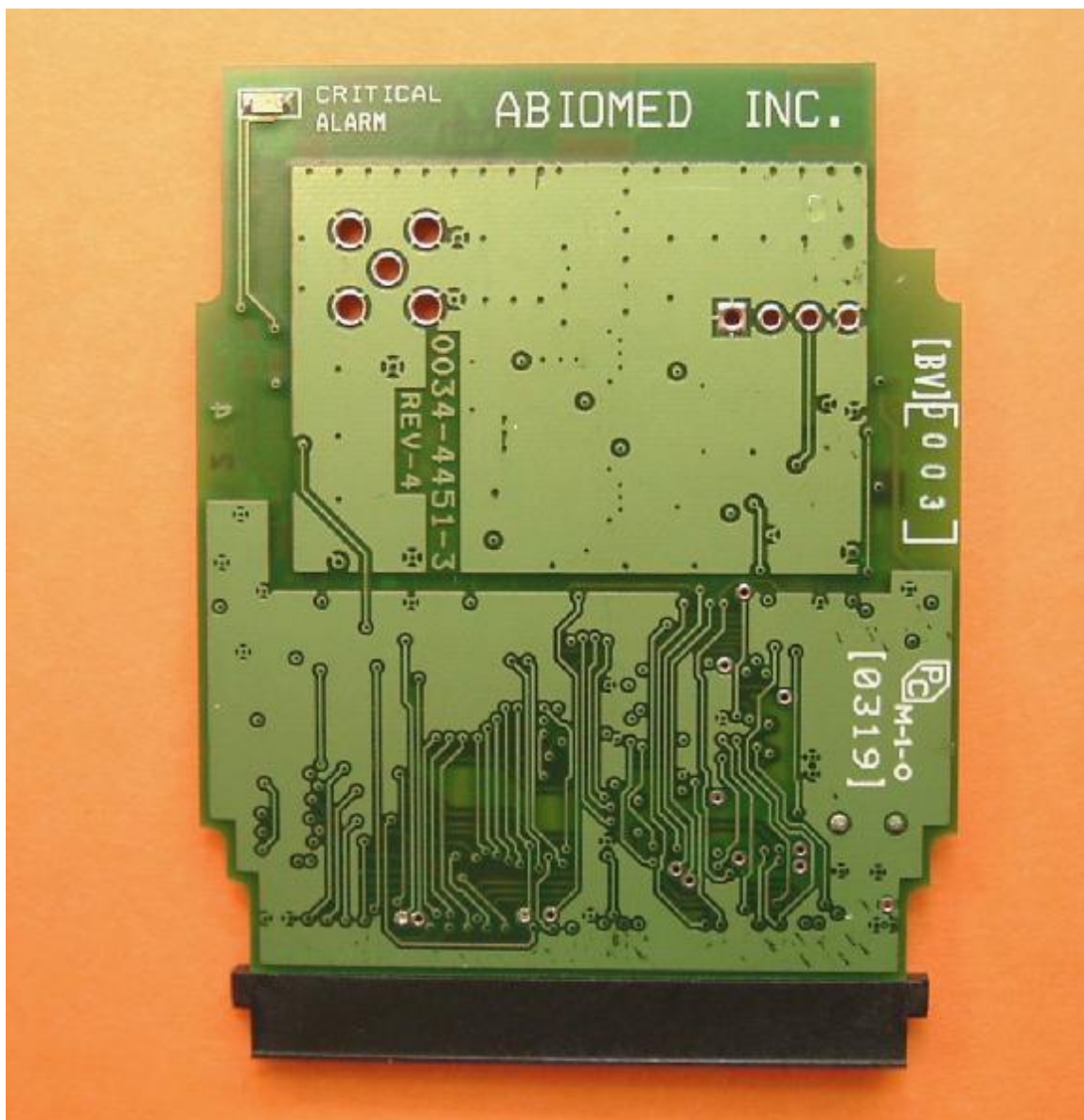
0034-4590 Handheld Monitor – PCB Bottom View
