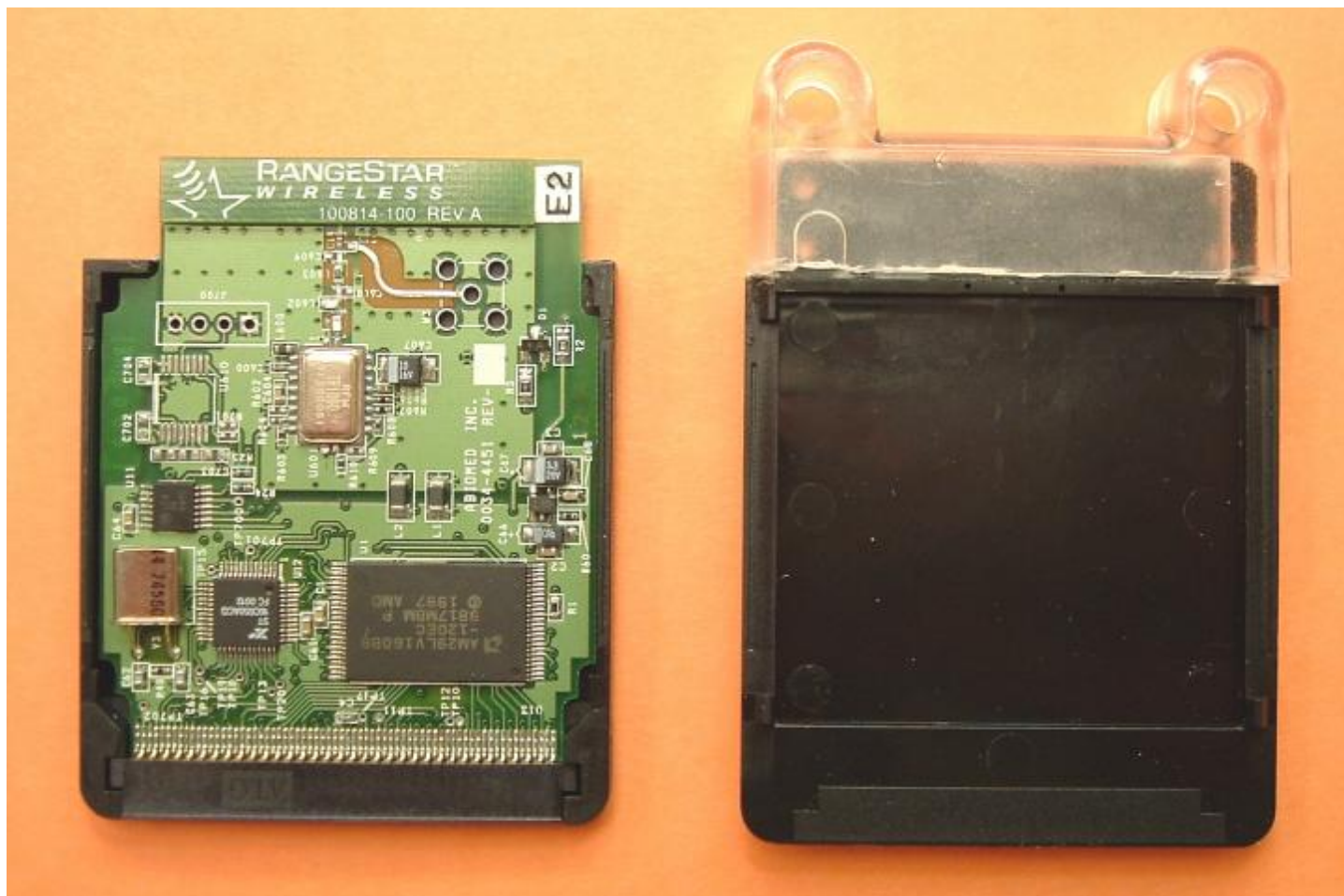
0034-4590 Handheld Monitor – Open ModuleView
