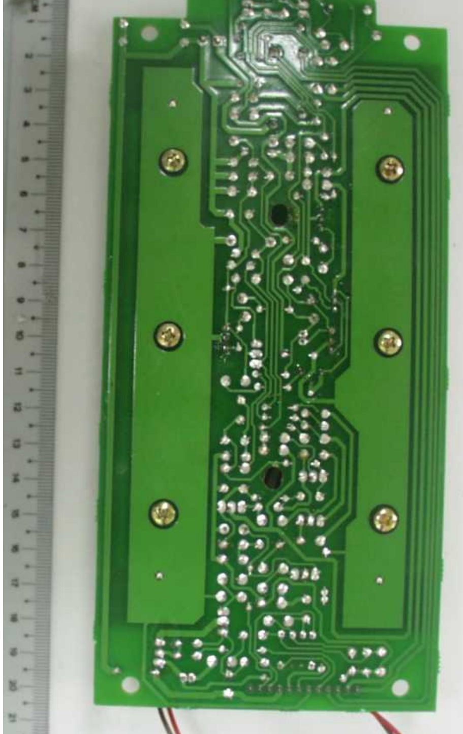
Rear Left/Right Speaker – Amplifier Board Trace Side
