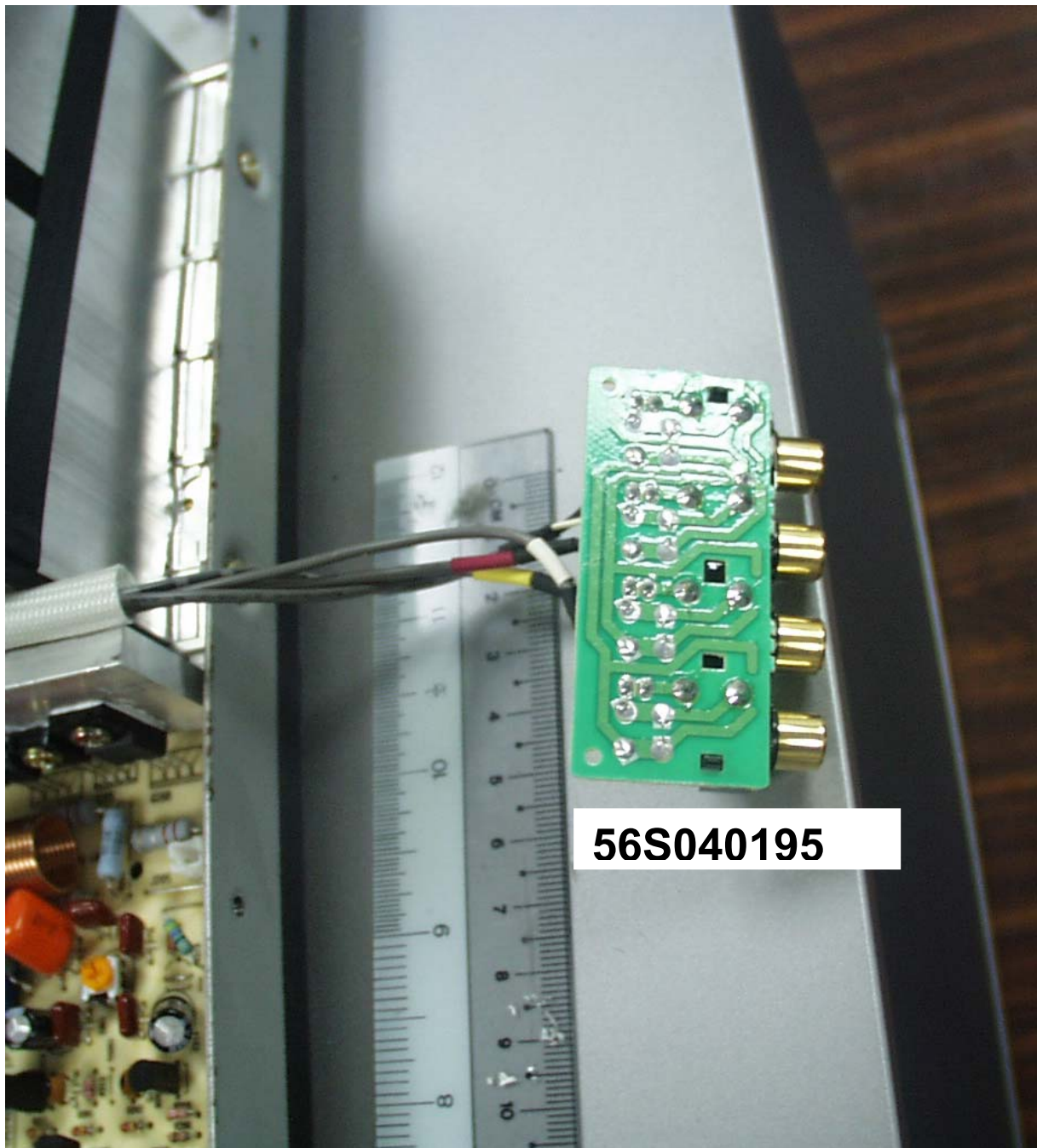
Subwoofer – Connector Board Trace Side
