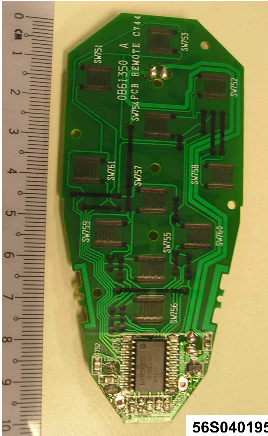
Sub Remote Control – Bottom View
