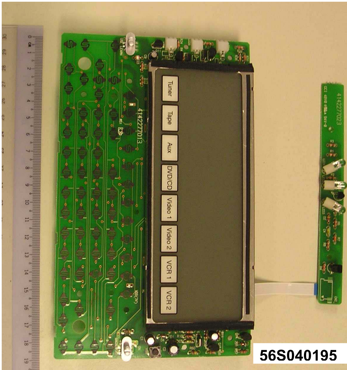
Main Control Unit – Top View
