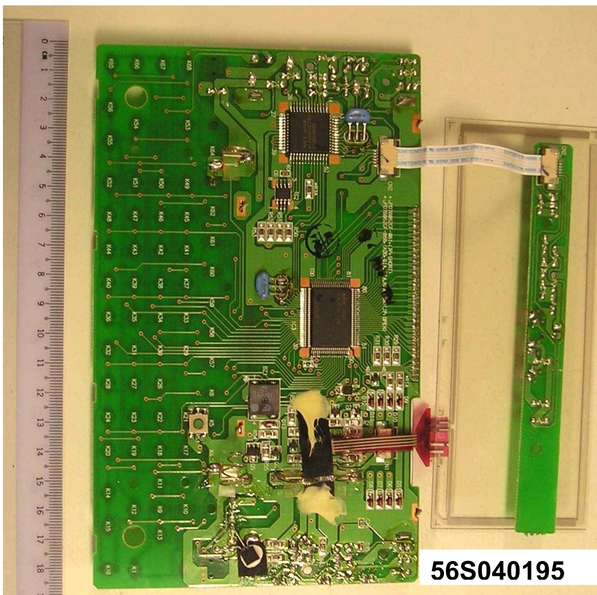
Main Control Unit – Bottom View
