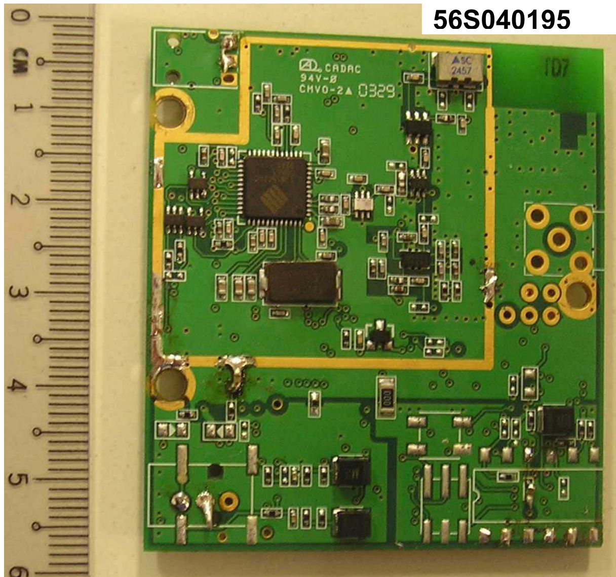
Rear Left/Right Speaker – RF Board Trace Side
