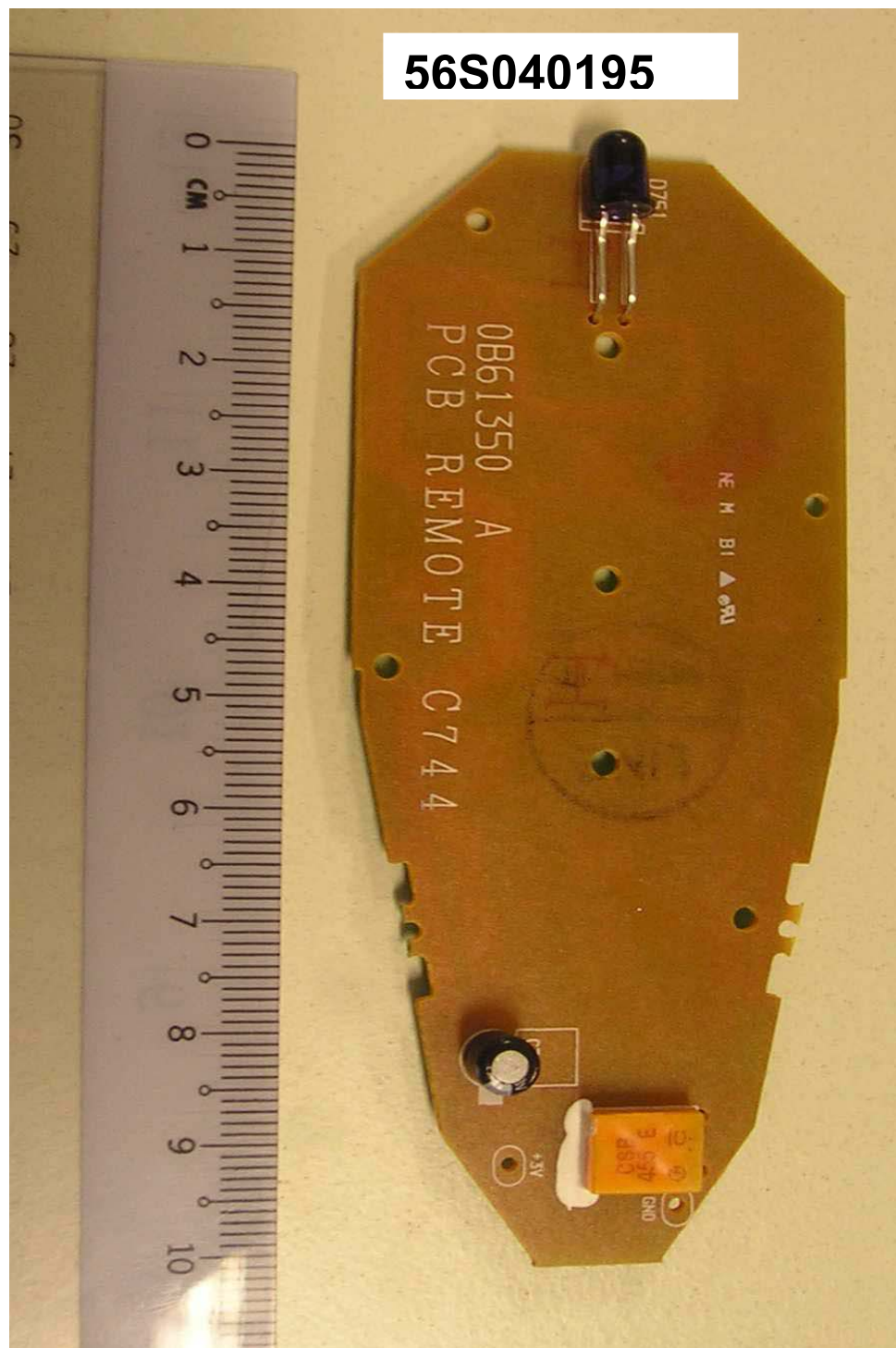
Sub Remote Control – Top View
