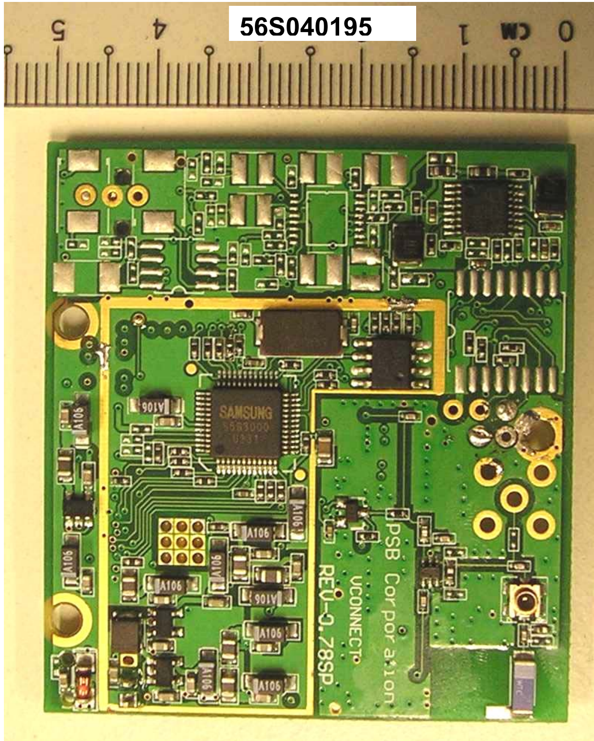
Rear Left/Right Speaker – RF Board Component Side (With RF Shield Removed)
