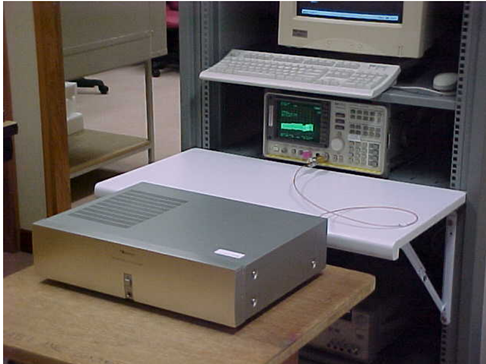
Carrier Frequency Separation Measurement Test Setup – AV Unit
