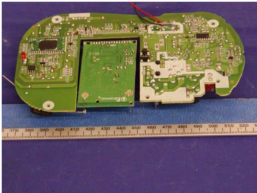
EUT – Main Board Solder View 2
