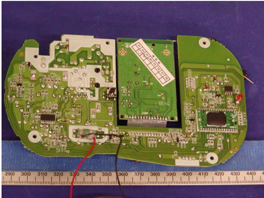
EUT – Main Board Solder View 1
