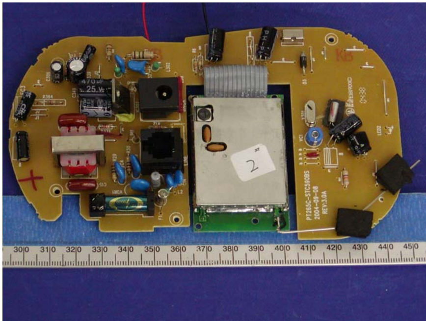
EUT – Main Board Component View 1
