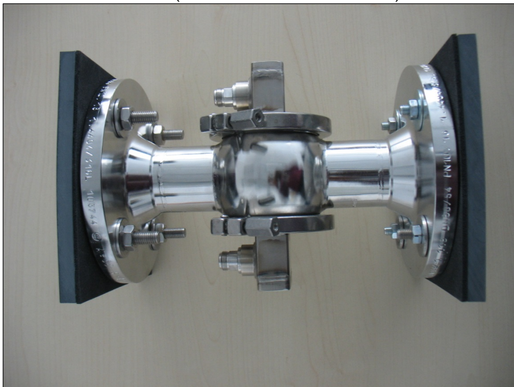
Photo 4: (Flow cell sensor LB 5660-XXX-XXX)
