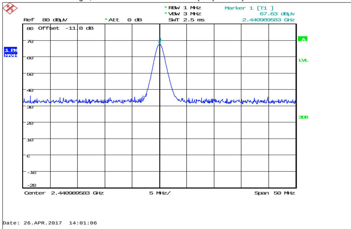
Plot 2: Maximum field strength, MicroPolar Brix ++ LB 565-11 (AC powered) with Flow cell sensor
