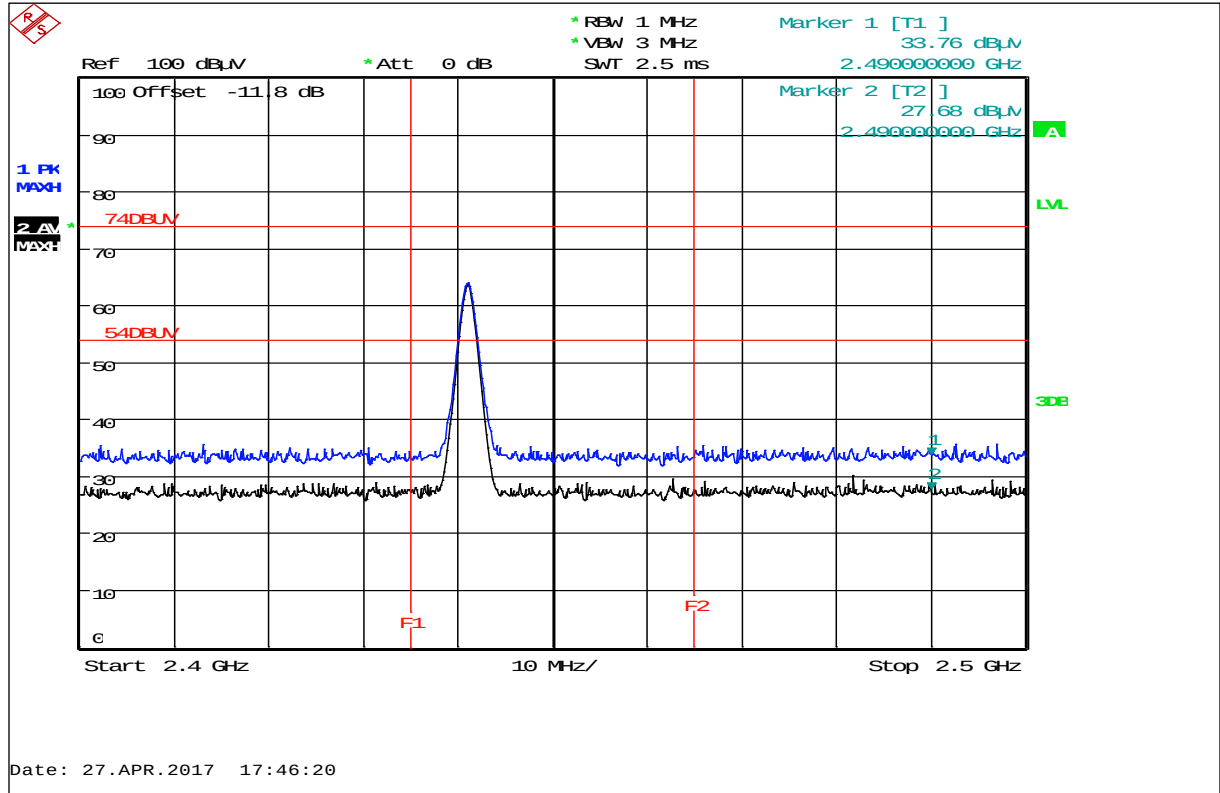
Plot 23: BEC, LB 565-12 (DC powered) with Tank sensor, horizontal / vertical polarization
