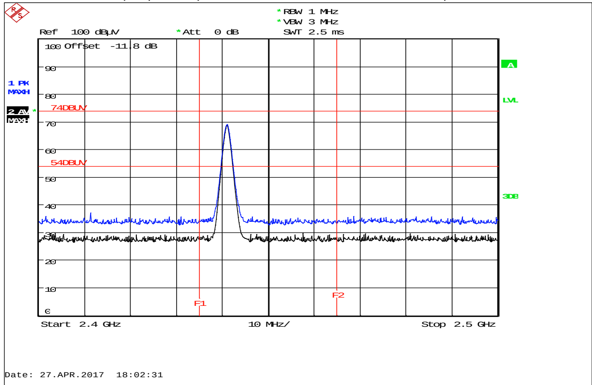
Plot 24: BEC, LB 565-12 (DC powered) with Flow cell sensor, horizontal / vertical polarization
