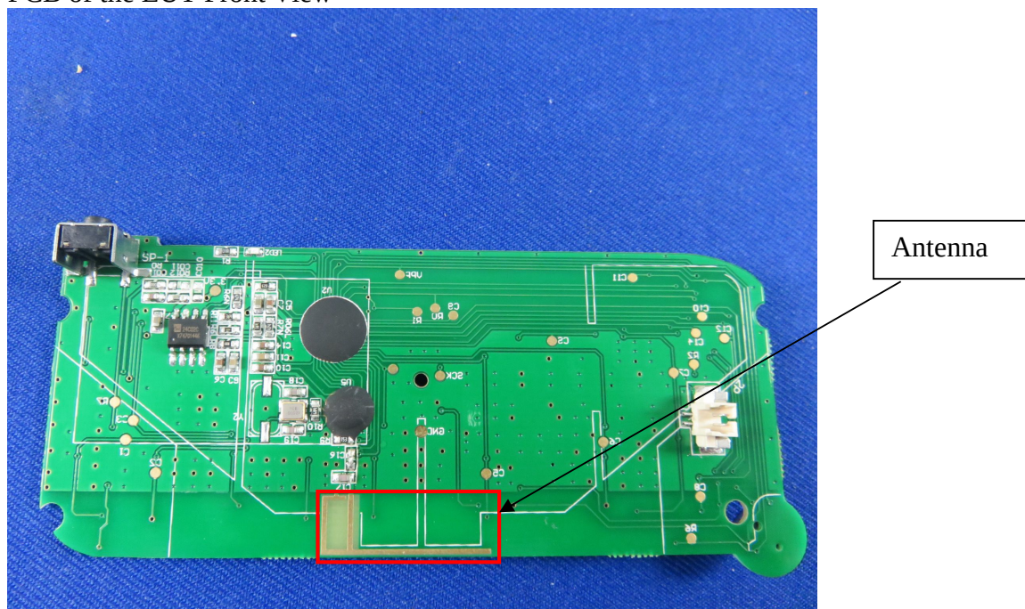
Figure 14 PCB of the EUT-Front View
