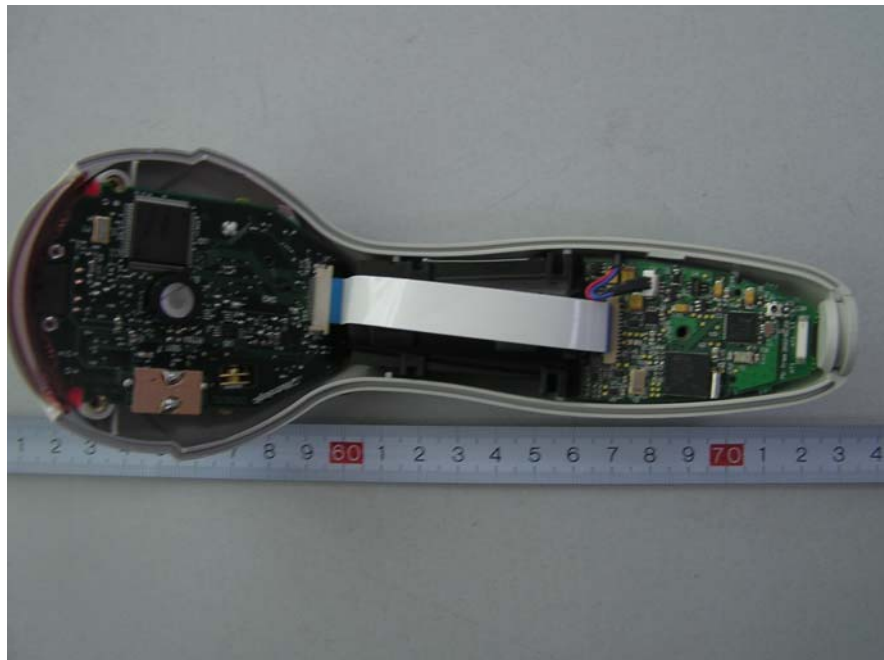
Handset –Inside View (2)
