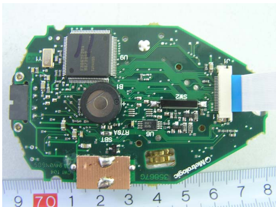
Handset –Digital PCB Bottom View
