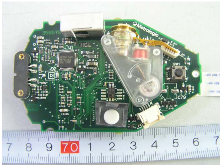
Handset – Digital PCB Top View
