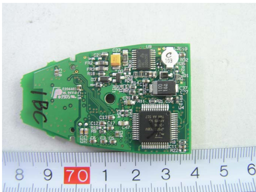
Handset –RF PCB Bottom View
