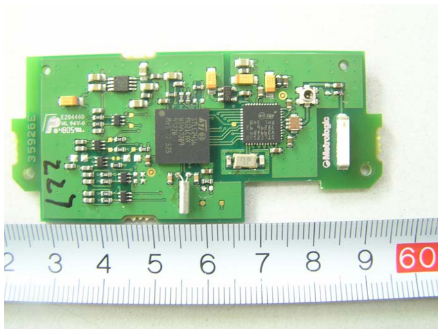
Base – RF PCB Top View
