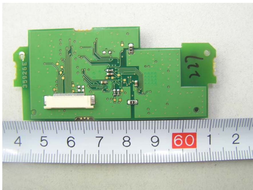
Base –RF PCB Bottom View
