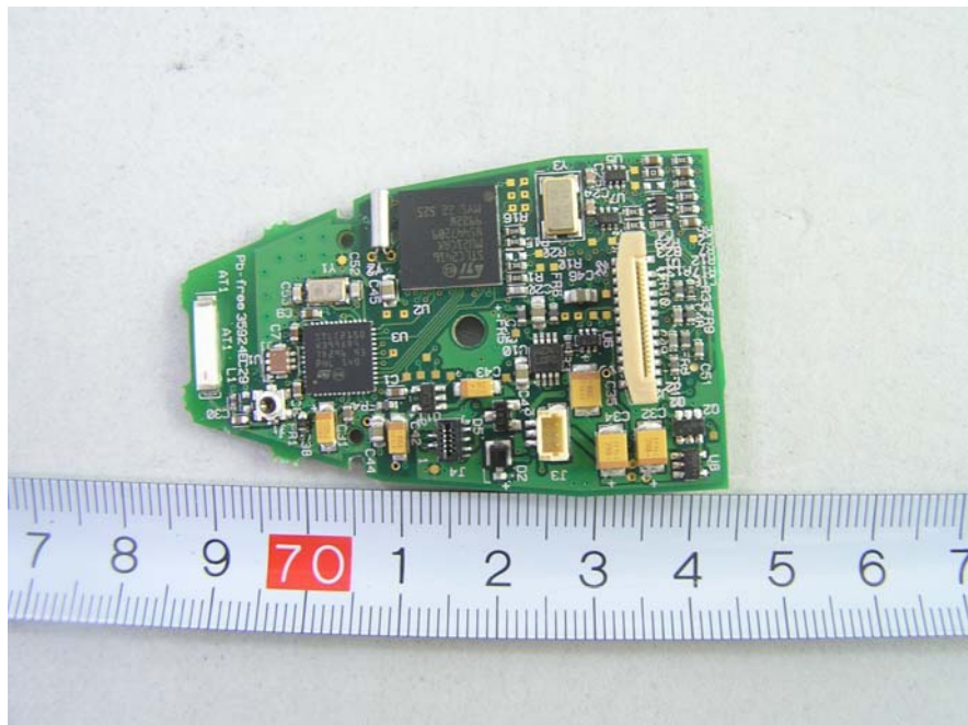
Handset – RF PCB Top View
