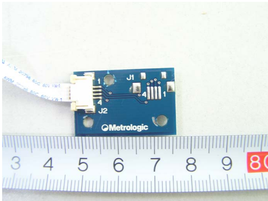
Handset – LED PCB Top View
