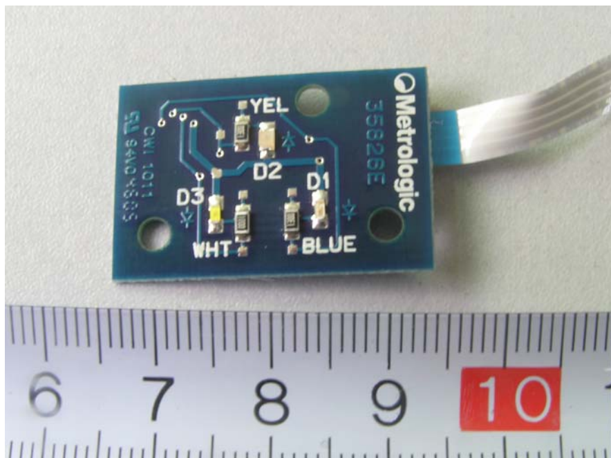
Handset –LED PCB Bottom View
