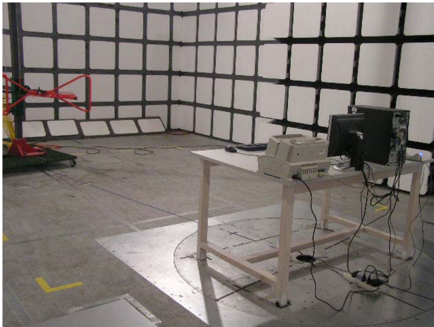
MI9535 Transmitting: Radiated Emission - Rear View (30 MHz-1 GHz)
