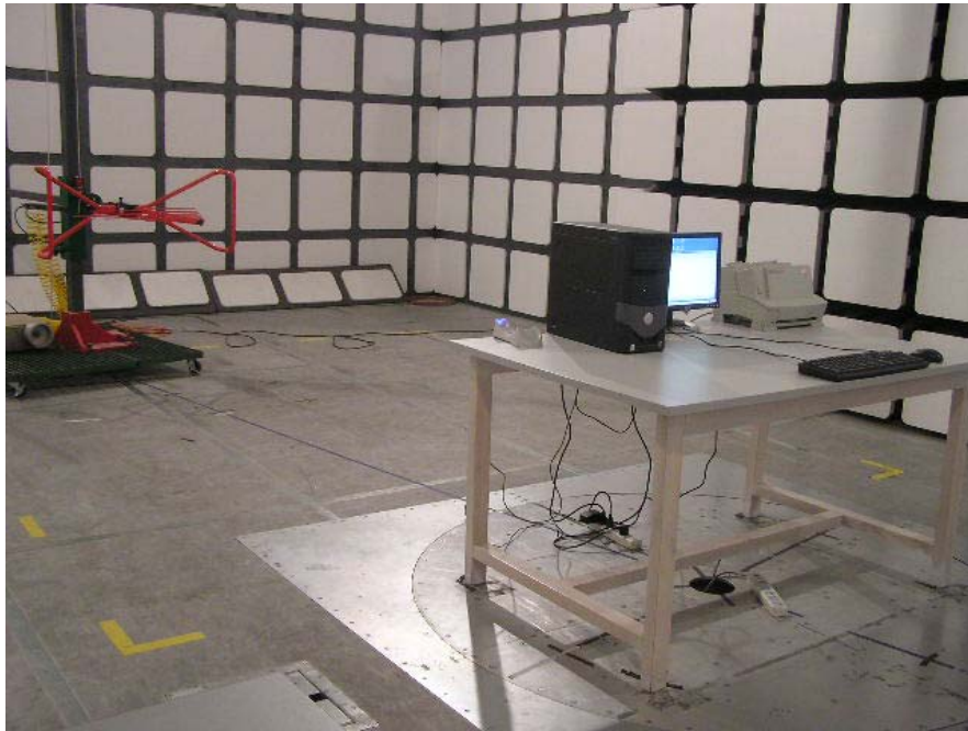
MI9535 Transmitting: Radiated Emission - Front View (30 MHz-1 GHz)
