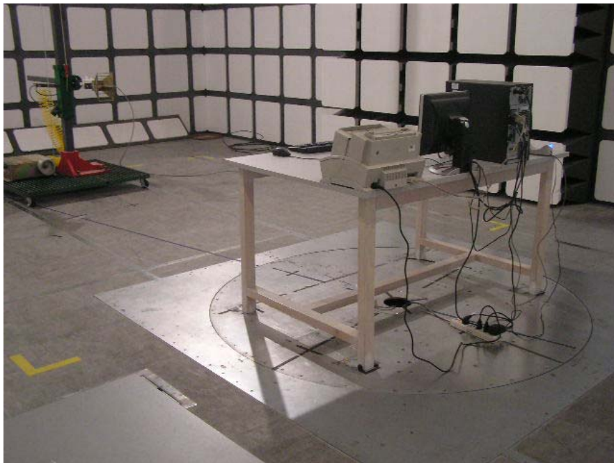
MI9535 Transmitting: Radiated Emission - Rear View (Above 1 GHz)
