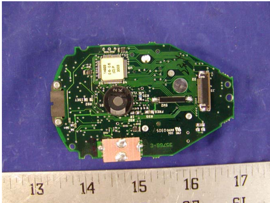
EUT – Scanner Laser Board Solder View
