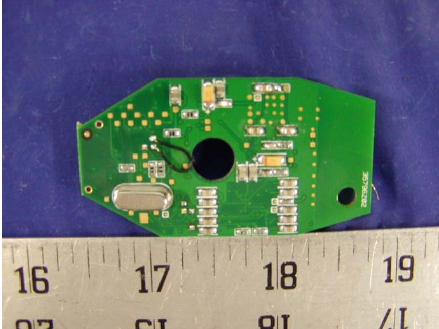
EUT – Scanner / Transmitter Main Board Solder View
