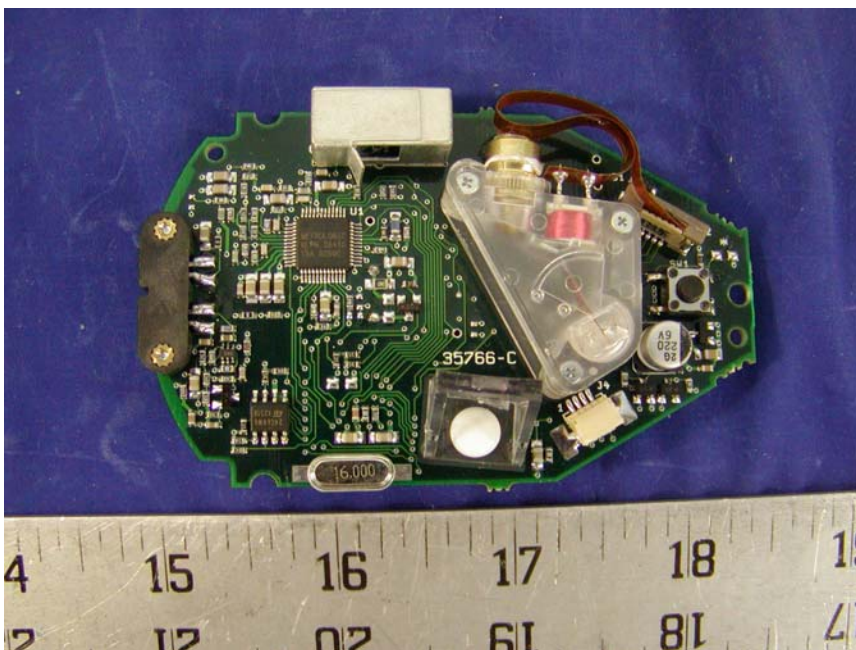
EUT – Scanner Laser Board Component View
