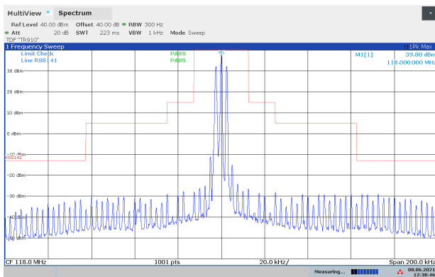
Emission Mask 2500Hz, 85% Mod, 118.000 MHz, Ch25kHz
