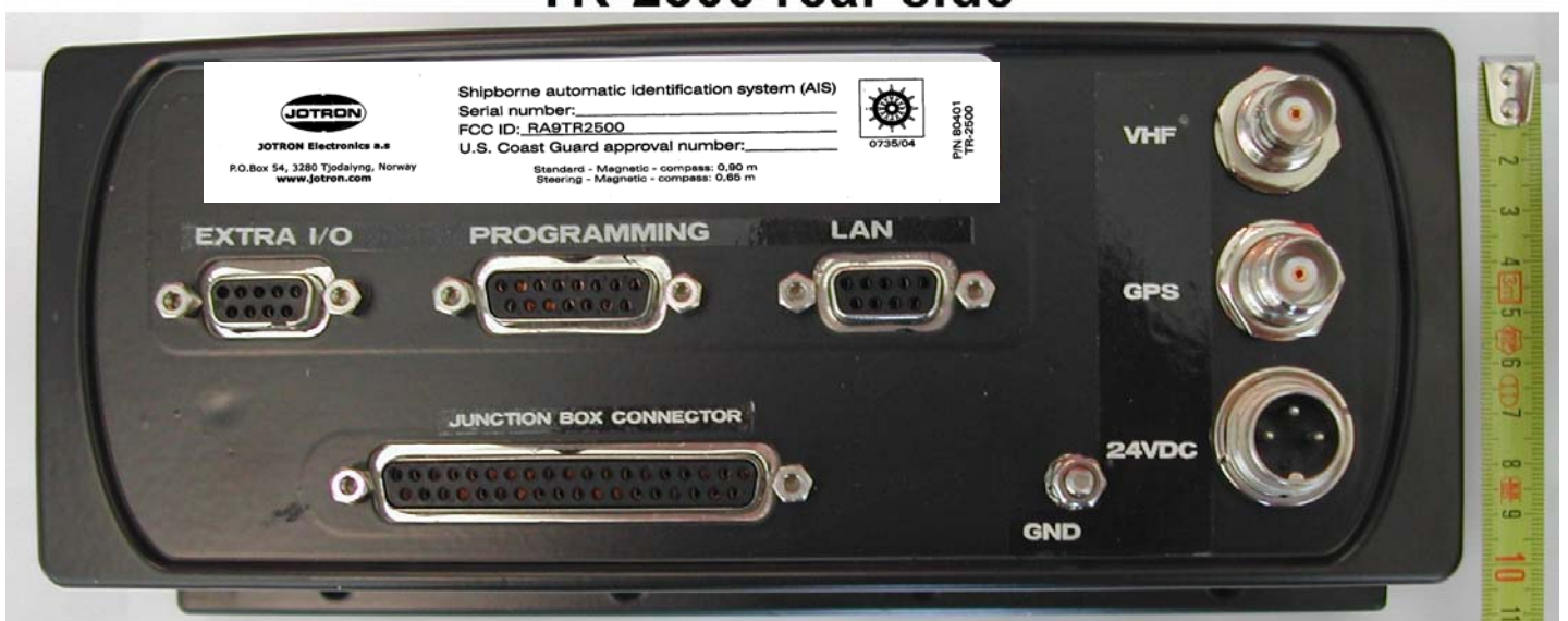
TR-2500 rear side
