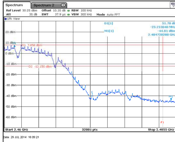
Figure 7.5.1.2-29: Upper Band-edge - 802.11b
