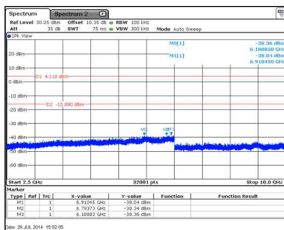
Figure 7.5.1.2-14: 802.11g – 2437MHz – 2.5GHz – 10GHz
