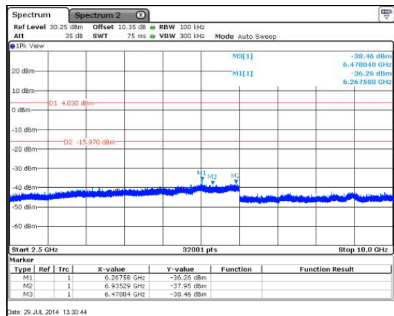
Figure 7.5.1.2-20: 802.11n – 2412MHz – 2.5GHz – 10GHz
