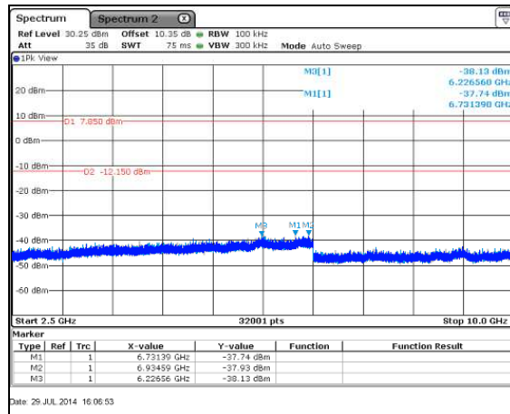
Figure 7.5.1.2-8: 802.11b - 2462MHz - 2.5GHz - 10GHz
