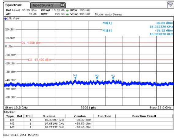
Figure 7.5.1.2-18: 802.11g – 2462MHz – 10GHz – 25GHz
