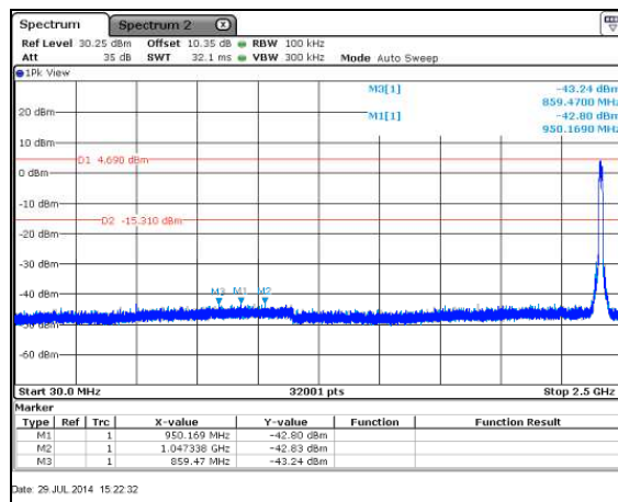
Figure 7.5.1.2-10: 802.11g - 2412MHz - 30MHz - 2.5GHz
