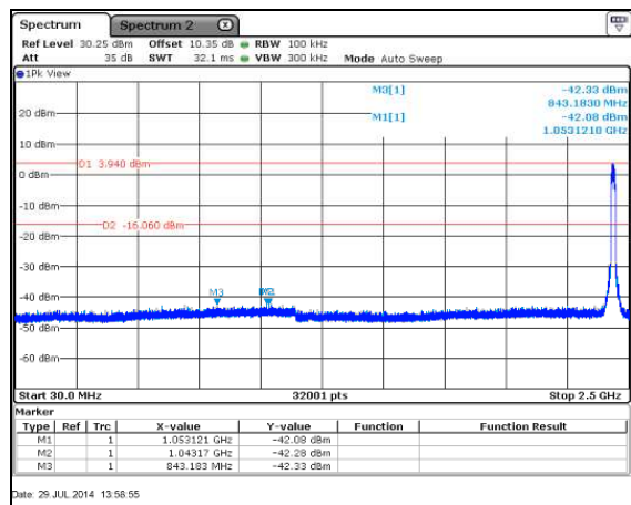
Figure 7.5.1.2-22: 802.11n – 2437MHz – 30MHz – 2.5GHz
