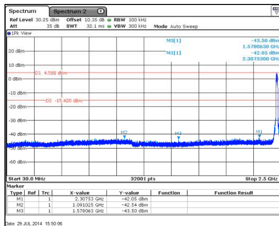
Figure 7.5.1.2-16: 802.11g – 2462MHz – 30MHz – 2.5GHz
