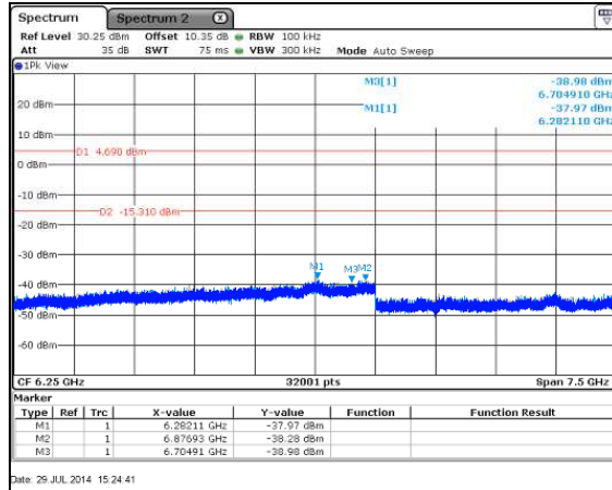
Figure 7.5.1.2-11: 802.11g – 2412MHz – 2.5GHz – 10GHz
