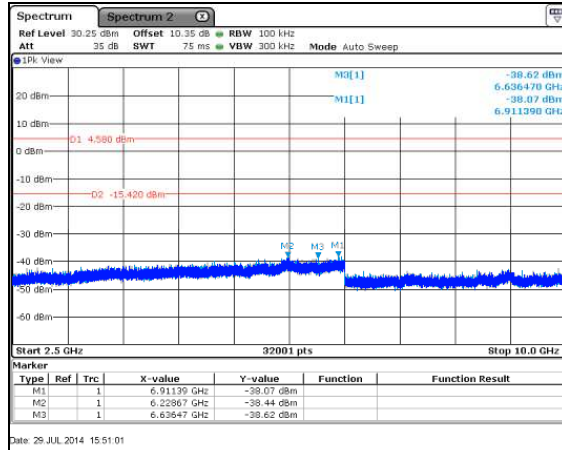
Figure 7.5.1.2-17: 802.11g – 2462MHz – 2.5GHz – 10GHz
