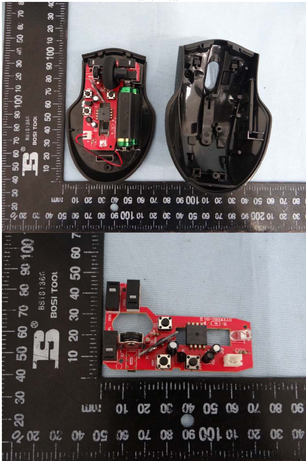
Internal Photo
