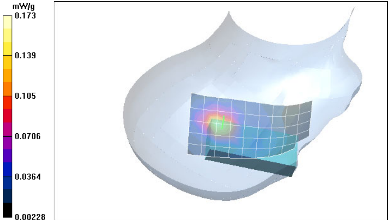
Fig. 4: SAR distribution for PCS 1900, channel 661, tilted position, right side of head. (25.06.2003; Ambient Temperature: 21.8° C; Liquid Temperature : 19.9° C).
