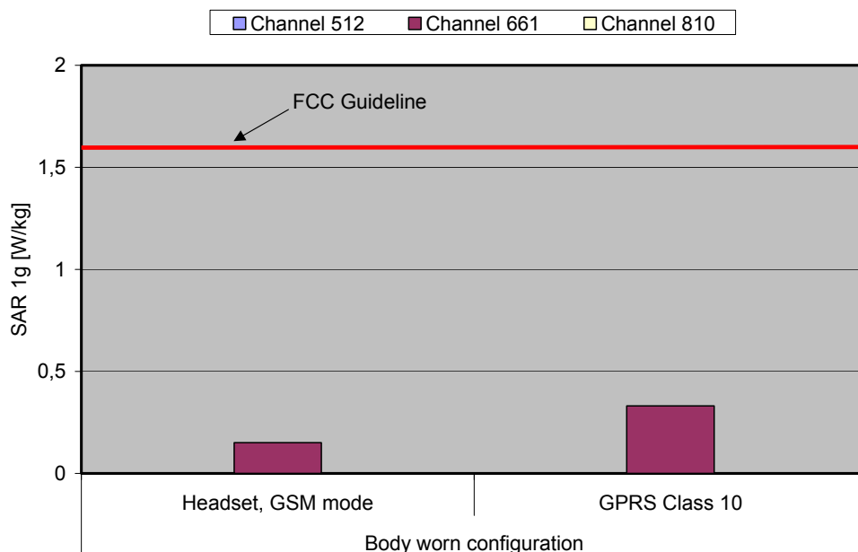
Fig. 9: The measured SAR values in body-worn configuration for the Alcatel OT-S853 for PCS 1900 in comparison to the FCC exposure limit.
