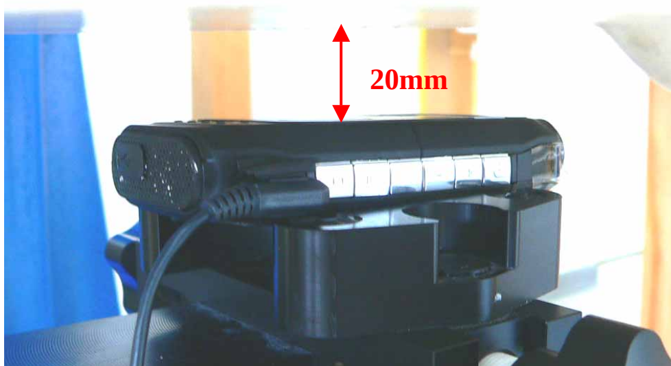
Fig. 20: Body worn configuration, GSM with headset, antenna towards the phantom.
