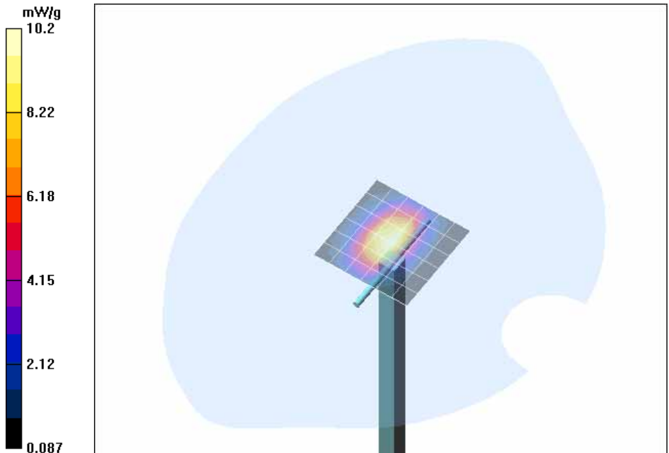
Fig. 10: Validation measurement 1900 MHz Head (August 15, 2005), coarse grid. Ambient Temperature: 22.0° C, Liquid Temperature: 21.0° C.
