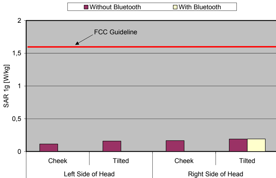
Fig. 8: The measured head phantom SAR values for the Alcatel OT-S853 for PCS 1900 in comparison to the FCC exposure limit.
