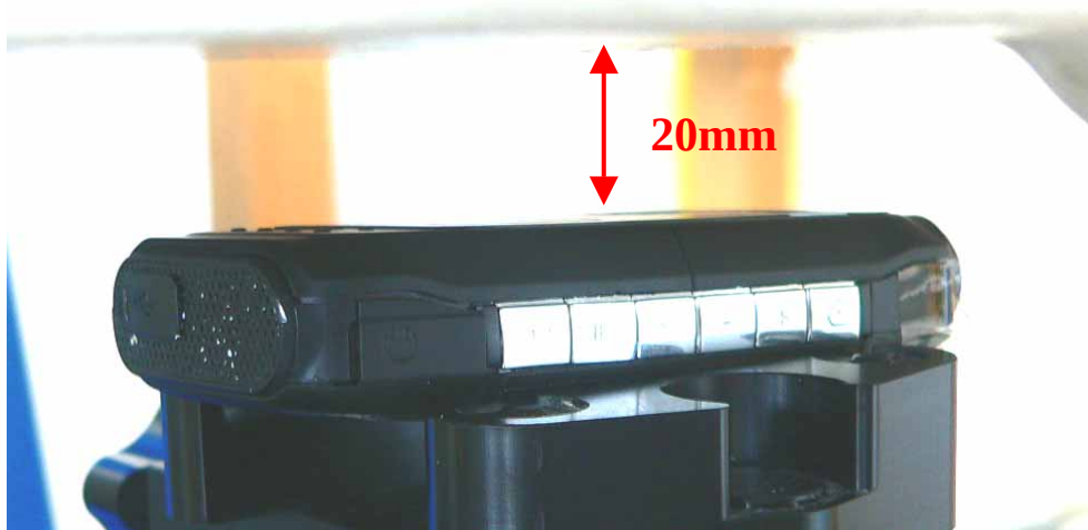
Fig. 21: Body worn configuration, GPRS (Class 10), antenna towards the phantom.
