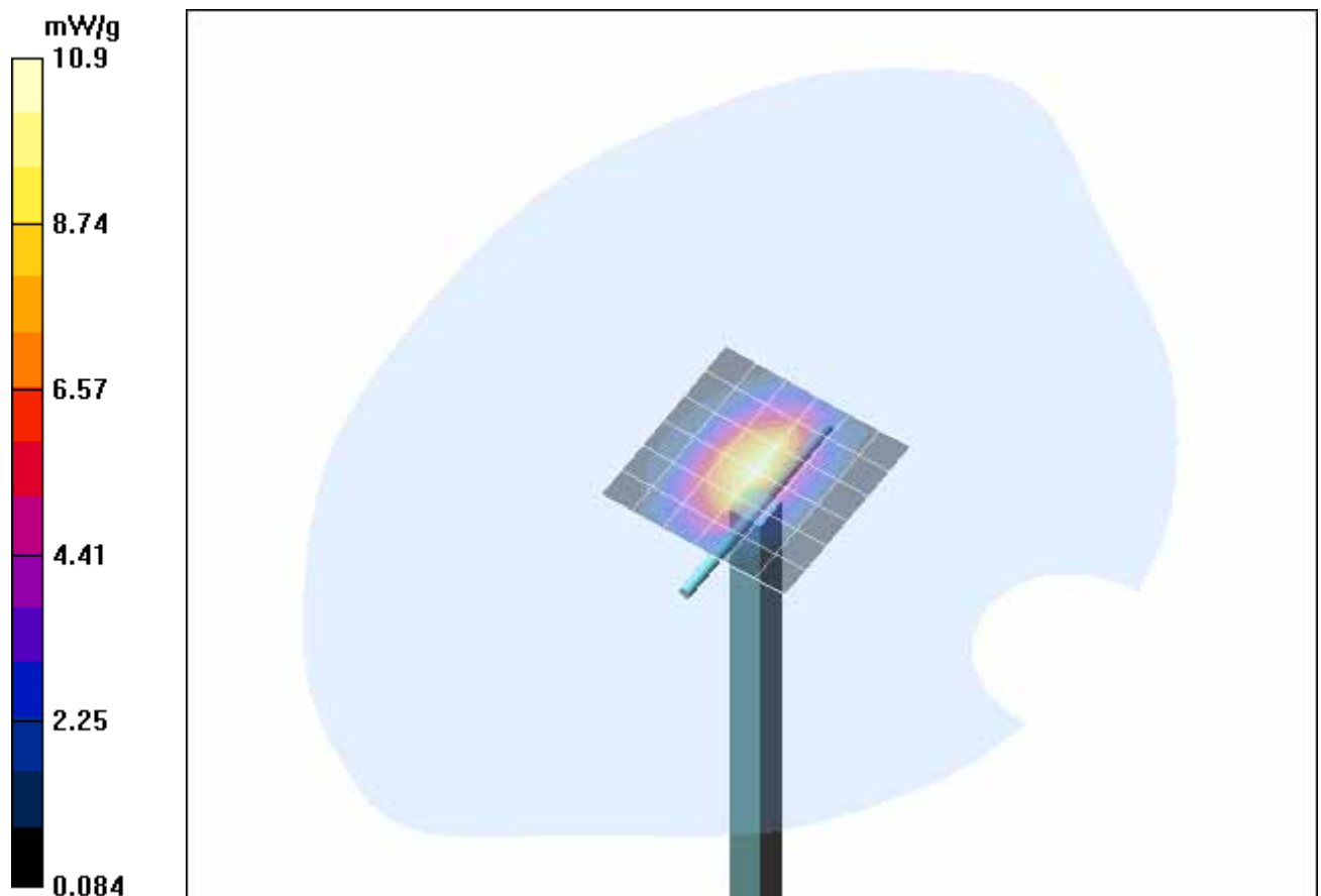
Fig. 11: Validation measurement 1900 MHz body (August 16, 2005), coarse grid. Ambient Temperature: 22.0° C, Liquid Temperature: 21.0° C.
