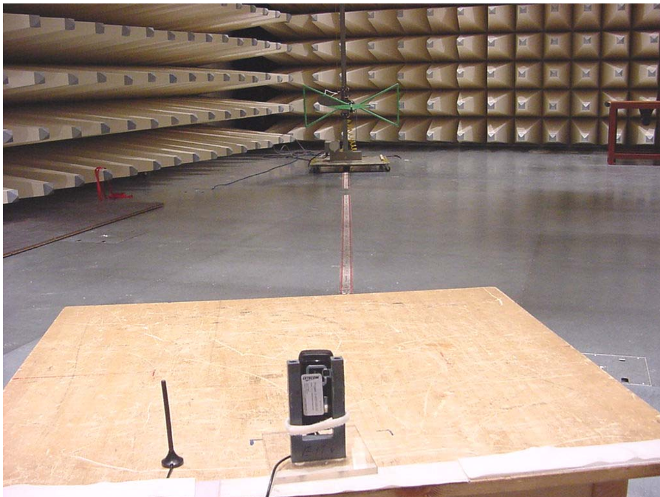
Photo 3 (Radiated Emissions):
