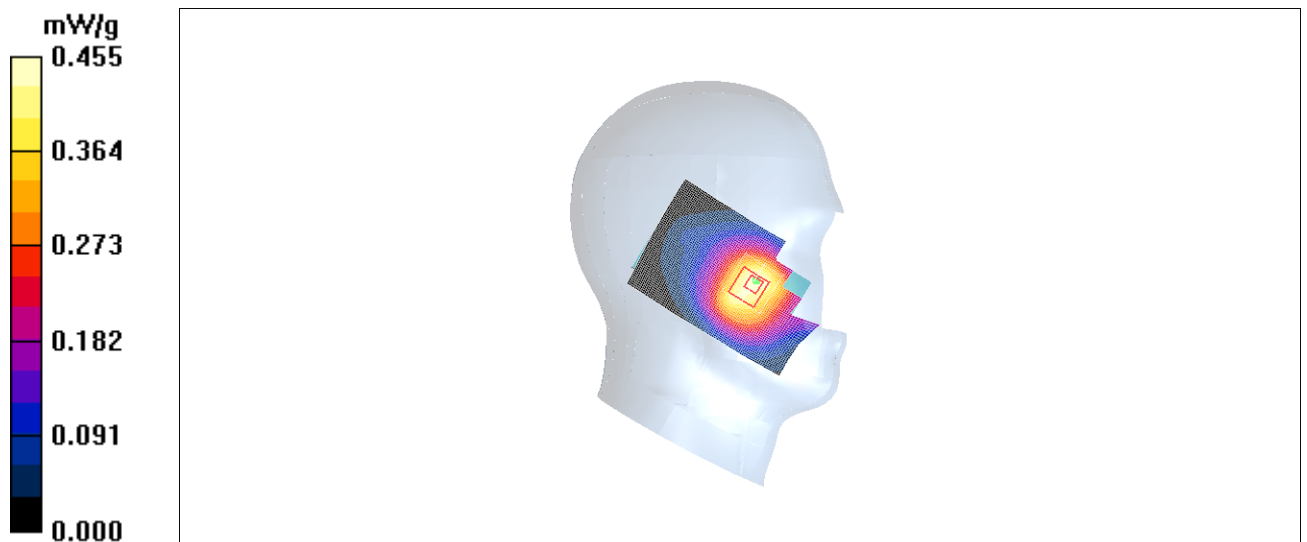
Fig. 3 850 MHz CH128
