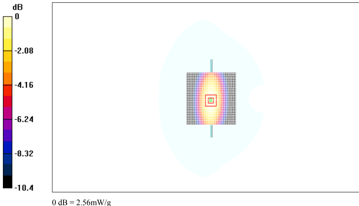
Fig.49 validation 835MHz 250mW
