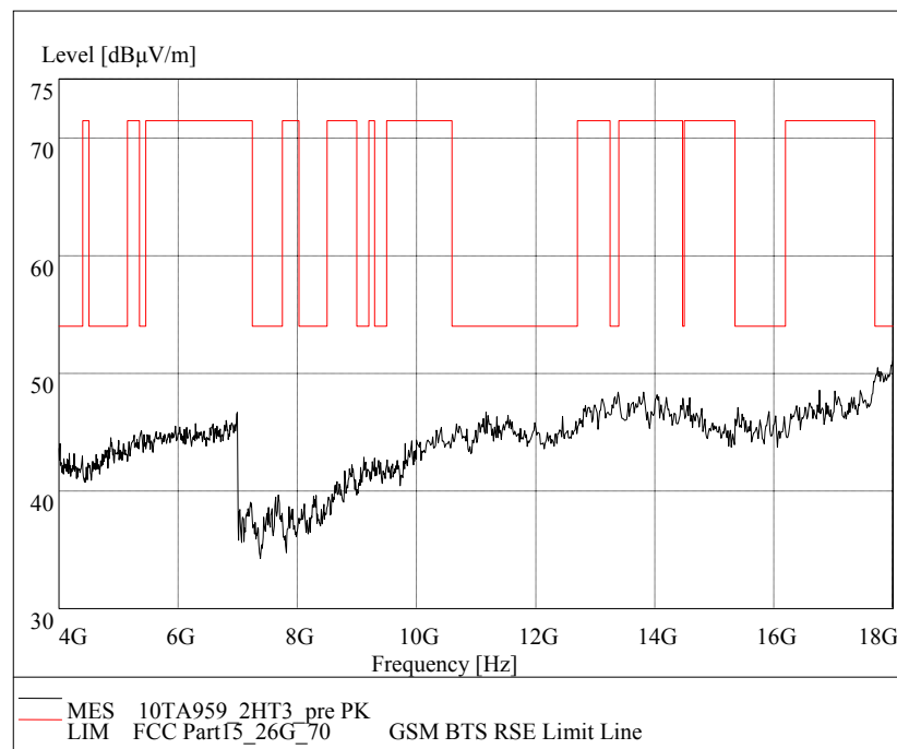
Fig.78. Radiated emission: \pi/4 DQPSK, Channel 78, 4 GHz - 18 GHz
