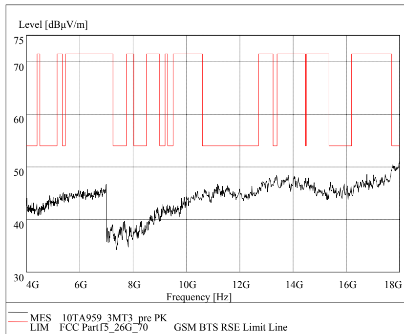
Fig.87. Radiated emission: 8DPSK, Channel 39, 4 GHz - 18 GHz
