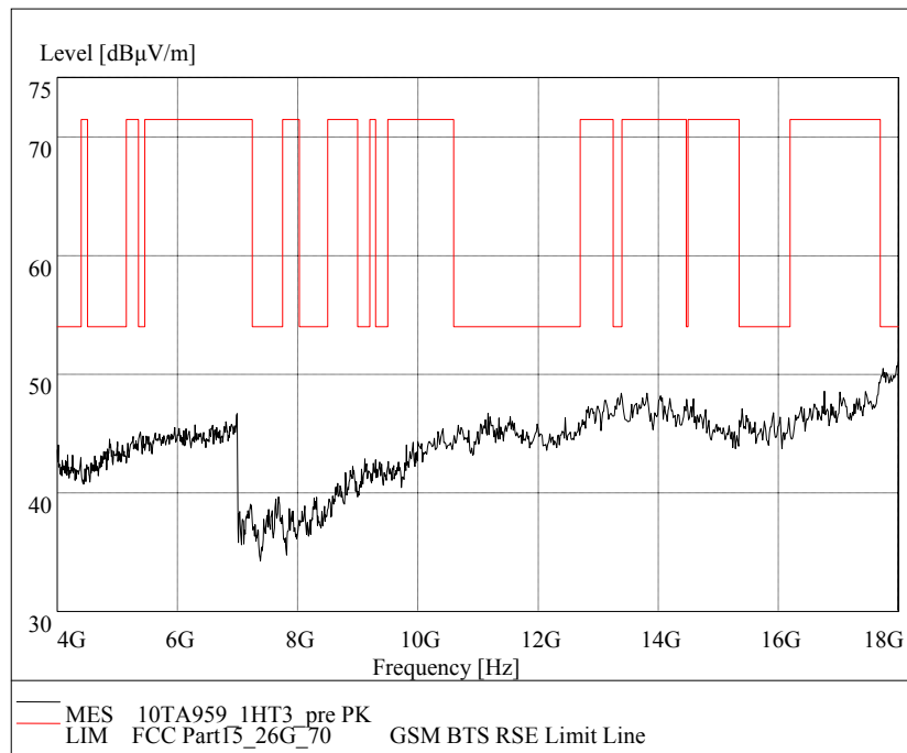
Fig.66. Radiated emission: GFSK, Channel 78, 4 GHz - 18 GHz
