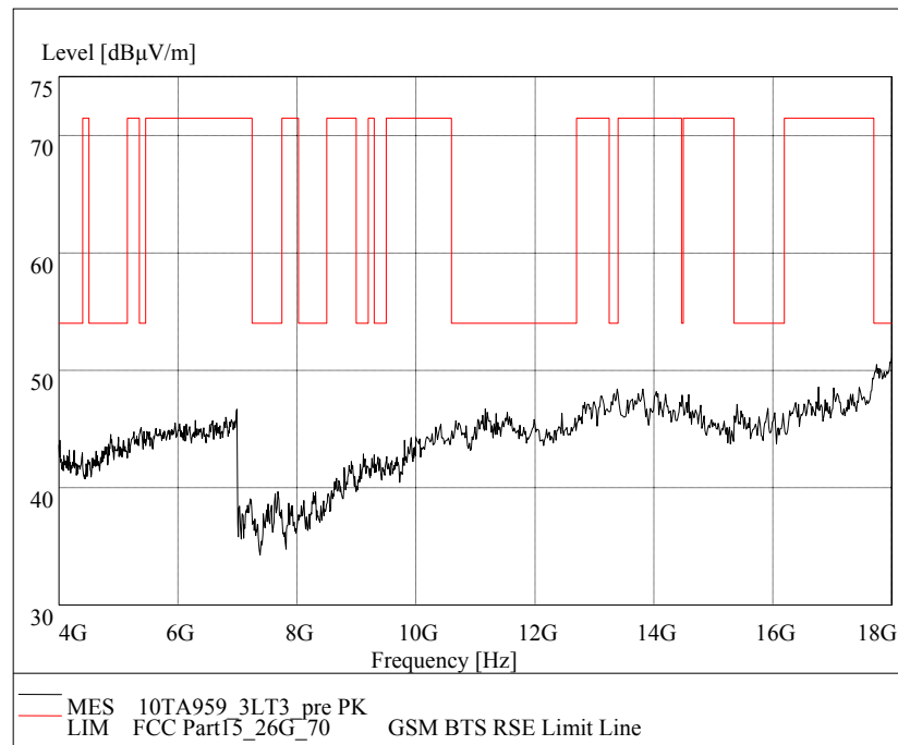
Fig.84. Radiated emission: 8DPSK, Channel 0, 4 GHz - 18 GHz
