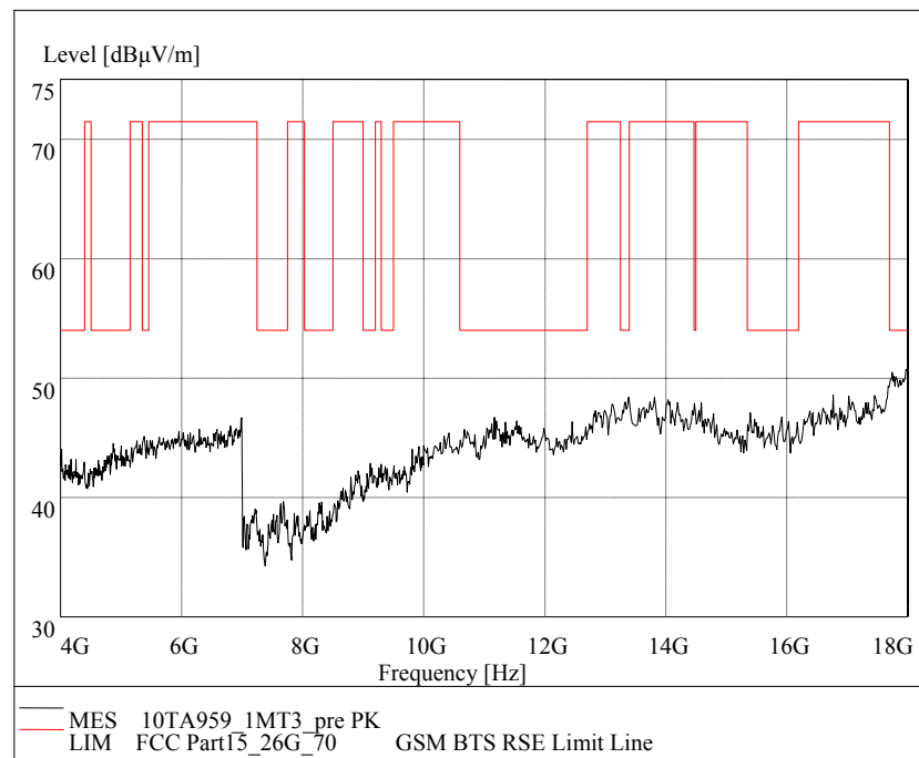
Fig.63. Radiated emission: GFSK, Channel 39, 4 GHz - 18 GHz
