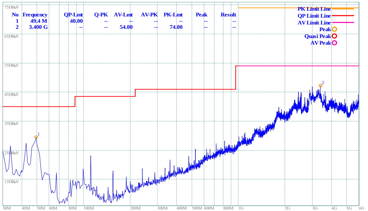
(Plot C: 30M – 6G, Test Antenna Horizontal)
