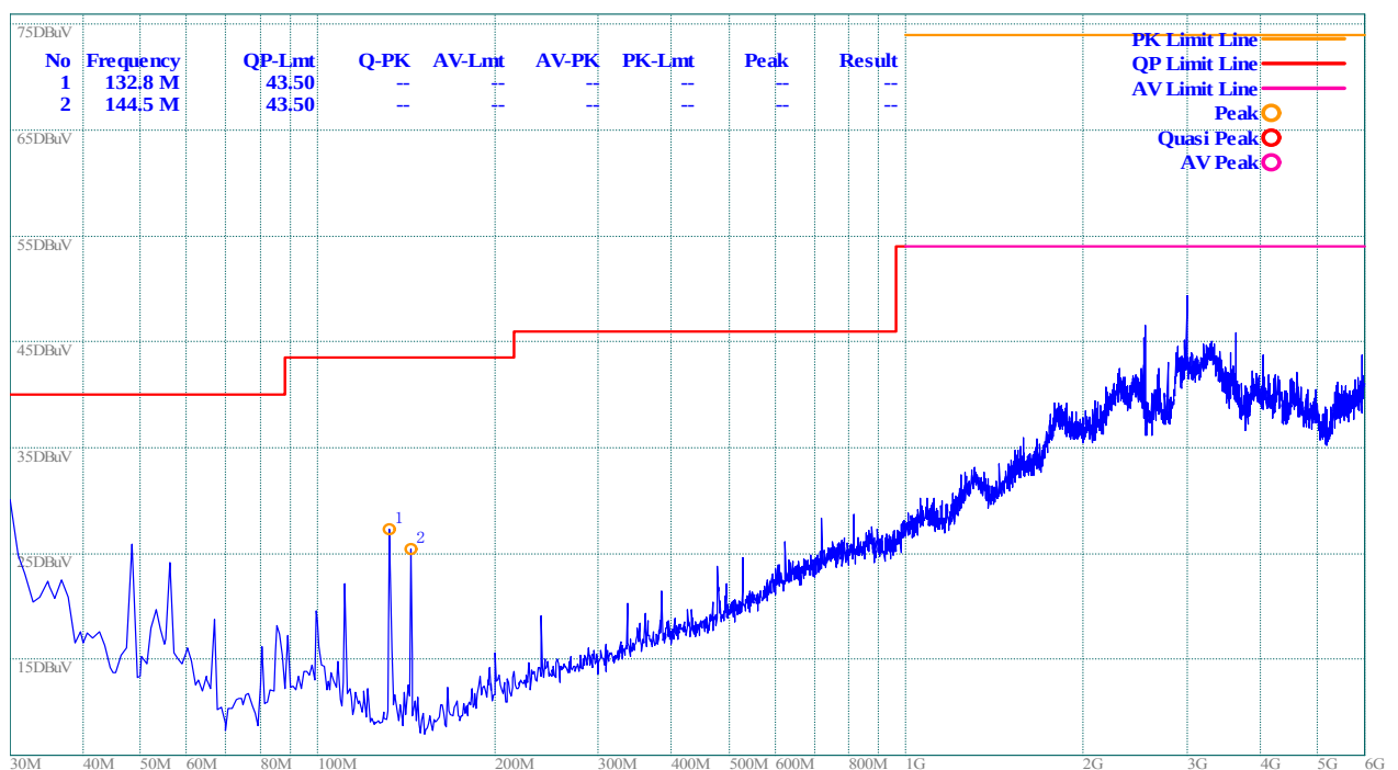
(Plot B: 30M – 6G, Test Antenna Vertical)
