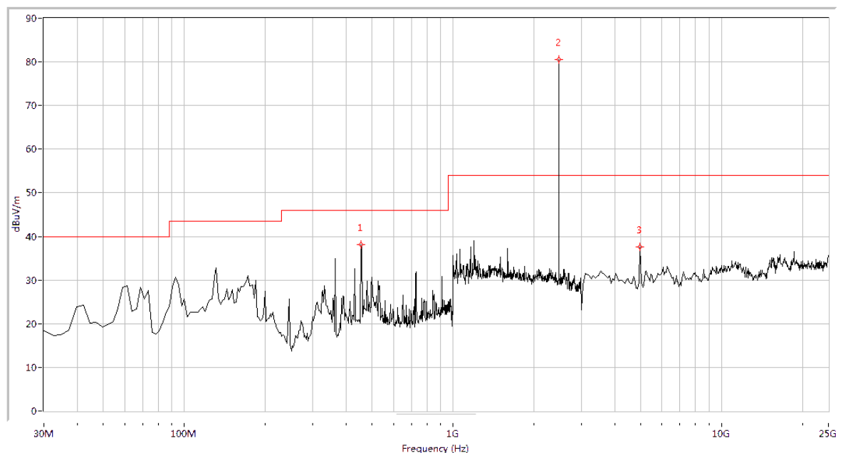
(Plot C.1: 30MHz to 25GHz, Antenna Horizontal @ 1/4-DQPSK, channel 78)
