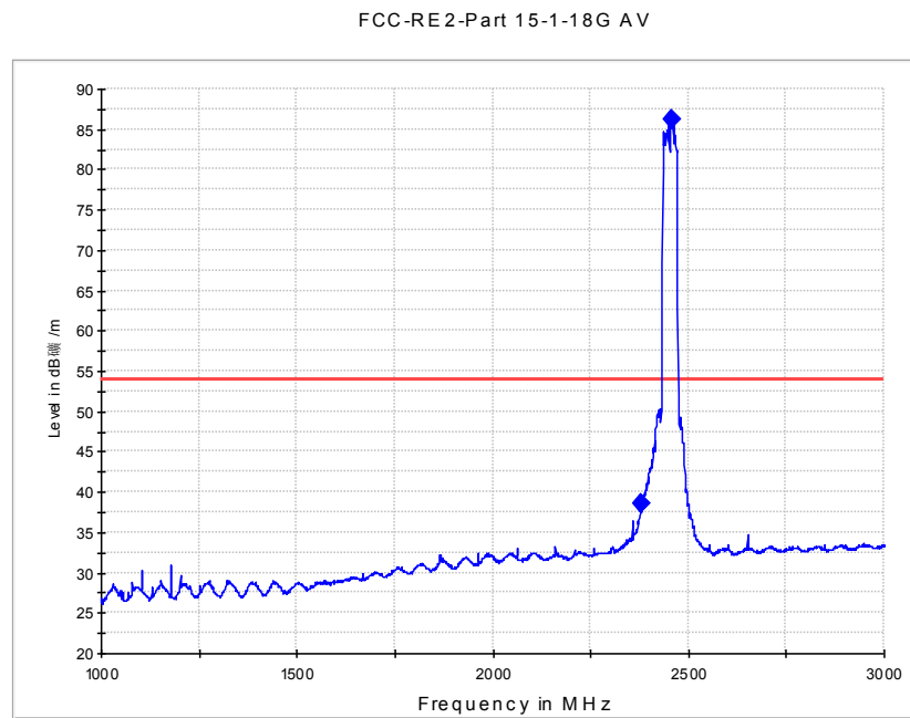
Fig.A.6.2.43 Radiated Spurious Emission (802.11n-HT40, ch9, 1 GHz-3 GHz)
