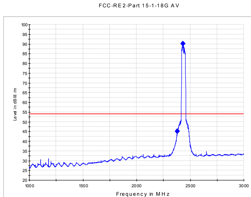
Fig.A.6.2.39 Radiated Spurious Emission (802.11n-HT40, Ch6, 1 GHz-3 GHz)
