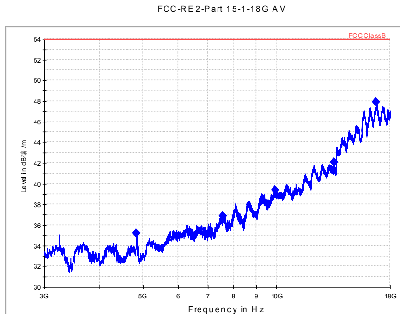
Fig.A.6.2.37 Radiated Spurious Emission (802.11n-HT40, ch3, 3 GHz-18 GHz)
