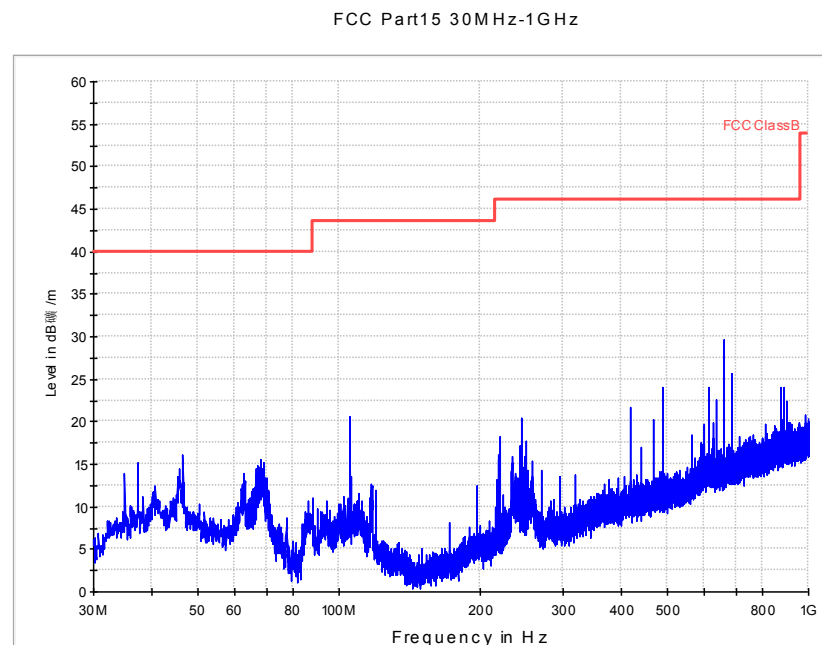
Fig.A.6.2.38 Radiated Spurious Emission (802.11n-HT40, Ch6, 30 MHz-1 GHz)
