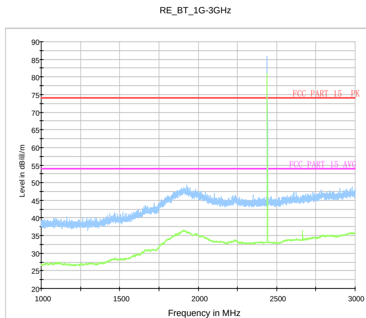
Fig.21. Radiated emission: GFSK, 2440MHz, 1 GHz - 3 GHz
