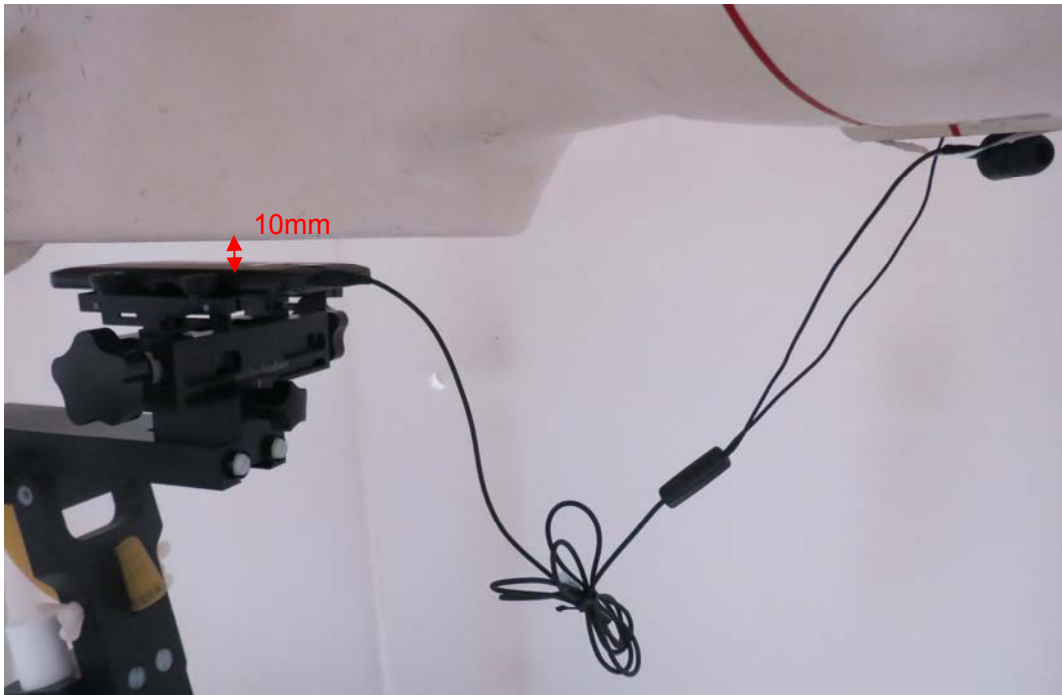
Picture 21: Back Side with Earphone, the distance from handset to the bottom of the Phantom is 10mm
