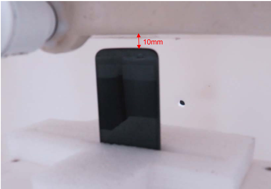
Picture 20: Bottom Edge, the distance from handset to the bottom of the Phantom is 10mm
