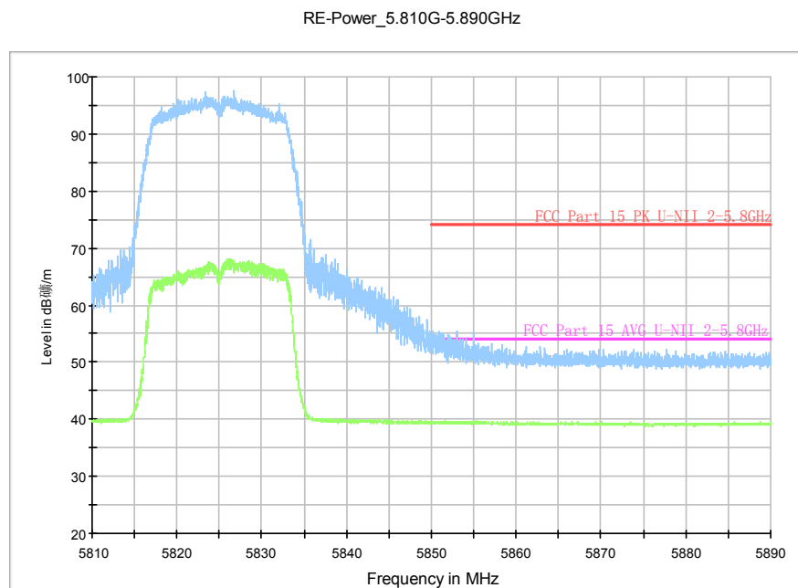
Fig. 73 Band Edges (802.11a, 5825MHz)
