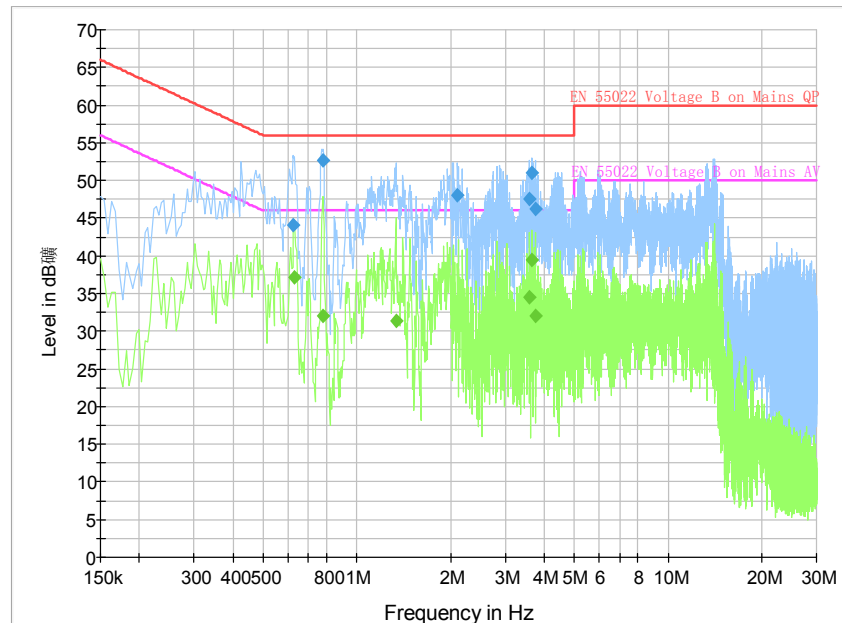
Fig. 79 AC Powerline Conducted Emission-Idle
