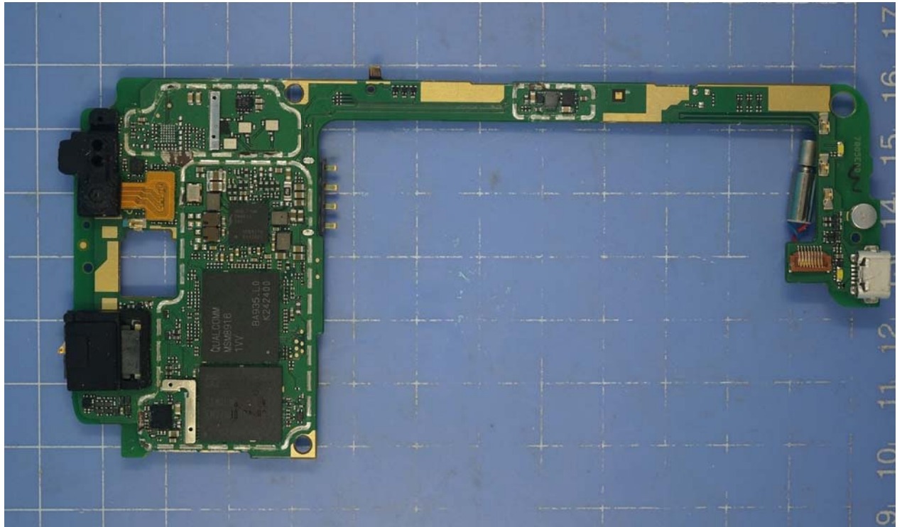
Mobile Phone Disassembly
