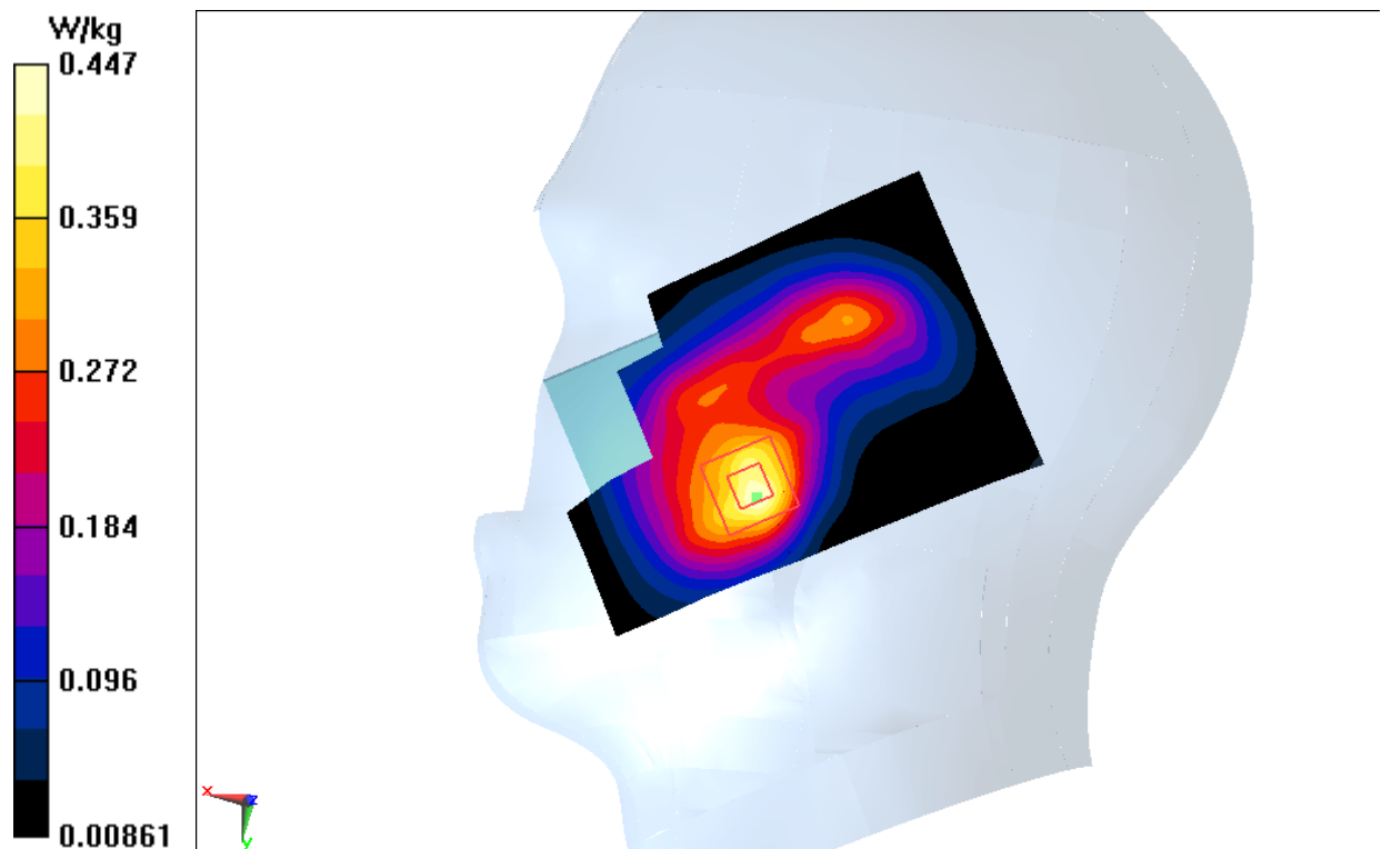
Fig.3 1900 MHz
