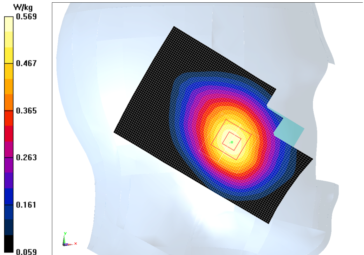
Fig.1 850MHz
